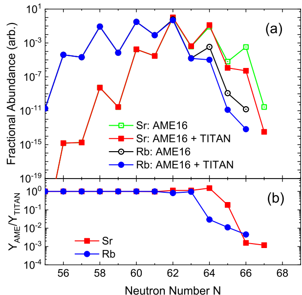
Figure 6. (Color online) (a) Fractional r-process abundance for Rb and Sr isotopes relative to most abundant isotopes using waiting point approximation. Open circles are values taken from AME2016. Filled circles denote a combination of values calculated from AME2016 values and new TITAN mass values from this work. (b) The ratio of fractional abundances ( Y_{\text{AME2016}}/Y_{\text{TITAN}} ) corresponding to values plotted in panel (a).
