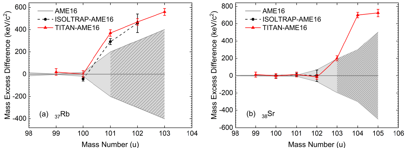
Figure 2. (Color online) Mass excess difference between the value measured in this work and the value reported in AME2016 [16], i.e. ME_{\text{TITAN}} - ME_{\text{AME2016}} for (a) _{37}\text{Rb} and (b) _{38}\text{Sr} isotopes. The shaded band indicates the AME2016 uncertainties and slanted lines in shaded region denotes values from extrapolation. ME difference is also plotted for a previous measurement from ISOLTRAP [30], published after the AME2016.
