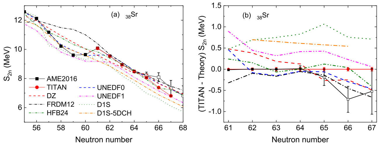
Figure 4. (Color online) (a) S_{2n} values for isotopes of ^{38}\text{Sr} compared with values from different mass models, and (b) the difference between S_{2n} values from this work and different mass models. Circles and squares represent experimental and AME2016 values, respectively, with open squares being extrapolated values.
