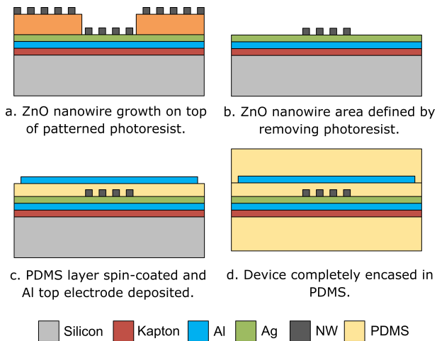
Figure 1. Schematic of device fabrication process.
