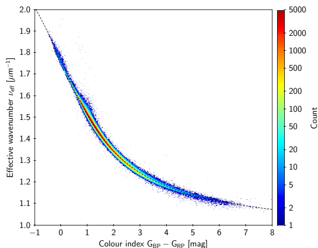
Fig. 2. Relation between the colour index and effective wavenumber for a random sample of 1.5 million sources in EDR3 brighter than G = 18 . The dashed curve is the approximate mean relation in Eq. (3) or (4).
