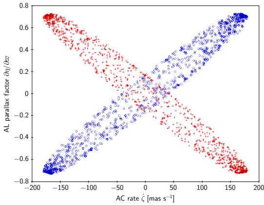
Fig. B.1. Correlation between AC rate and AL parallax factor. Blue circles show a random selection of 1000 FoV transits from data segments DS0–DS5, when the scanning law was in its normal (forward precession) mode. Red crosses show 1000 random transits from data segments DS6 and DS7, when the reversed precession mode was used. EDR3 is exclusively based on observations taken in the forward precession mode.
