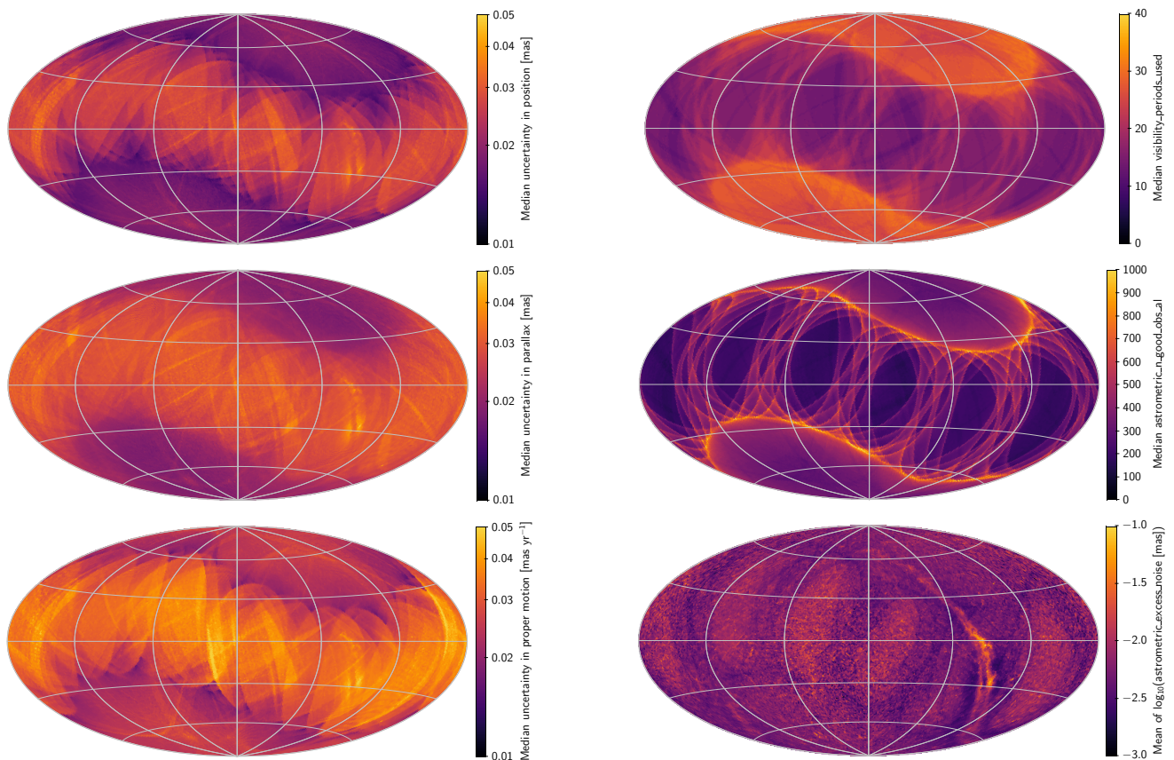
Fig. 9. Selected observation statistics at G \approx 15 for sources with a five-parameter solution in EDR3. These statistics are main factors governing the formal uncertainties of the astrometric data. Top: Number of visibility periods used. Middle: Number of good CCD observations AL. (The number of FoV transits used in the solution looks very similar, only with a factor nine smaller numbers.) Bottom: Mean of \log_{10}[\max(0.001, \text{astrometric\_excess\_noise})] .
