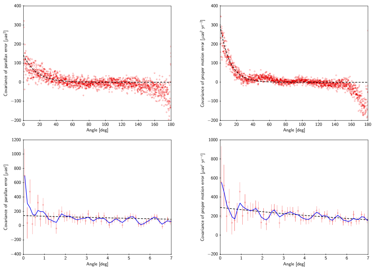
Fig. 15. Angular covariances of the five-parameter quasar sample. Left: Covariance in parallax, V_\pi(\theta) . Right: Covariance in proper motion, V_\mu(\theta) . The red circles are the individual estimates; the dashed black curves are fitted exponential functions. The bottom panels show the same data as in the top panels, but for small separations only, with error bars (68% confidence intervals) and running triangular mean values (blue curves).
