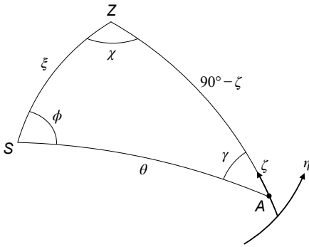
Fig. B.2. Spherical triangle for the parallax factor and AC rate. A is the position of the star, Z the nominal spin axis of Gaia (perpendicular to the two viewing directions), and S the position of the Sun. The directions of the AL and AC field angles \eta , \zeta are indicated.
