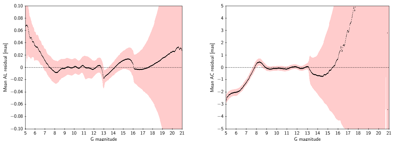
Fig. A.4. Mean residual AL (left) and AC (right) vs. magnitude for the primary sources. A mean residual (AL and AC) is computed for each source. The black curve is the median of these values, and the shaded areas indicates their 16th and 84th percentiles.
