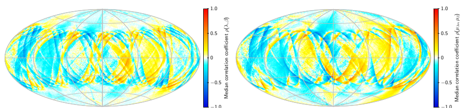
Fig. 11. Median correlation coefficients among the astrometric parameters for six-parameter solutions in Gaia EDR3. The plots were made using all six-parameter sources with G magnitude between 13 and 16. The correlations at other magnitudes are very similar.
