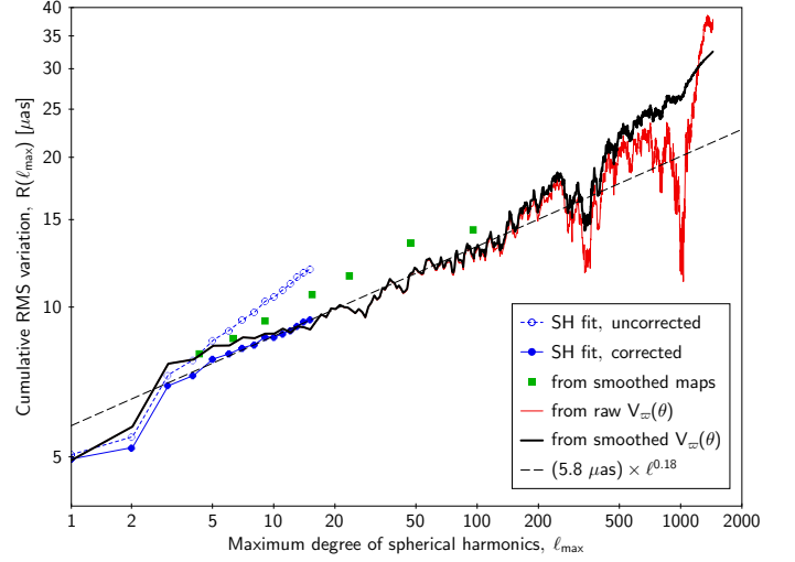
Fig. 16. Cumulative angular power spectrum of systematics in quasar parallaxes.
