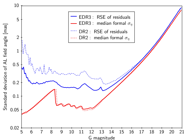
Fig. A.1. Precision of along-scan astrometric measurements as a function of magnitude. Solid curves are for EDR3, dashed for DR2. The red (lower) curves show the median formal precisions from the image parameter determination; the blue (upper) curves are robust estimates 7 of the actual standard deviations of the post-fit residuals.
