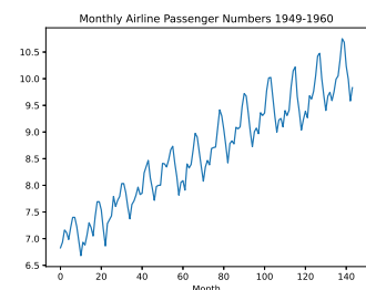
Fig. 71 Airline time series: Box-Cox transformation ( \lambda = 0.148 ).
