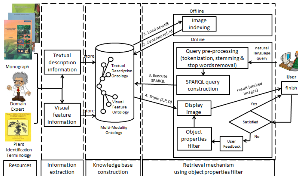
Figure 1. General Framework of Semantic MMO IMR with Object Properties Filter
