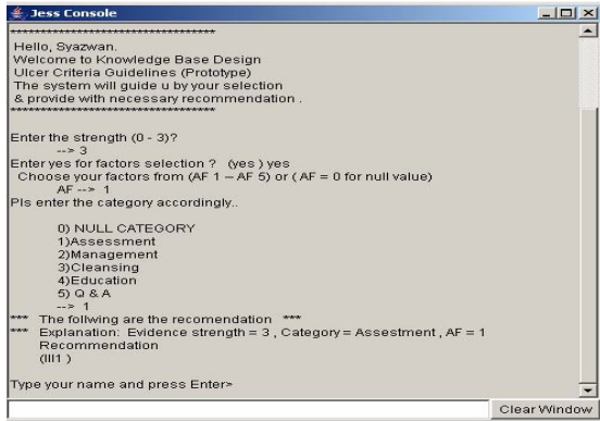
Fig. 4. Sample screenshot of the CPG system
