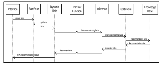
Fig. 3. Sequence Diagram of the CPG system
