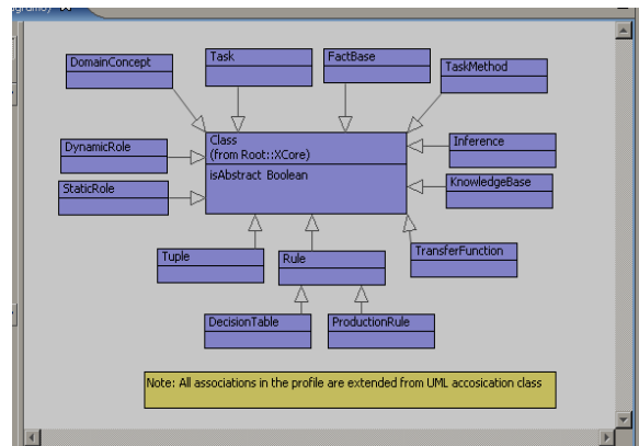
Figure 1. Extension of the UML with stereotypes for the Profile defined in XMF Mosaic tool
