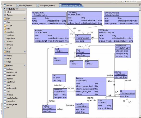
Fig. 2. CPG knowledge model
