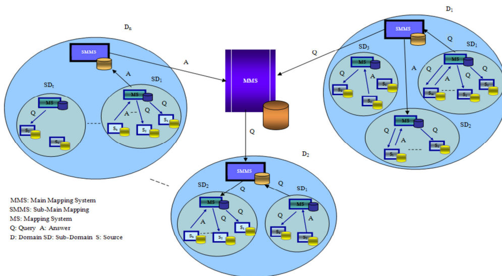
Figure 13. The Architecture of MMSLDI
