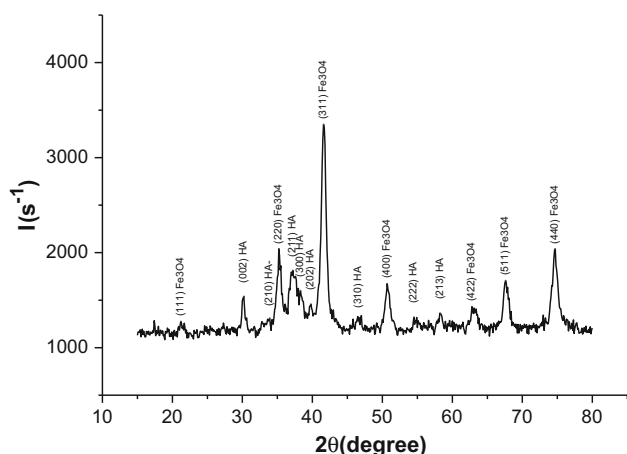
Fig. 3 X-ray diffractogram of Fe 3 O 4 /HA nanocomposite
