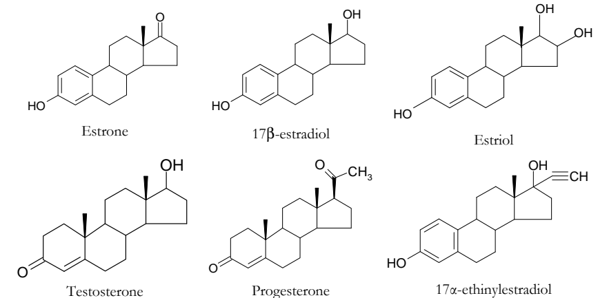
Figure 3: Structures of several steroid hormones.
