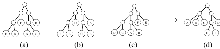
Figure 4.3: An illustration of the consensus hierarchy procedure. From the three sampled dendrograms on the left we identify the clusters encoded in each dendrogram; dendrograms (a),(b) and (c) encode the clusters \{AC, ABC, DE, DEF, ABCDEF\} , \{BC, ABC, EF, DEF, ABCDEF\} , and \{AB, CD, ABCD, EF, ABCDEF\} , respectively. Rejecting those clusters which do not appear in a majority of dendrograms leaves the clusters \{ABC, EF, DEF, ABCDEF\} , which are encoded in the consensus hierarchy (d).
