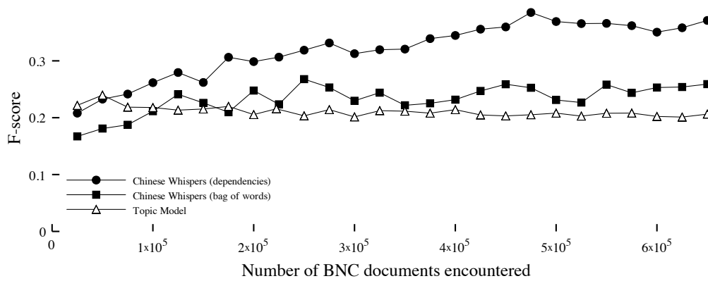
Figure 3.4: Performance of the topic model and Chinese Whispers using dependencies and a bag of words context window.
