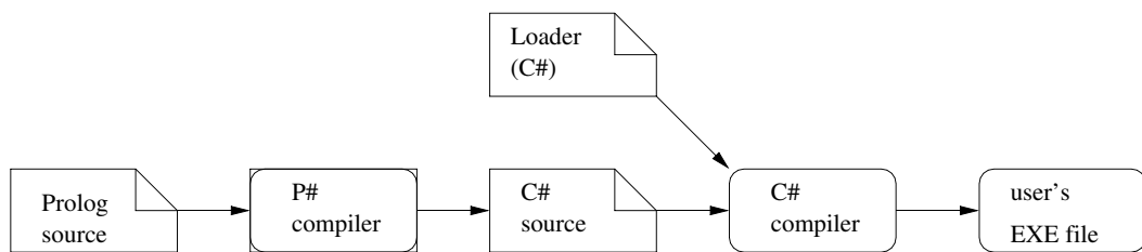
Figure 3.2: Separation into a DLL and an EXE
