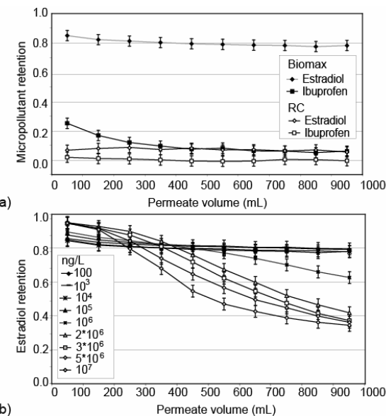
Figure 1 UF of estradiol and ibuprofen: a) Retention by hydrophobic (Biomax) and hydrophilic (RC) membrane, b) Retention of estradiol by hydrophobic (Biomax) membrane for solutions with different estradiol concentrations.
