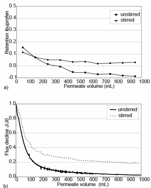
Figure S1 Stirred and unstirred ultrafiltration of alginate 4 mg C/L and ibuprofen a) ibuprofen retention, b) relative flux decline.
