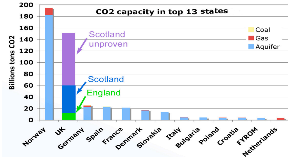
CO2 storage in EU and nearby - the UK is highly ranked. Data from SCCCS study “opportunities for CO2 storage around Scotland” and EU Geocapacity study. Central case values used, assuming 2% efficiency of aquifers.
