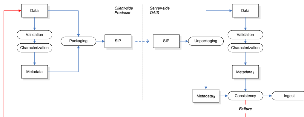
Figure 2. Ingest workflow
