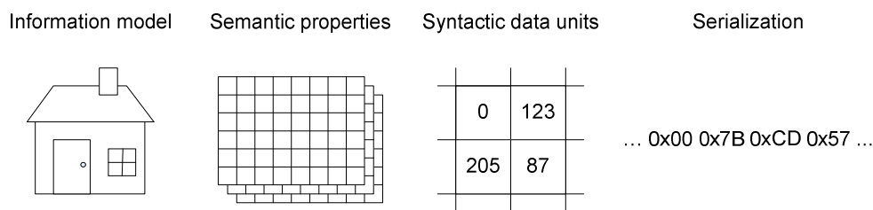
Figure 1. Raster image format in terms of three-stage format transformation
