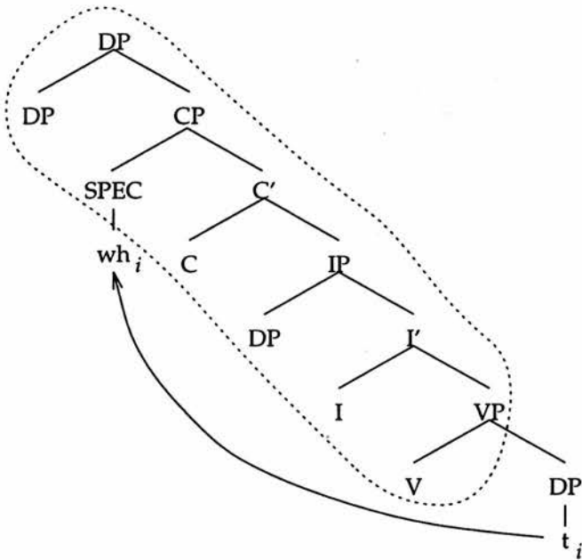
Figure 3.2. Object relative.
