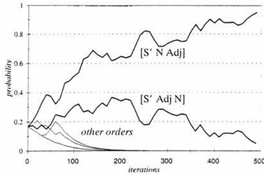
Figure 4. A typical run of the simulation reflecting the parsing preference within a multiple branching noun phrase node NP[N, Adj, {}_S[S Comp]] .
