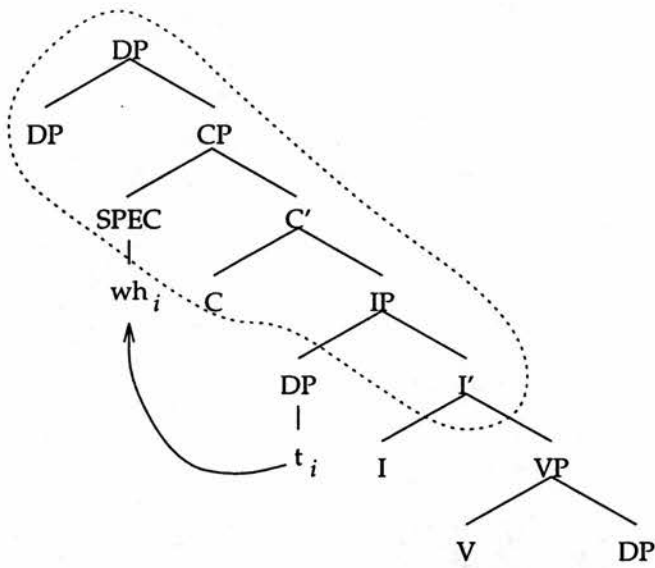
Figure 3.1. Subject relative.
