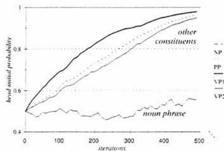
Figure 7. Average of ten runs of the simulation showing the partial fixing of completely free word order to MNCC initial order.
