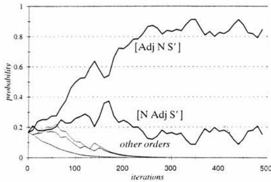
Figure 5. A typical run fixing order within a multiple branching noun phrase node NP[N, Adj, {}_S[Comp S]] .
