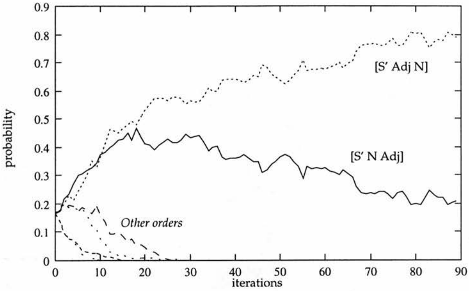
Figure 2.9. A run of the simulation with comp-final relative clause.
