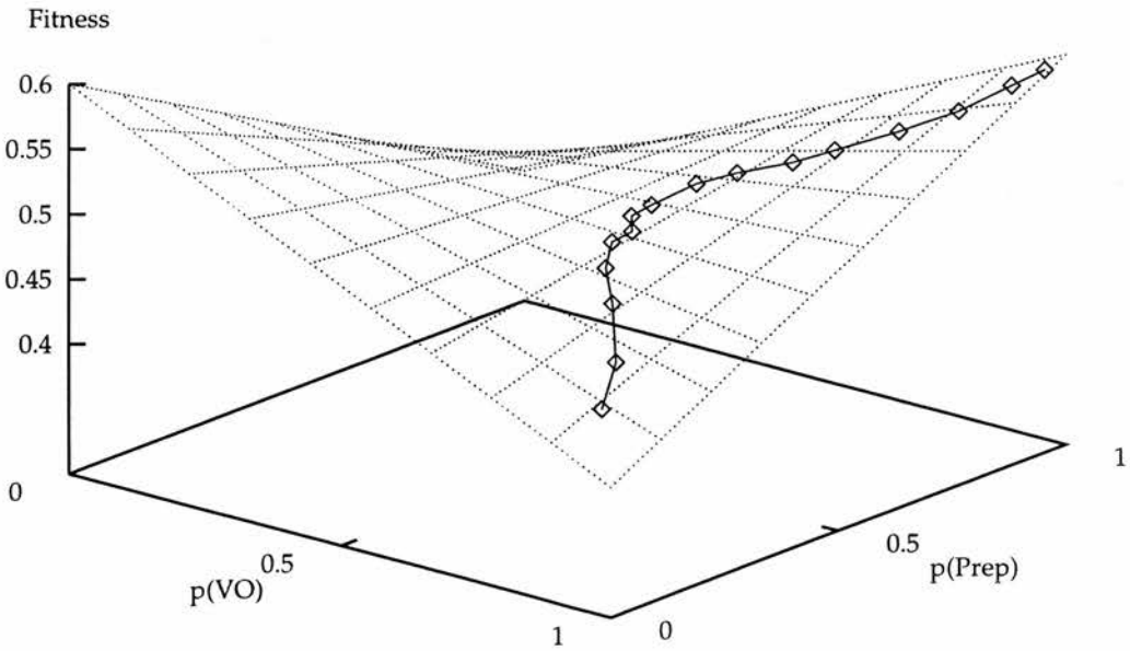
Figure 2.8. The simulation climbing a fitness landscape.
