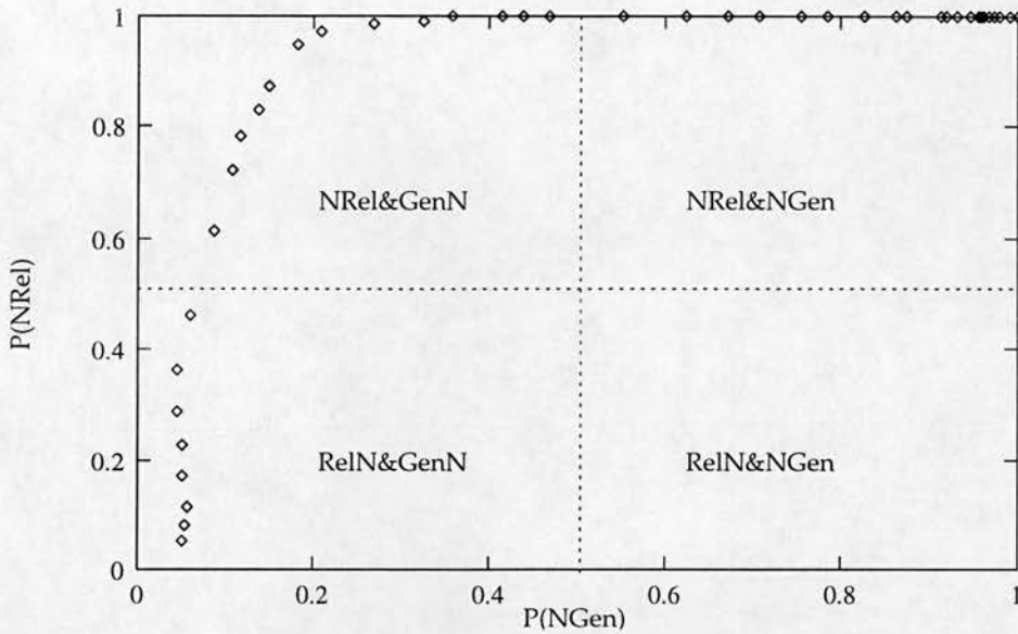
Figure 2.14. Plot of the simulation on NGen/NRel space.
