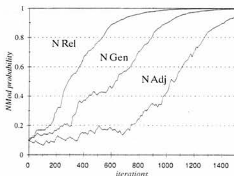
Figure 6. A run of the simulation showing the order of word order rearrangement in line with the prepositional noun-modifier hierarchy.
