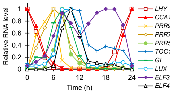
Figure 1. Clock gene expression in Arabidopsis . Peak-normalised RNA profiles of clock genes listed at right, in plants of the Col-0 accession under a 12h light:12h dark cycle (LD 12:12). Time is in Zeitgeber Time (ZT, h), relative to lights-on (ZT0). In lhy cca1 plants without the LHY and CCA1 repressors, the peak expression of all the RNAs shown here advances to ZT2-6 (data not shown). Figure adapted from (Flis et al. 2015), licensed as CC-BY.
