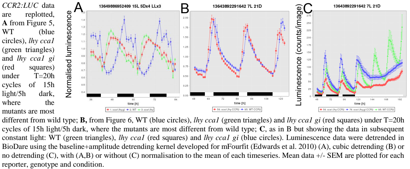
Figure 7. Conditional severity of the lhy cca1 mutant phenotype.
