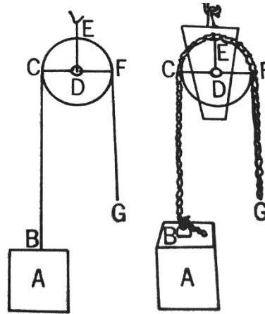
Figure 2. Pulley from Mechanicorum Liber . Drake and Drabkin, Mechanics in Sixteenth-Century , 305
