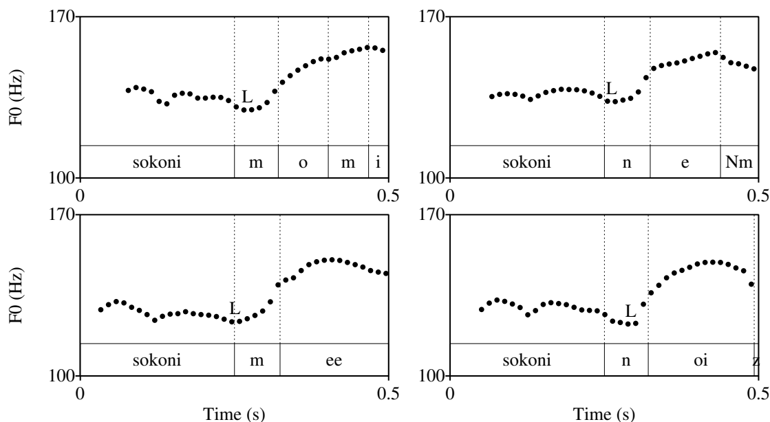
Figure 3.16: Examples of the utterance-medial F0 valley alignment: from the top on the left to the bottom on the right, /momizi/ ‘red leaves’ (CVCV), /neN+maku/ ‘mucous membrane’ (CVN), /mee+niti/ ‘the anniversary of somebody’s death’ (CVR), and /noizu/ ‘noise’ (CVV). The first vertical dotted line indicates C0 (the beginning of the target sequence).
