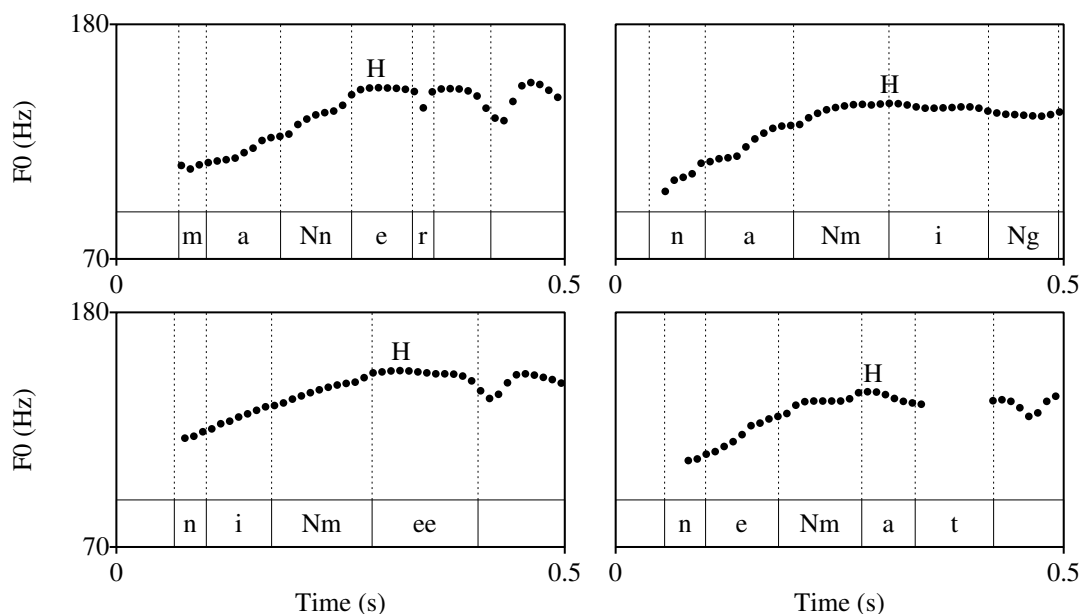
Figure 5.5: Examples of the F0 peak location for the phrase tone of an unaccented accen-tual phrase whose initial syllable is CVN: /maNneri/ ‘mannerism’, /naNm i Ng/ ‘refugee’, /nimeNsee/ ‘bilateral’ and /neNmatu/ ‘the end of the year’ (N is a moraic nasal).
