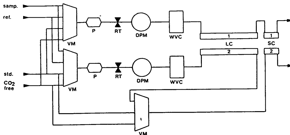
Figure 2.5. Functional diagram of the air circuit used for measurement and calibration. VM: group of valves working as a manifold; P: diaphragm pump; RT: needle valve and rotameter; DPM: dew-point meter; WVC: water vapour condenser; LC1, LC2: long cells of the IRGA; SC1, SC2: short cells of the IRGA. The differential pressure meter, individual solenoid valves, and blow-offs have not been included in the diagram to simplify it. Detailed diagrams are given by Sandford (1987).
