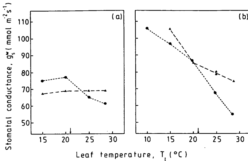
Figure 5.2. Relationship between stomatal conductance ( g_s^w ) and leaf temperature ( T_l ) under constant D_s^w=10 \text{ mmol mol}^{-1} ( \Delta ), and under constant h_s=0.60 ( \bullet ). (a) Mean of three plants from set A, I=200 \mu\text{mol m}^{-2} \text{s}^{-1} . (b) Typical plant from set B, I=340 \mu\text{mol m}^{-2} \text{s}^{-1} . The arrow above the temperature axis shows the point at which humidity is identical for both treatments. Both treatments were applied to the same leaves of the same plants. All measurements were taken at \chi_s^c=350 \mu\text{mol mol}^{-1} .
