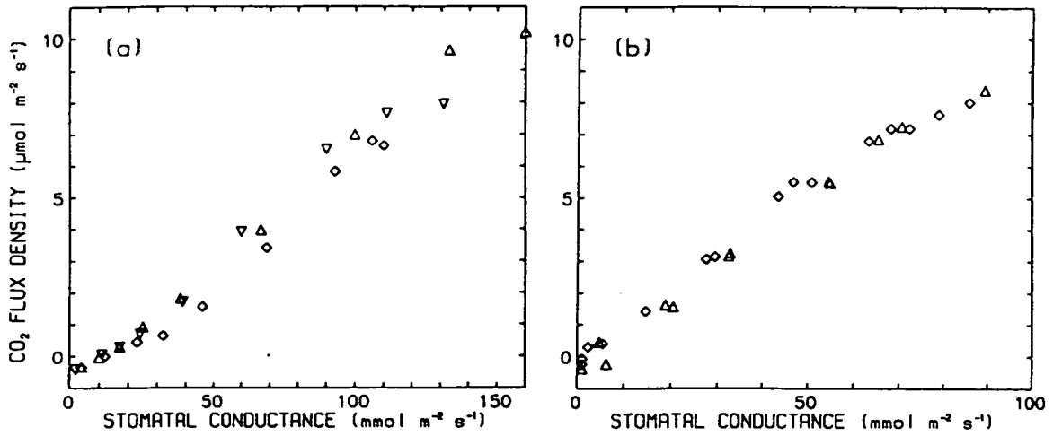
Figure 4.4. CO 2 flux density vs. stomatal conductance, measured under changing photon flux densities. Same data as in Figs. 4.2 & 4.1. D_s^w=10 mmol mol -1 , \chi_s^c=350 μmol mol -1 , T_1=20 °C. (a) Three plants from set A, (b) two plants from set B. Symbols indicate data from different plants.
