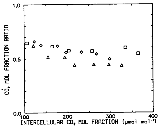
Figure 6.8. Relationship between the \chi_i^c/\chi_s^c ratio and intercellular \text{CO}_2 mol fraction ( \chi_i^c ) measured at constant leaf temperature and leaf surface water vapour deficit ( T_l = 20^\circ\text{C} , D_s^w = 7 \text{mmol mol}^{-1} , and I = 490 \mu\text{mol m}^{-2} \text{s}^{-1} ). The different symbols indicate data from different plants.
