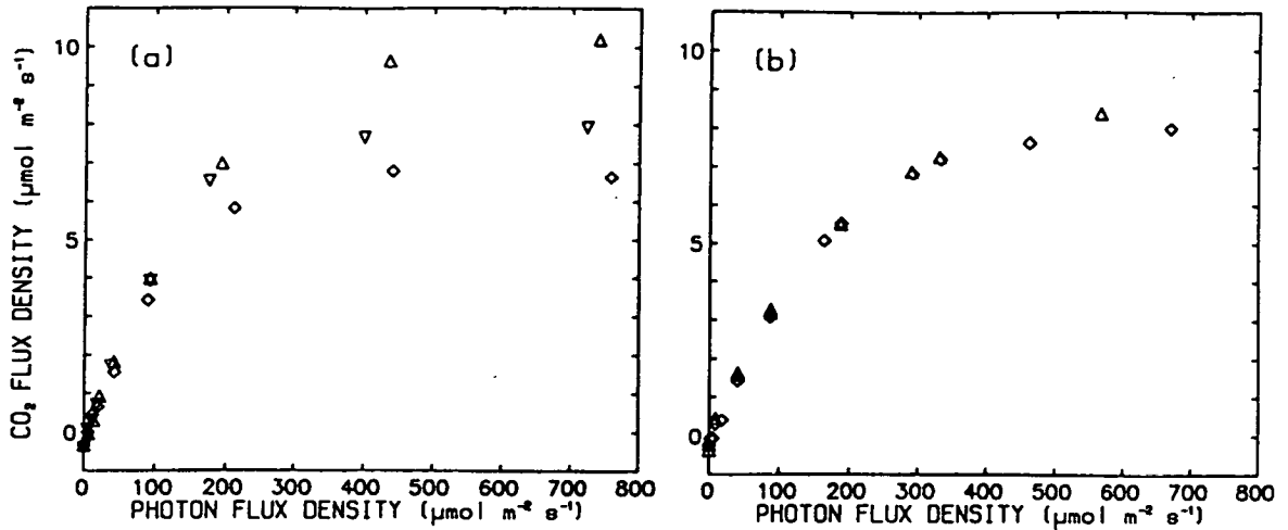
Figure 4.2. CO 2 flux density vs. photon flux density of white light. D_s^w=10 \text{ mmol mol}^{-1} , \chi_s^c=350 \text{ μmol mol}^{-1} , T_1=20 \text{ °C} . (a) Three plants from set A, (b) two plants from set B. Symbols indicate data from different plants.
