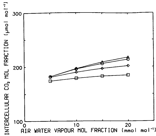
Figure 6.10. Simulated relationship between intercellular CO 2 mol fraction ( \chi_i^c ) and bulk air water vapour molar fraction ( \chi_a^w ) for (□) g_b^w = 100 , (◇) g_b^w = 200 , (○) g_b^w = 500 , and (△) g_b^w = 1000 mmol m -2 s -1 , under constant leaf temperature and bulk air CO 2 mol fraction ( T_l = 20 °C, \chi_a^c = 350 μmol mol -1 , and I = 500 μmol m -2 s -1 ). Simulation based on response data in Figs. 6.3, 6.4, & 6.5.
