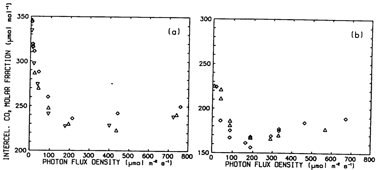
Figure 4.3. Intercellular CO 2 concentration vs. photon flux density of white light. D_s^w=10 \text{ mmol mol}^{-1} , \chi_s^c=350 \text{ μmol mol}^{-1} , T_1=20 \text{ °C} . Data from the same experiment as that in Fig. 4.2. (a) Three plants from set A, (b) two plants from set B. Symbols indicate data from different plants.
