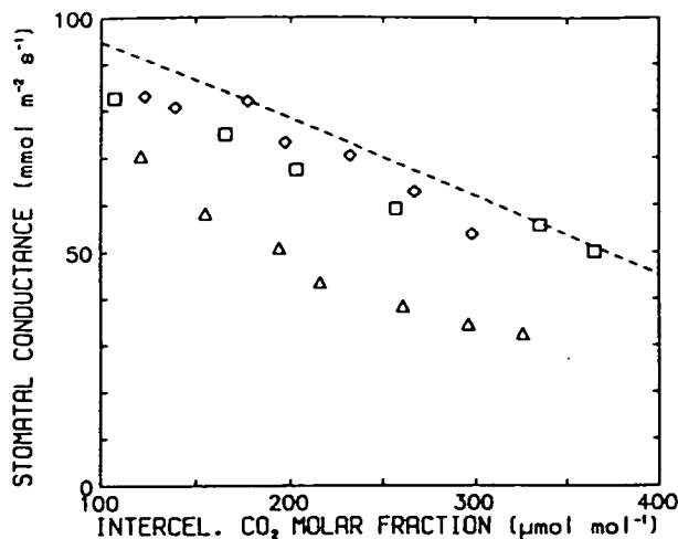
Figure 6.4. Relationship between stomatal conductance ( g_s^w ) and intercellular \text{CO}_2 mol fraction ( \chi_i^c ) measured at constant leaf temperature and leaf surface water vapour deficit ( T_l = 20^\circ\text{C} , D_s^w = 7 \text{ mmol mol}^{-1} , and I = 490 \mu\text{mol m}^{-2} \text{ s}^{-1} ). The different symbols indicate data from different plants, the dashed line is the relationship used in the model.
