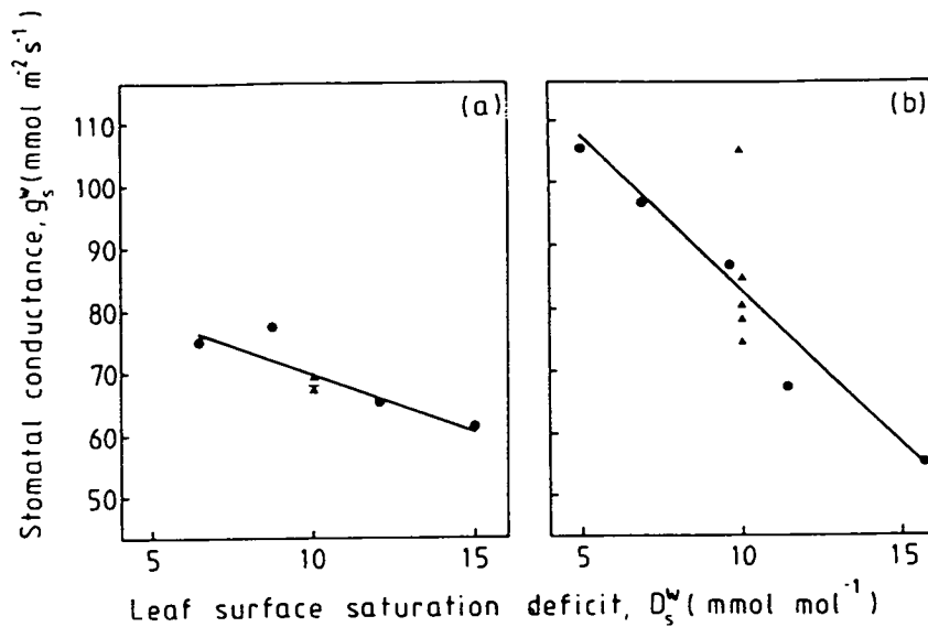
Figure 5.4. Relationship between stomatal conductance ( g_s^w ) and water vapour deficit at the leaf surface ( D_s^w ), measured under changing leaf temperature ( T_l ) in the range 10–29 °C. Symbols as in Fig. 5.2. (a) Mean of three plants from set A, R^2=0.77 , P=0.004 . (b) Typical plant from set B, R^2=0.75 , P=0.001 . The triangle with an underscore represents three overlapping data points.
