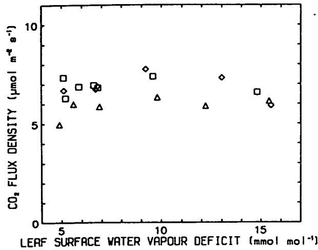
Figure 6.6. Relationship between \text{CO}_2 flux density ( A ) and leaf surface water vapour deficit ( D_s^w ) measured at constant leaf temperature and intercellular \text{CO}_2 mol fraction ( T_l = 20^\circ\text{C} , \chi_i^c \approx 200 \mu\text{mol mol}^{-1} , and I = 490 \mu\text{mol m}^{-2} \text{ s}^{-1} ). The different symbols indicate data from different plants.
