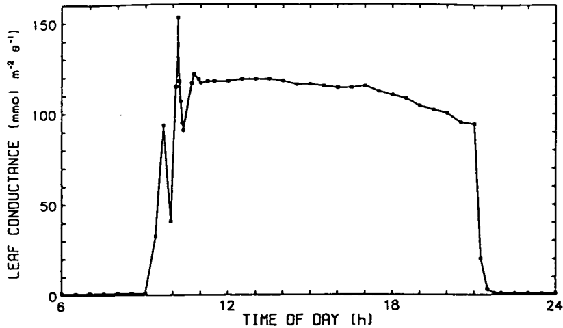
Figure 3.8. Leaf conductance of an ivy leaf throughout a day under constant conditions. Typical response under 340 \mu\text{mol m}^{-2} \text{s}^{-1} of white light. D_s^w=10 \text{ mmol mol}^{-1} , T_1=20 \text{ }^\circ\text{C} , \chi_a^c=350 \mu\text{mol mol}^{-1} . The photoperiod was from 9:00 to 21:00.
