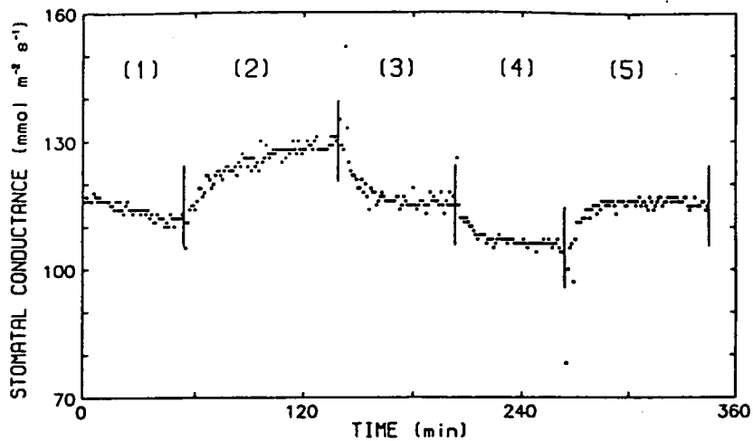
Figure 6.2. Effect of boundary layer conductance ( g_b^w ) on stomatal conductance ( g_s^w ) in a typical leaf. g_b^w was altered by changing the wind speed. Five different treatments were applied in sequence: (1) g_b^w=750 \text{ mmol m}^{-2} \text{ s}^{-1} , \chi_i^c=200 \text{ } \mu\text{mol mol}^{-1} , D_s^w=7 \text{ mmol mol}^{-1} , \chi_a^c=345 \text{ } \mu\text{mol mol}^{-1} , D_a^w=8.1 \text{ mmol mol}^{-1} ; (2) g_b^w=360 \text{ mmol m}^{-2} \text{ s}^{-1} , bulk air mol fractions as in (1); (3) g_b^w=360 \text{ mmol m}^{-2} \text{ s}^{-1} , \chi_i^c=200 \text{ } \mu\text{mol mol}^{-1} , D_s^w=7 \text{ mmol mol}^{-1} ; (4) g_b^w=750 \text{ mmol m}^{-2} \text{ s}^{-1} and bulk air mol fraction as in (3); (5) restored to g_b^w=750 \text{ mmol m}^{-2} \text{ s}^{-1} , \chi_i^c=200 \text{ } \mu\text{mol mol}^{-1} , D_s^w=7 \text{ mmol mol}^{-1} . ( T_l=20 \text{ }^\circ\text{C} , and I=500 \text{ } \mu\text{mol m}^{-2} \text{ s}^{-1} ). The vertical bars indicate the times when conditions were changed.
