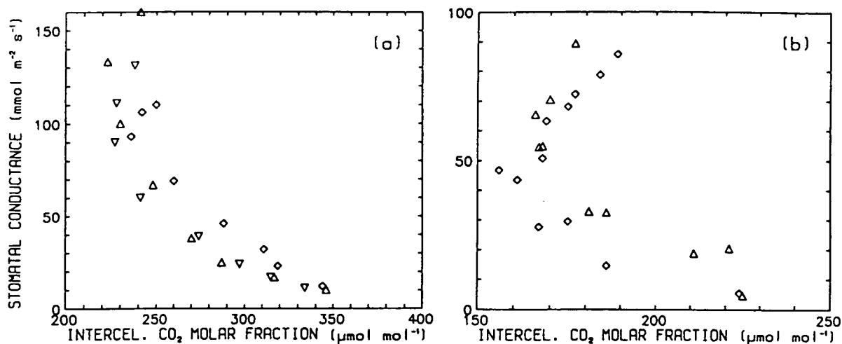
Figure 4.5. Stomatal conductance vs. intercellular CO 2 concentration, measured under changing photon flux densities. Same data as in Figs. 4.1 & 4.3. D_s^w = 10 \text{ mmol mol}^{-1} , \chi_s^c = 350 \text{ μmol mol}^{-1} , T_1 = 20 \text{ °C} . (a) plants from set A, (b) from set B. Symbols indicate data from different plants.
