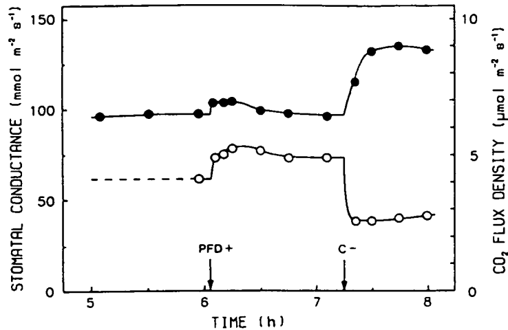
Figure 4.6. Responses of stomatal conductance (●) and CO 2 flux density (○) to increased photon flux density ( I ) and decreased intercellular CO 2 concentration ( \chi_i^c ) in a leaf in inverted position. Starting conditions: \chi_i^c = 220 \mu\text{mol mol}^{-1} , I = 500 \mu\text{mol m}^{-2} \text{s}^{-1} (white light), D_s^w = 7 \text{ mmol mol}^{-1} , T_i = 20 \text{ }^\circ\text{C} . C-: \chi_i^c reduced to 120 \mu\text{mol mol}^{-1} ; PFD+: I increased to 750 \mu\text{mol m}^{-2} \text{s}^{-1} .
