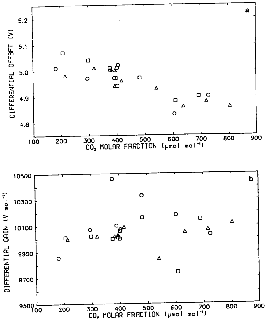
Figure 2.8. Sensitivity of the standardized IRGA calibration to the background CO 2 concentration. Plots of (a) the differential offset ( \bar{s}_{\text{null}} ), and (b) the differential gain or sensitivity ( \bar{\beta} ) of the IRGA vs. the reference molar fraction of CO 2 ( \chi_{\text{in}}^c ). Values shown were standardized to \chi_{\text{in}}^c = 350 \mu\text{mol mol}^{-1} . Data from 27 calibrations done on three different days (indicated with different symbols).
