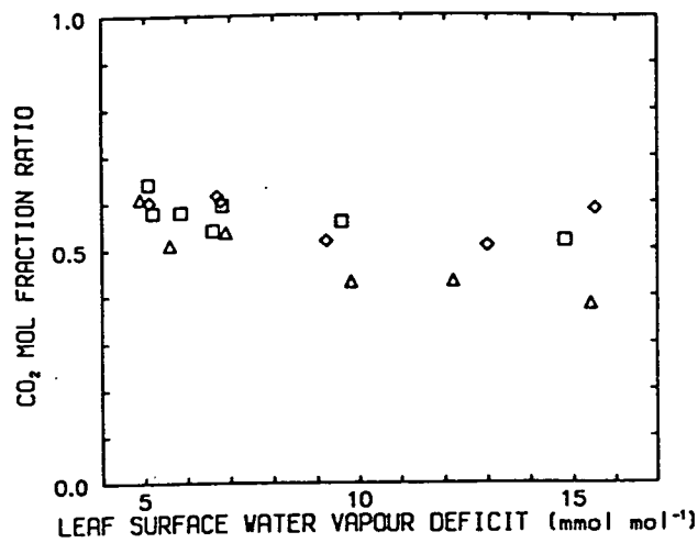
Figure 6.7. Relationship between the \chi_i^c/\chi_s^c ratio and leaf surface water vapour deficit ( D_s^w ) measured at constant leaf temperature and intercellular \text{CO}_2 mol fraction ( T_l = 20^\circ\text{C} , \chi_i^c \approx 200 \mu\text{mol mol}^{-1} , and I = 490 \mu\text{mol m}^{-2} \text{s}^{-1} ). The different symbols indicate data from different plants.
