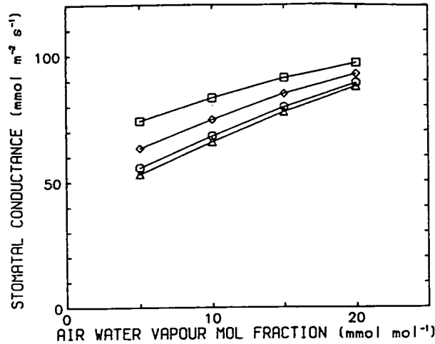
Figure 6.9. Simulated relationship between stomatal conductance ( g_s^w ) and bulk air water vapour molar fraction ( \chi_a^w ) for ( \square ) g_b^w = 100 , ( \diamond ) g_b^w = 200 , ( \circ ) g_b^w = 500 , and ( \triangle ) g_b^w = 1000 \text{mmol m}^{-2} \text{s}^{-1} , under constant leaf temperature and bulk air \text{CO}_2 mol fraction ( T_l = 20 ^\circ\text{C} , \chi_a^c = 350 \mu\text{mol mol}^{-1} , and I = 500 \mu\text{mol m}^{-2} \text{s}^{-1} ). Simulation based on response data in Figs. 6.3, 6.4, & 6.5.
