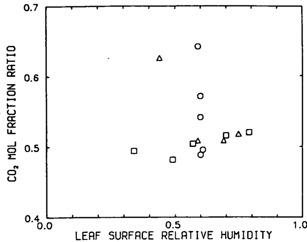
Figure 7.1. Ratio between intercellular and leaf surface \text{CO}_2 mol fractions vs. leaf surface relative humidity. Measured ( \square ) under constant temperature ( T_1=20^\circ\text{C} ), or changing temperature and ( \triangle ) constant leaf surface water vapour deficit ( D_s^w=10\text{ mmol mol}^{-1} ), or ( \circ ) constant leaf surface relative humidity ( h_s=0.60 ); I=340\text{ }\mu\text{mol m}^{-2}\text{ s}^{-1} . Data from one typical ivy plant from the experiment described in Chapter 5 obtained at the same time as data in Figs. 5.1b & 5.4b.
