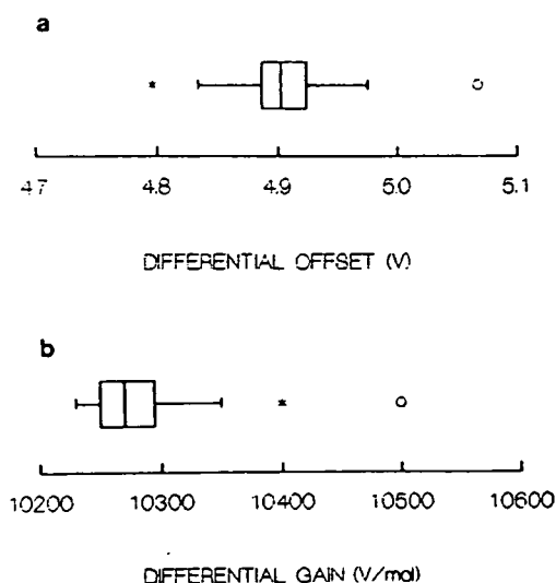
Figure 2.7. Box diagrams for the IRGA calibration data measured during a single day, and under the same reference \text{CO}_2 molar fraction ( \chi_{\text{in}}^{\text{c}} = 365 \mu\text{mol mol}^{-1} ). (a) standardized differential offset ( \bar{s}_{\text{null}} ), and (b) standardized differential gain ( \bar{\beta} ) of the IRGA. In a box diagram the crossbar at the center of the box is the median , the length of the box is the fourth spread , the lines extending from the end of the box give the tail length , and * or o indicate the location of outliers (see Emerson & Strenio, 1983).
