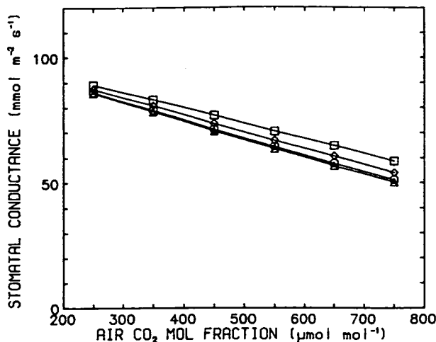
Figure 6.17. Simulated relationship between stomatal conductance ( g_s^w ) and bulk air \text{CO}_2 molar fraction ( \chi_a^c ) for ( \square ) g_b^w = 100 , ( \diamond ) g_b^w = 200 , ( \circ ) g_b^w = 500 , and ( \triangle ) g_b^w = 1000 \text{ mmol m}^{-2} \text{ s}^{-1} , under constant leaf temperature and water vapour molar fraction in the bulk air ( T_l = 20 \text{ }^\circ\text{C} , \chi_a^w = 15 \text{ mmol mol}^{-1} , and I = 500 \text{ } \mu\text{mol m}^{-2} \text{ s}^{-1} ). The stomata were assumed to be insensitive to humidity. Simulation based on response data in Figs. 6.4, & 6.5.
