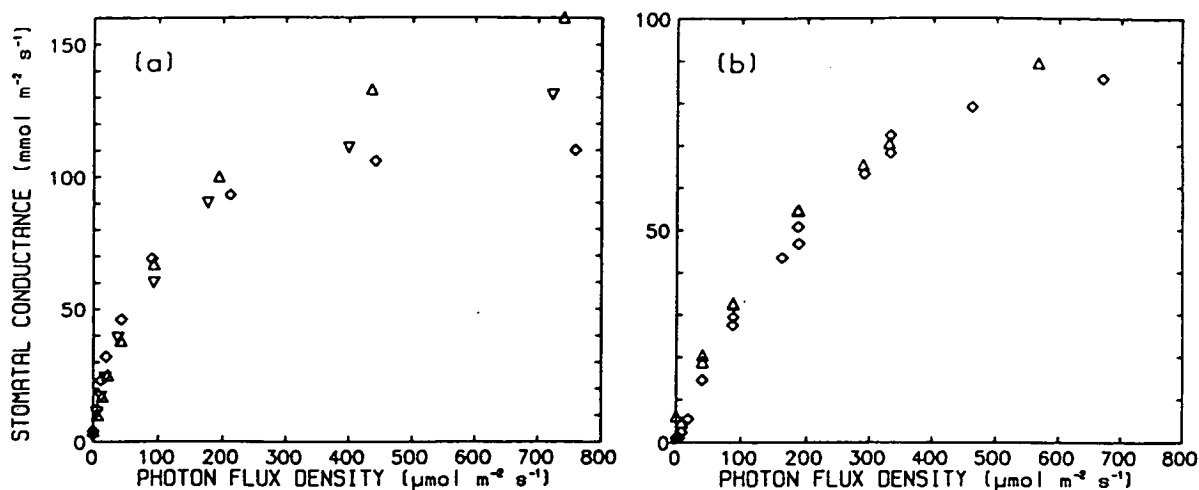
Figure 4.1. Stomatal conductance vs. photon flux density of white light. D_s^w=10 mmol mol -1 , \chi_i^c=350 μmol mol -1 , T_i=20 °C. (a) Three plants from set A, (b) two plants from set B. Symbols indicate data from different plants.
