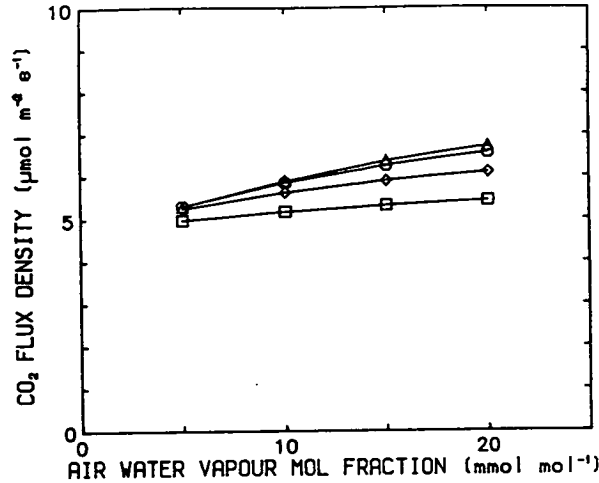
Figure 6.11. Simulated relationship between CO 2 flux density ( A ) and bulk air water vapour molar fraction ( \chi_a^w ) for (□) g_b^w = 100 , (◇) g_b^w = 200 , (○) g_b^w = 500 , and (△) g_b^w = 1000 mmol m -2 s -1 , under constant leaf temperature and bulk air CO 2 mol fraction ( T_l = 20 °C, \chi_a^c = 350 μmol mol -1 , and I = 500 μmol m -2 s -1 ). Simulation based on response data in Figs. 6.3, 6.4, & 6.5.
