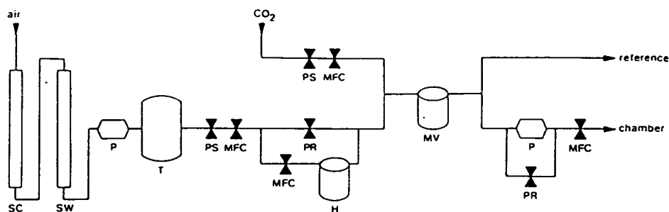
Figure 2.2. Air circuit diagram of air-conditioning block. SC: CO 2 scrubbing column; SW: water vapour scrubbing column; P: diaphragm pump; T: steel tank; H: humidifier; MFC: mass-flow controller; PS: pressure regulator; PR: pressure relief valve; MV: mixing vessel. Detailed diagrams are given by Sandford (1987).
