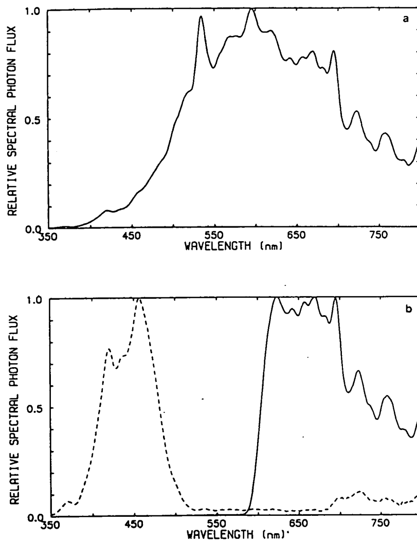
Figure 2.4. Photon spectra of the light sources used in the gas exchange experiments. (a) HQI-R lamp with a heat filter, as seen through the chamber window; (b) with a red filter (—); and with a blue filter (-----). Measured with an optical spectrum analyser (model 6800; with a 6100 monochromator, with a 0.9 mm slit installed; and a 6118 photo-tube detector. Monolight Instruments Ltd., Weybridge, Surrey, U.K.).
