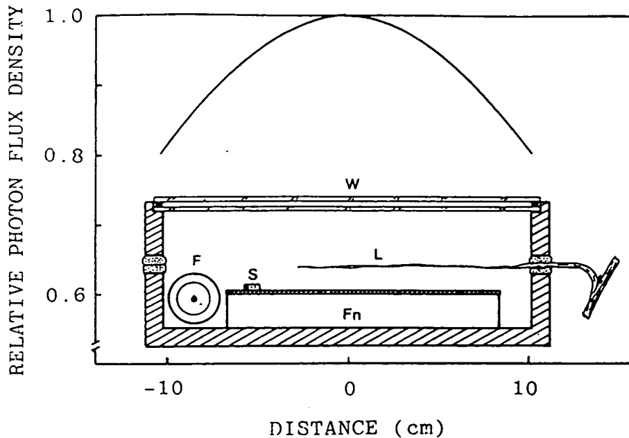
Figure 2.3. Spatial distribution of photon flux density on a horizontal plane situated 50 cm below a vertically positioned metal-halide reflector lamp (Wotan 'power-star'; HQI-R 250 W/NDL; Wotan Lamps Ltd., London). Measured with a Li-Cor cosine corrected PAR sensor (type Li-190SB, Li-Cor Ltd., Lincoln, Nebraska). A diagram of a lengthwise cross-section of the leaf chamber is overlaid. L: leaf, S: light sensor, W: window, F: fan, Fn: fins for heat exchange. Drawn to scale, width of the chamber: 12.4 cm.
