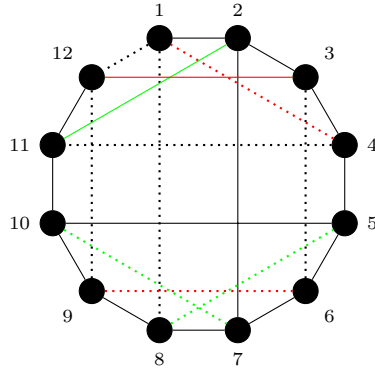
Figure 4.14: The 12-vertex sporadic maximal connected cyclotomic \mathcal{L} -graph S_{12} .
