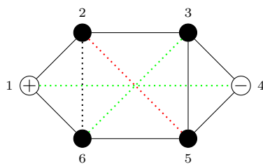
Figure 4.8: The 6-vertex sporadic maximal connected cyclotomic charged \mathcal{L} -graph \mathcal{S}'_6 .
