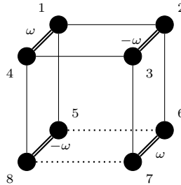
Figure 4.10: The 8-vertex sporadic maximal connected cyclotomic \mathcal{L} -graph \mathcal{S}_8^*
