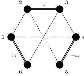
Figure 4.9: The 6-vertex sporadic maximal connected cyclotomic \mathcal{L} -graph \mathcal{S}_6^\dagger . (where \omega = \frac{1}{2} + \frac{\sqrt{-7}}{2} .)
