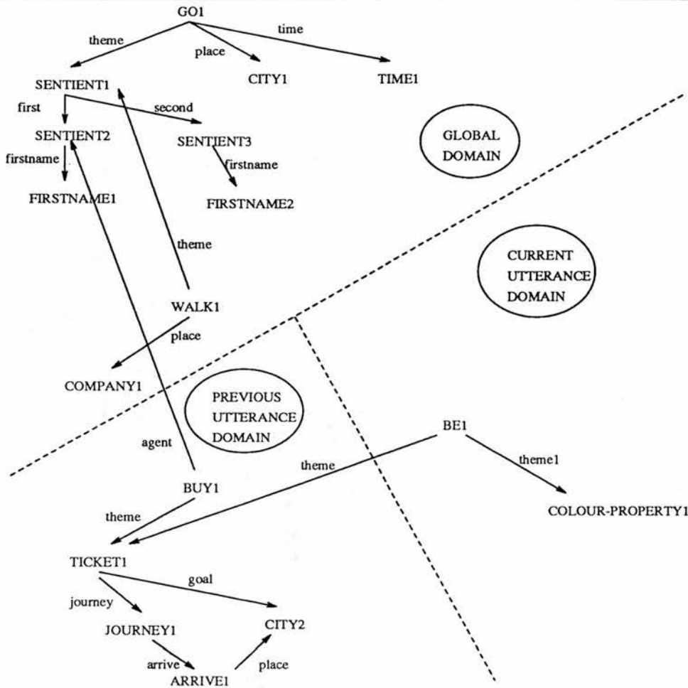
Figure 5-6: A discourse model structured in terms of accessible domains
