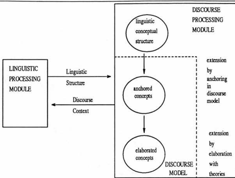
Figure 5–1: Interaction between the linguistic and discourse processing modules together with phases in conceptual extension
