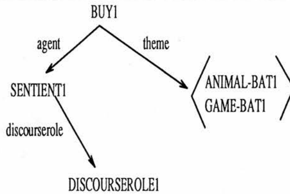
Figure 5–7: A concept related to two ‘virtual’ pegs for bat
