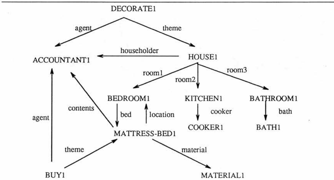
Figure 5–10: Discourse model after Then she bought a bed.
