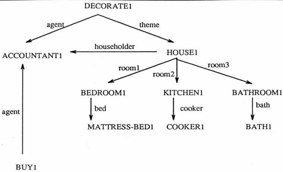
Figure 7-3: Discourse model after interpretation of The accountant decorated her new house. Then she bought
