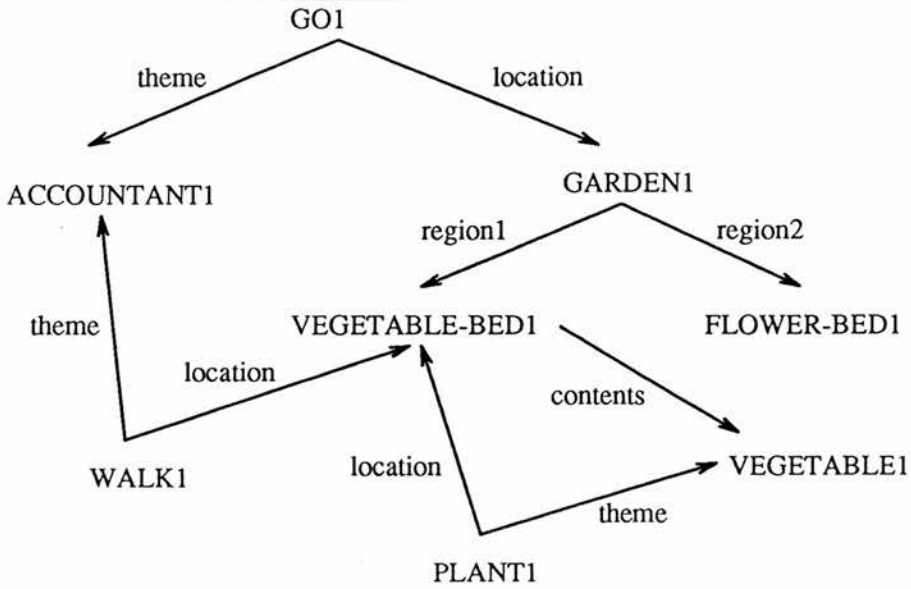
Figure 5-12: Discourse model after She walked across the bed planted with vegetables
