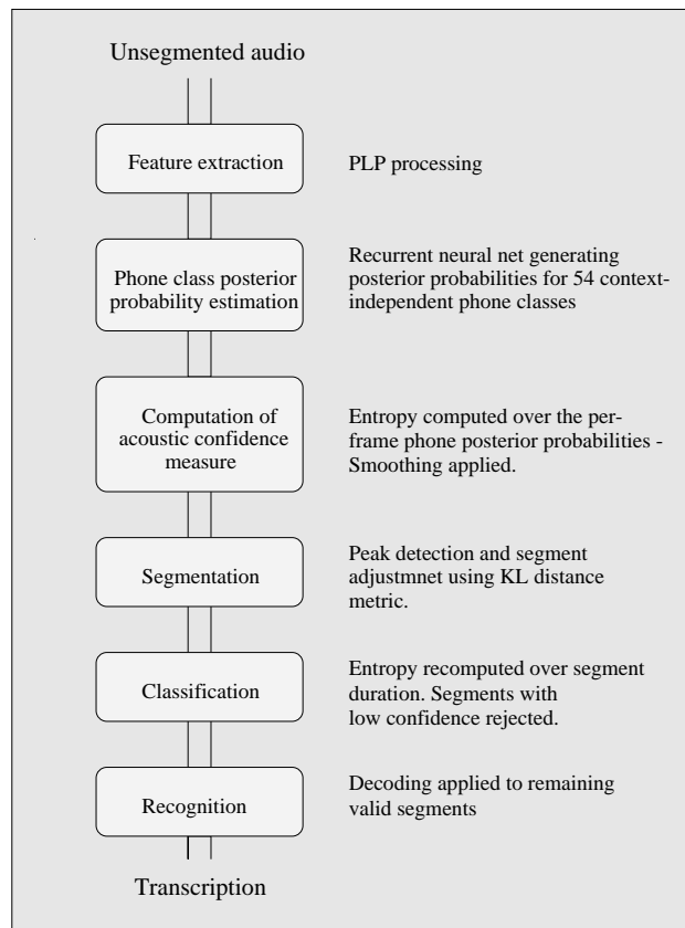
Figure 3: A summary of the segmentation system.
