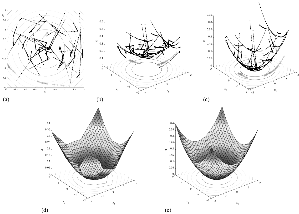
Figure 5. Top: (a) Toy data (trajectories (2-D) and contour of true potential. Estimated potential along the trajectories before (b) and after (c) alignment. Trajectories detected as difficult to align ‘outliers’ are shown by light crosses. Bottom: Learned (d) and true (e) potential function after training on the aligned trajectories.
