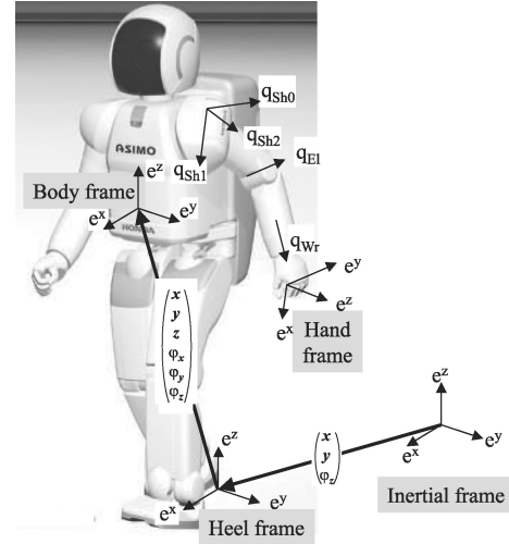
Figure 1. Kinematic model of the ASIMO humanoid robot (Gienger et al. 2005). In our experiments 22 upper body DOF were used ( 2 \times 7 DOF arms, 2 DOF head, 6 DOF torso), with the heel frame fixed.
