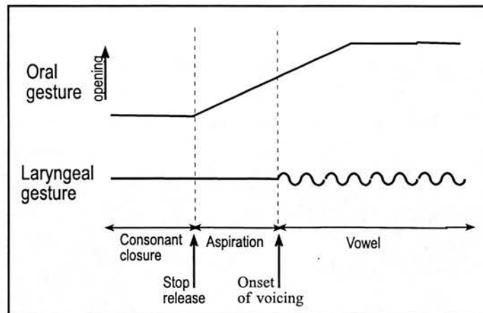
Figure 4.7: Schematic diagram of the relationship between aspiration duration and vowel duration.
