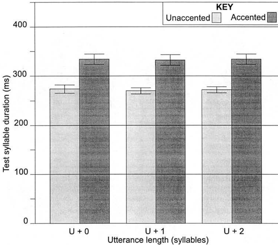
Figure 4.1: Mean test syllable duration (ms) in Keyword Series B for all keywords, excluding part , cap , dog , speck and port . Data points = 396; missing = 3.8%. Here and throughout, error bars represent two standard errors either side of the mean: this interval contains the population mean with 95% confidence.
