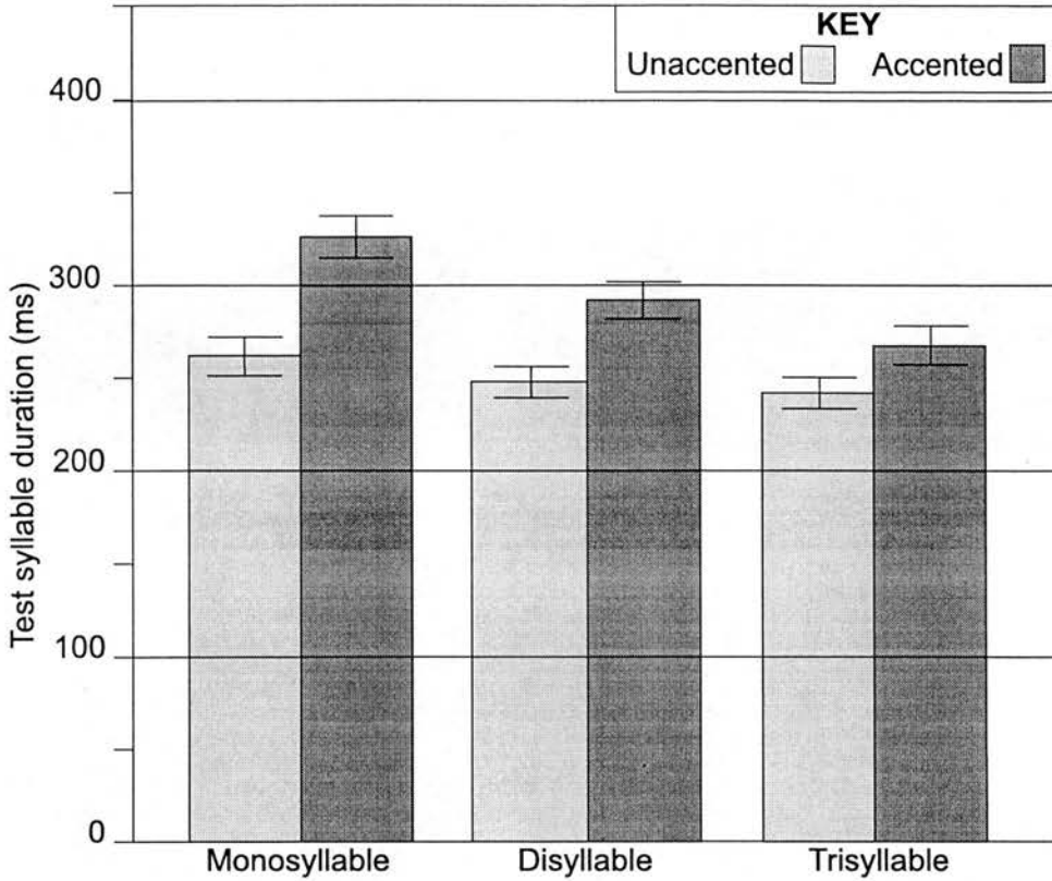
Figure 4.2: Mean test syllable duration (ms) in Series A for right-headed keywords excluding port : data points = 252; missing = 3.8%.
