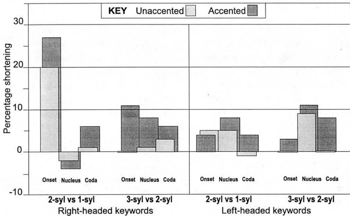
Figure 4.4: Proportional word-level shortening in monosyllabic, disyllabic and trisyllabic keywords in Series A. Proportional shortening is the difference in duration expressed as a percentage of syllable duration in the longer context. All right-headed keywords are included except port : data points = 252; missing = 3.8%. Left-headed keywords are fish , mace , mend and send : data points = 144; missing = 2.0%.
