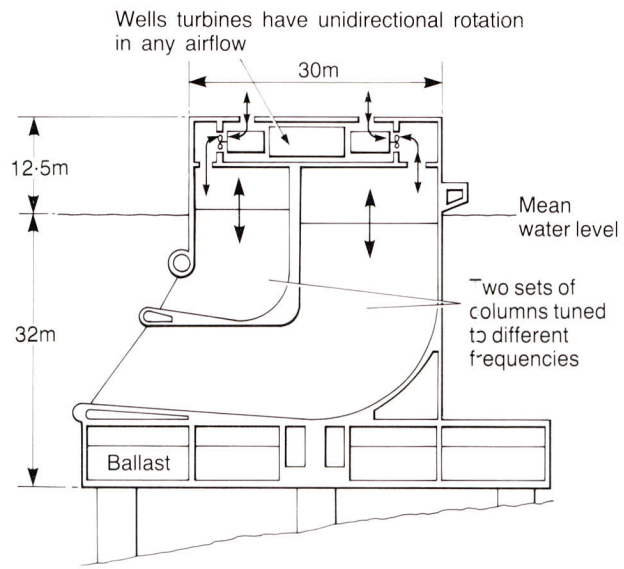
TYPICAL CROSS SECTION
