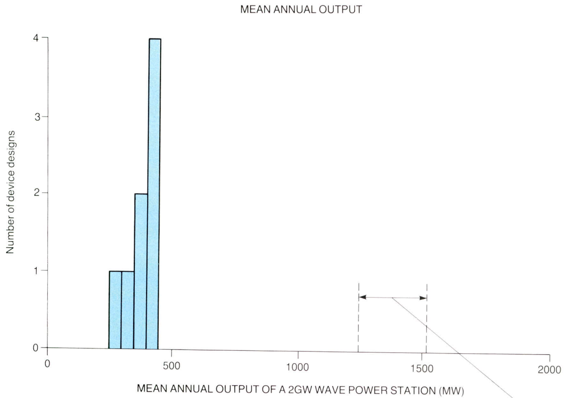
Fig. 10.3 The mean annual output and load factor of the various wave energy devices shown in histogram form
