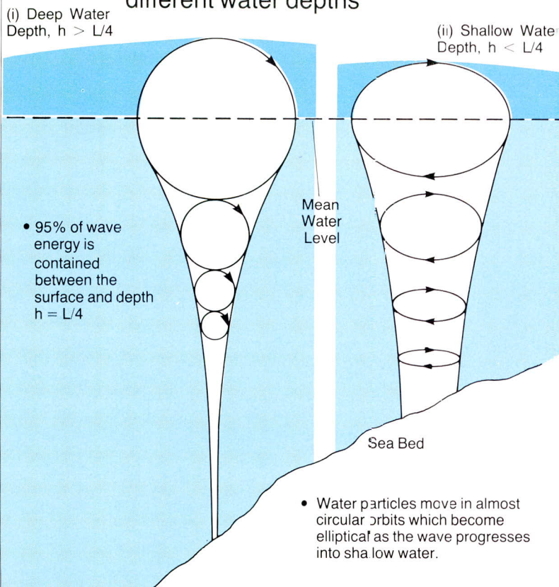
Fig. 3.2 Particle orbits for different water depths
