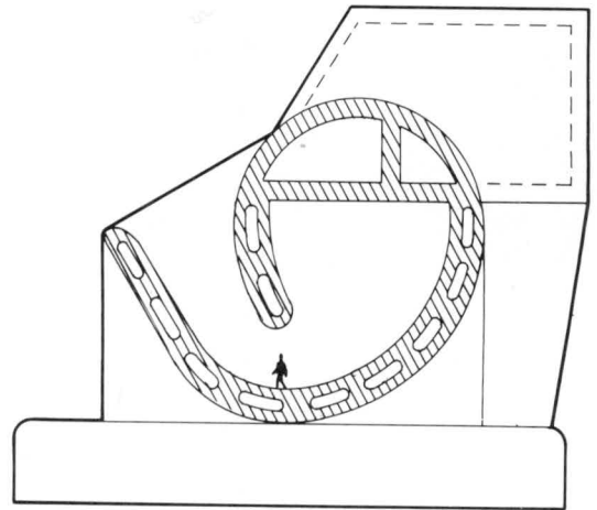
Vickers Terminator
