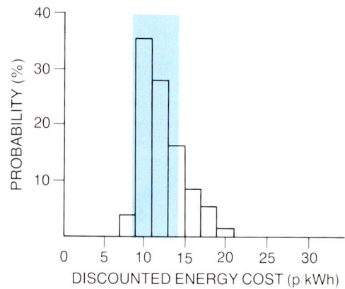
Vickers OWC (terminator)
