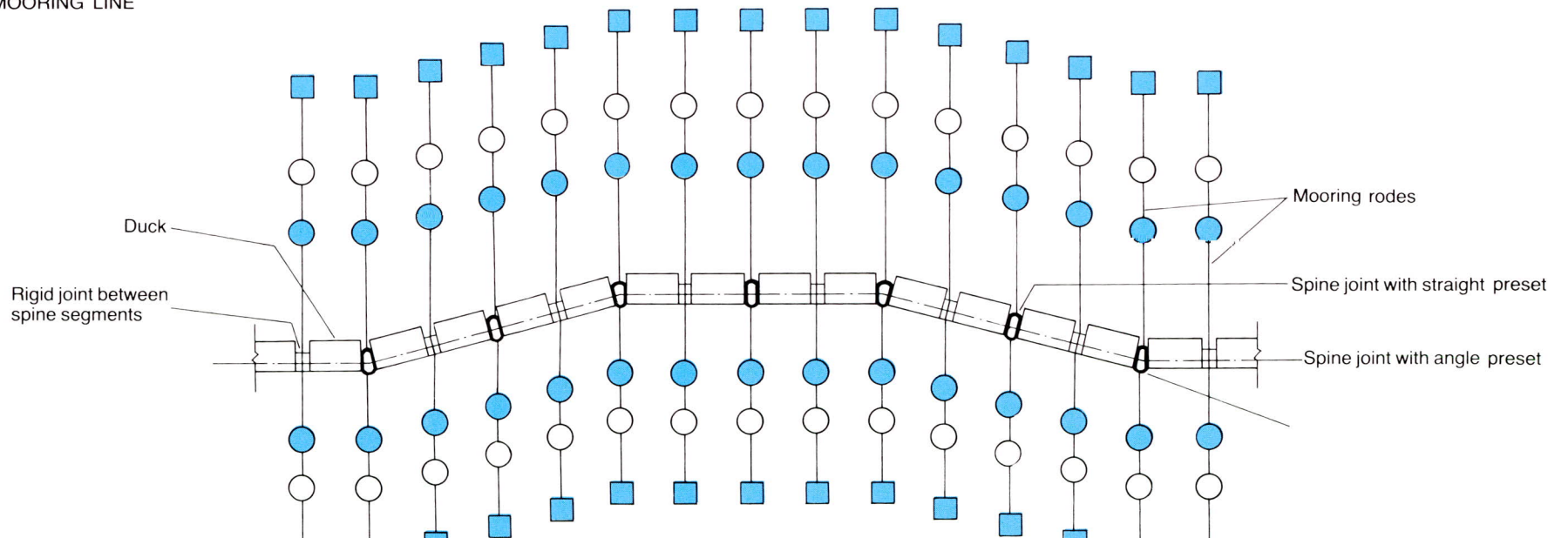
PLAN OF MOORING SYSTEM
