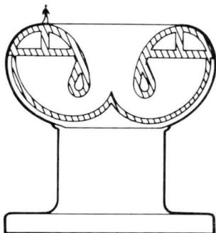
Vickers Attenuator
