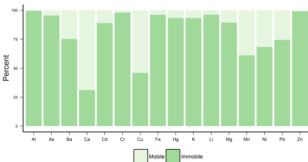
Figure 3.9: Percentage of 16 elements classified as "mobile" and "immibile" as per Kirsch et al. (2014). Data in Table 3.4.
