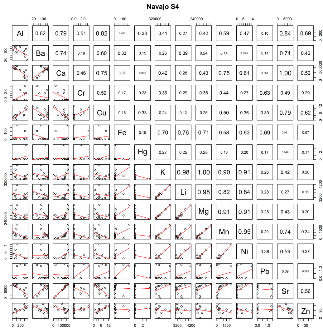
Figure D.11: Correlation matrix for Navajo S4 elements.
