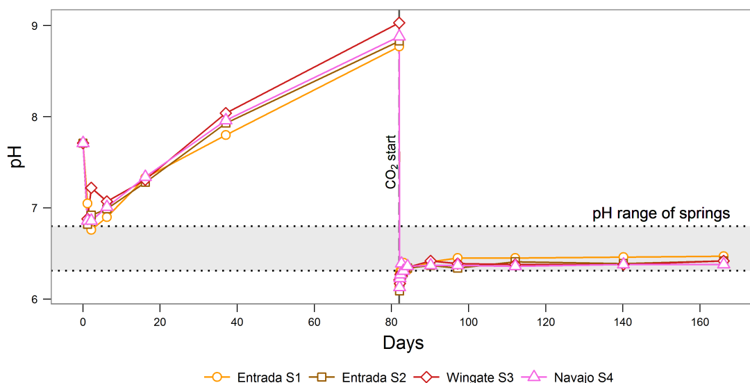
Figure 4.7: pH values for the batch reaction experiment using water collected from Crystal Geysir, and rock samples collected from the nearby San Rafael Swell, Utah (see Figure 2.1, Chapter 2). CO 2 flow commences at day 82. Shaded area indicates the field-measured pH values of the Green River spring waters, Table 4.1).
