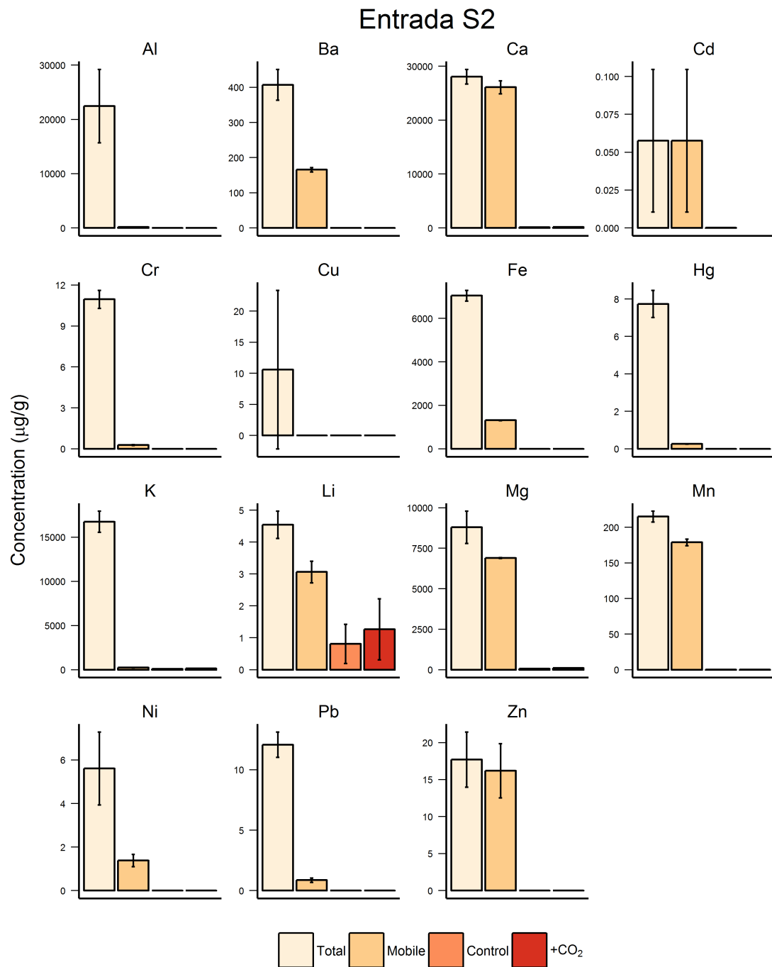
Figure 4.20: Concentrations of 15 elements leached from Entrada S2 sample during Control (Days 0 - 82) and +CO 2 (Days 82 - 163) batch experiments, compared with the mobile fractions determined by the sequential extraction procedure (SEP), and the sum of the (SEP) steps representing bulk concentrations. Error bars are 2s. Data in Table 4.5.
