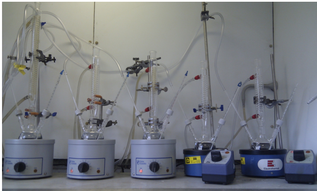
Figure 2.5: General setup of sandstone batch experiments.
