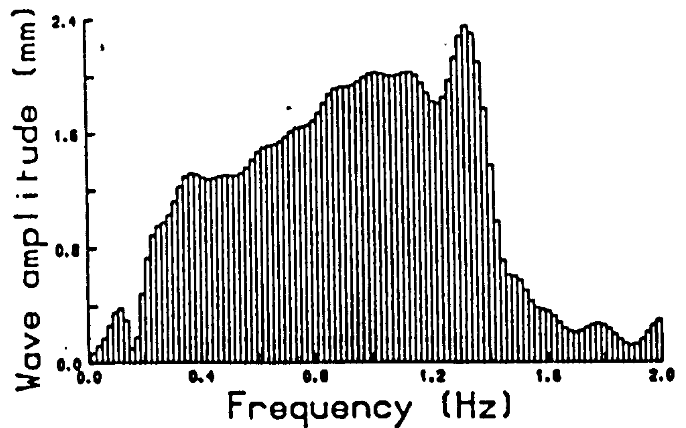
Figure 6.2: the composition of the wavefield ahead of the wave paddle is detected by the wave-gauge (see figure 6.1). The wave gauge record is shown on the left and its spectral content (calculated by FFT) on the right. Both diagrams courtesy of D.J.Skyner (see[114]).
