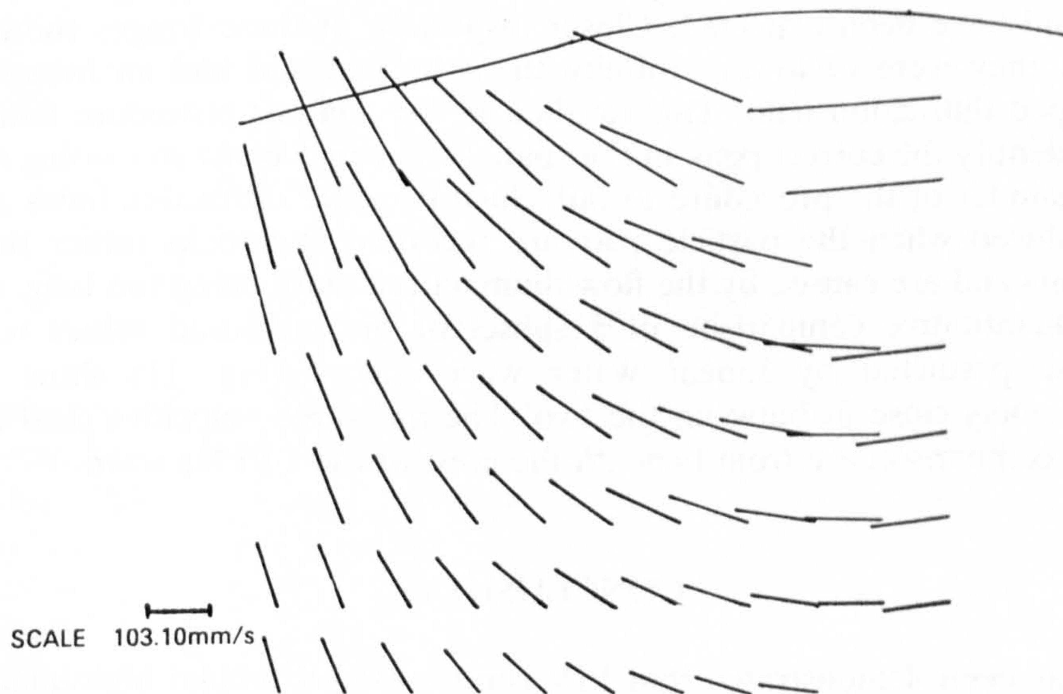
Fig. 9. Velocity map before crest of water wave (1.316 Hz, 1.559 m wavelength, 33 mm amplitude).
