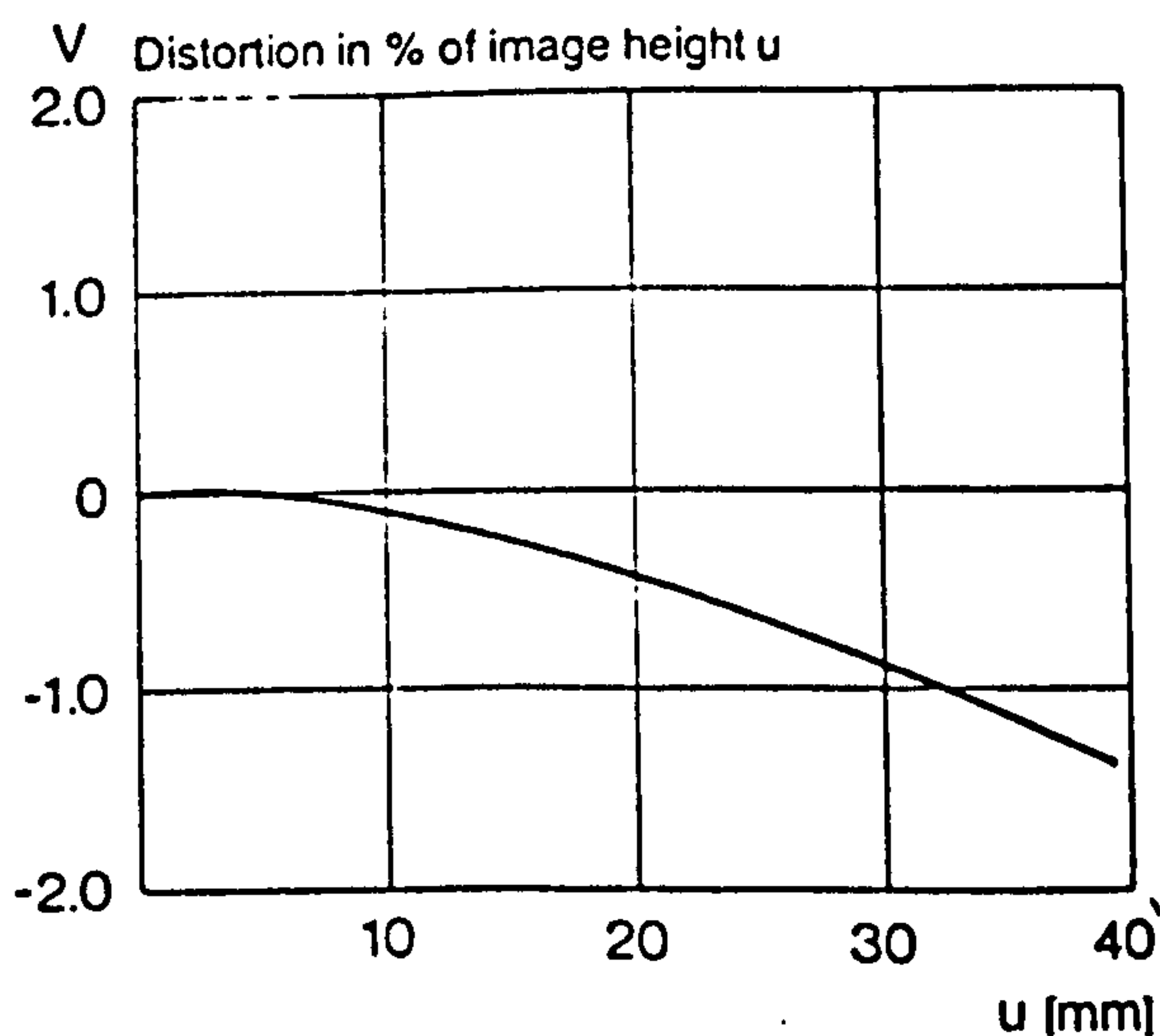
Figure 2.16: Distortion in % of image height
