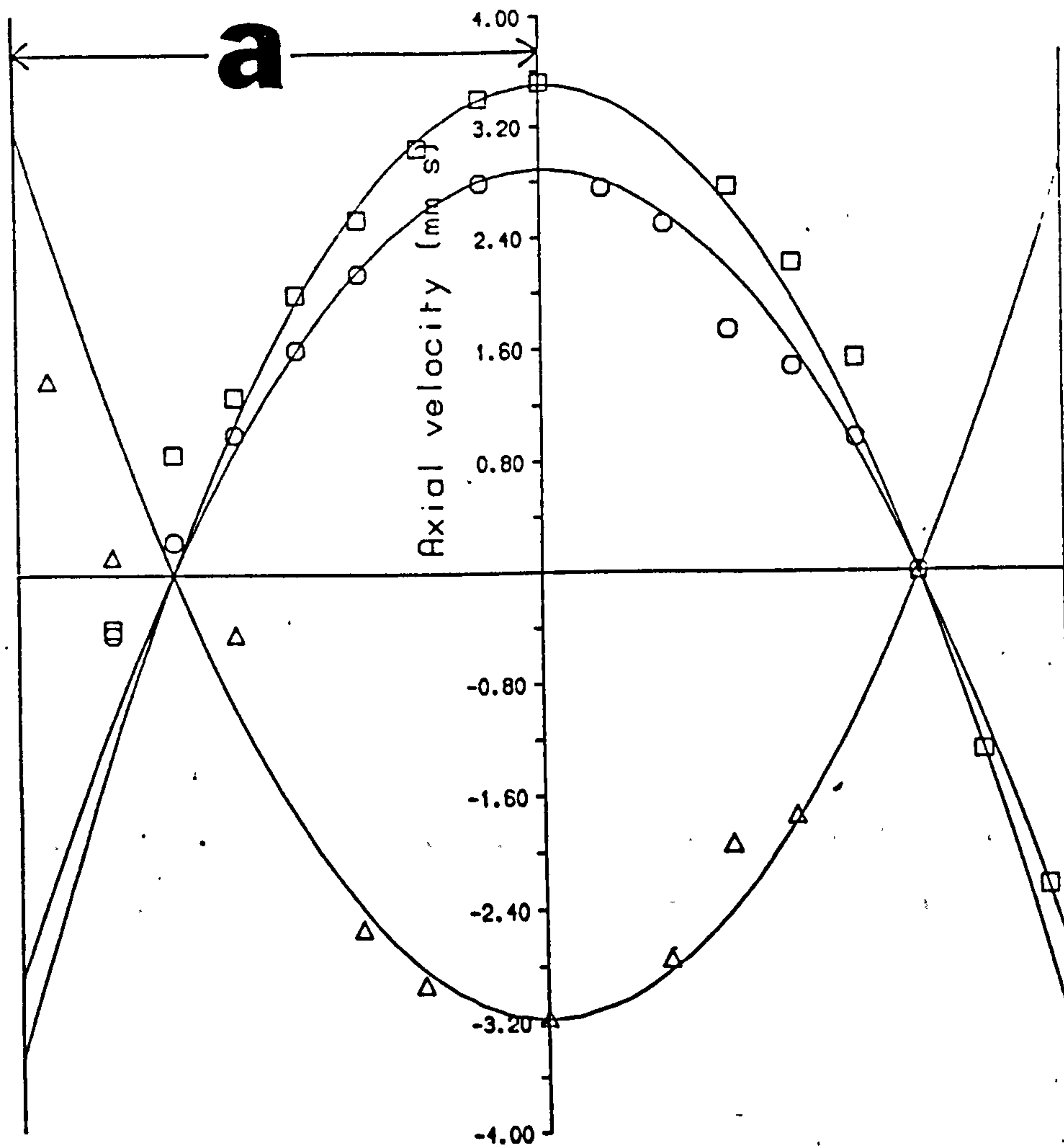
Figure 7.12: Experimentally measured axial velocities in the tube (symbols) and theoretical curves.
