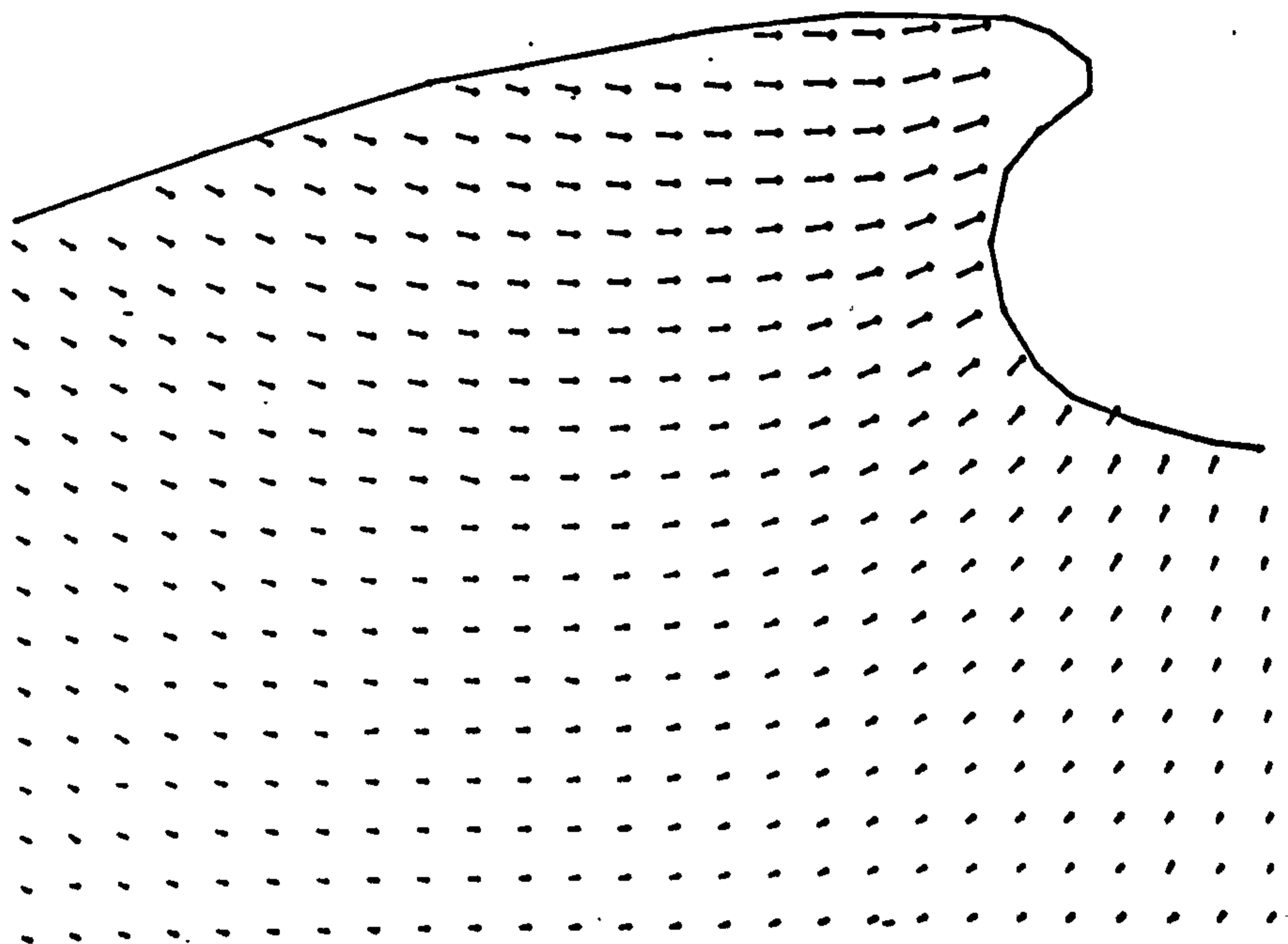
Figure 5 Velocity distribution generated from numerical model.
