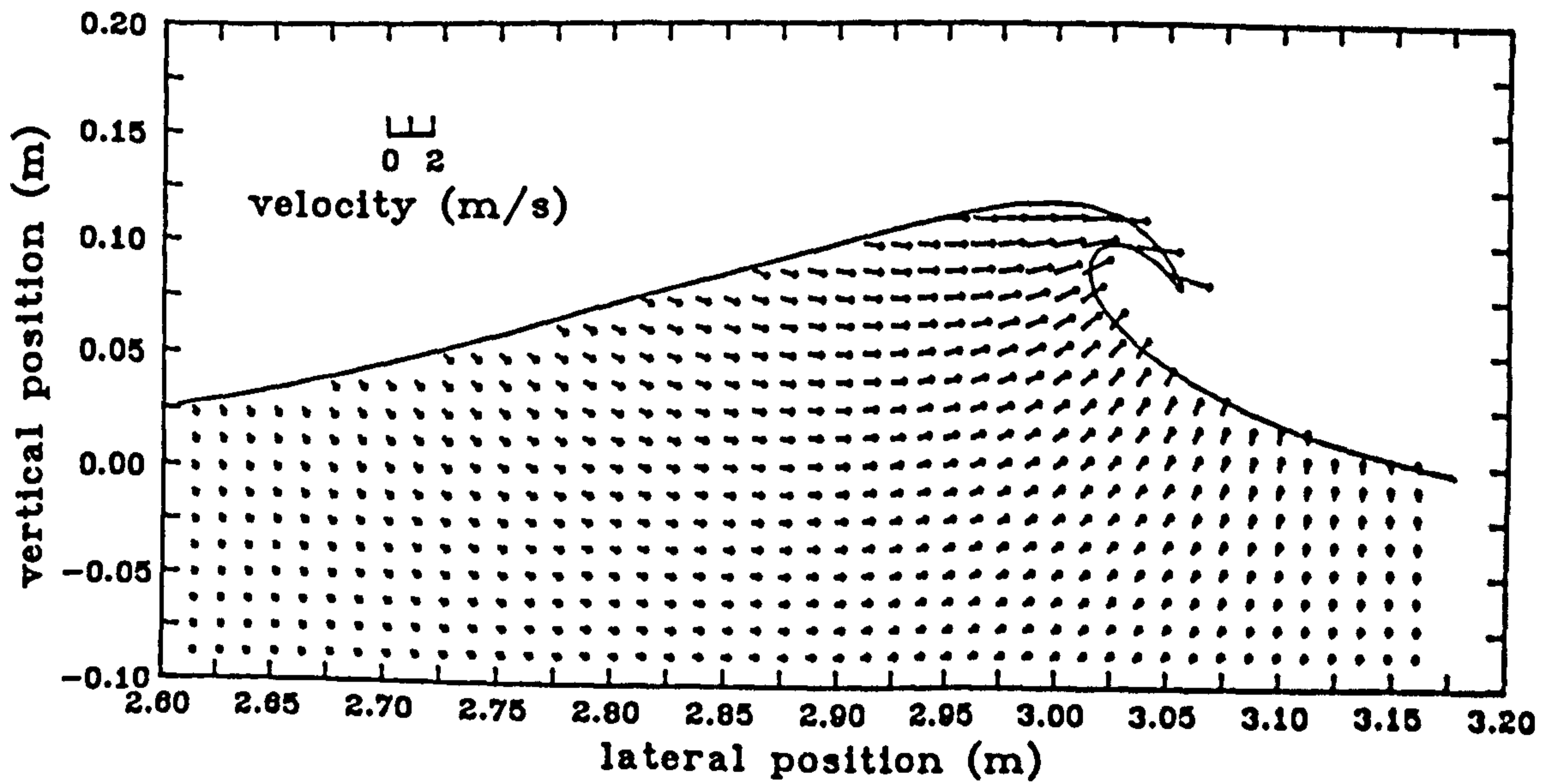
Figure 14: Numerically generated velocity field for an earlier phase of the wave.
