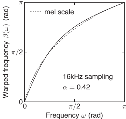
Figure 3: Frequency warping using the all-pass function. At a sampling frequency of 16 kHz, \alpha = 0.42 provides a good approximation to the mel scale.
