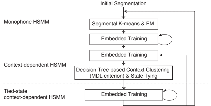
Figure 4: Overview of HMM training stages for HTS voice building.
