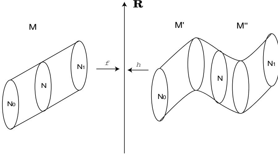
FIGURE 1. f and its splitting h .
