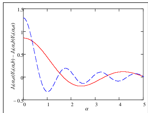
Figure 3. Equation (6), — [0.65, 2.5], - - [0.65, 5].
