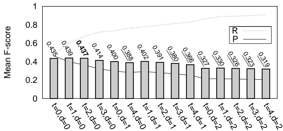
Figure 4.12: Window size results for combined (token and dependency) model. The f-score of the system that achieves the highest mean rank is in bold and those that are statistically distinguishable from the best are underlined.
