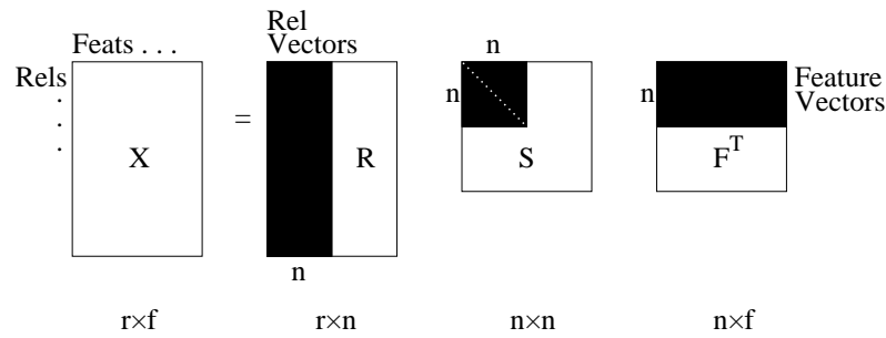
Figure 5.4: Matrix visualisation of singular value decomposition (SVD).
