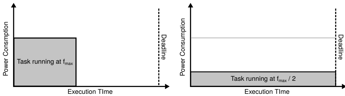
Figure 1.2: The same task is executed on two different voltage and frequency levels. The left side shows the task being executed on the maximum frequency. It finishes well before its deadline. The right side shows the task's execution with half that frequency. Here, execution ends right at the deadline. Due to a quadratic relation between voltage and dynamic core power, energy is significantly reduced (source [5]).
