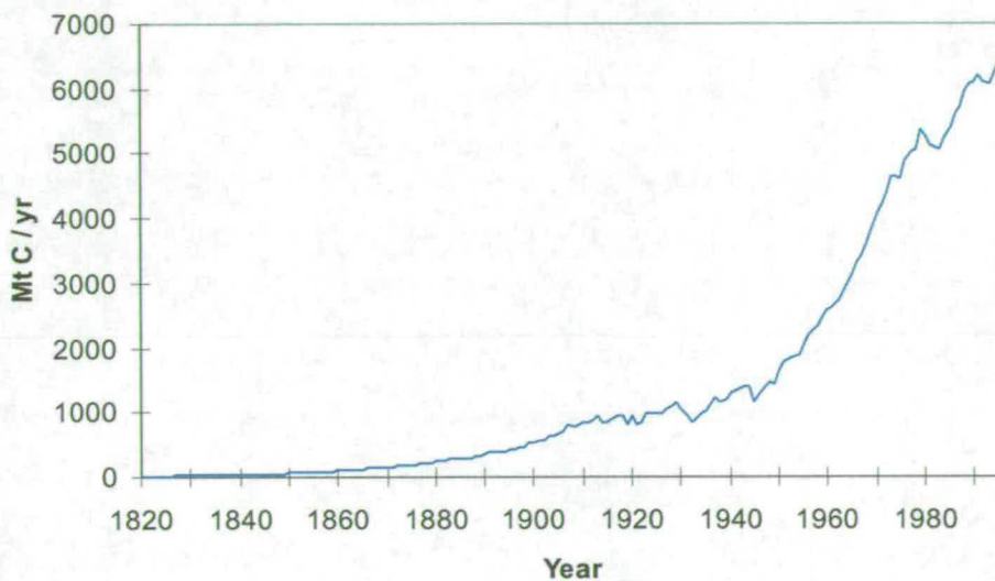
Figure 2.3: Global carbon emissions from fossil fuel combustion and cement production. MtC/yr over 1820-1996 [9]
