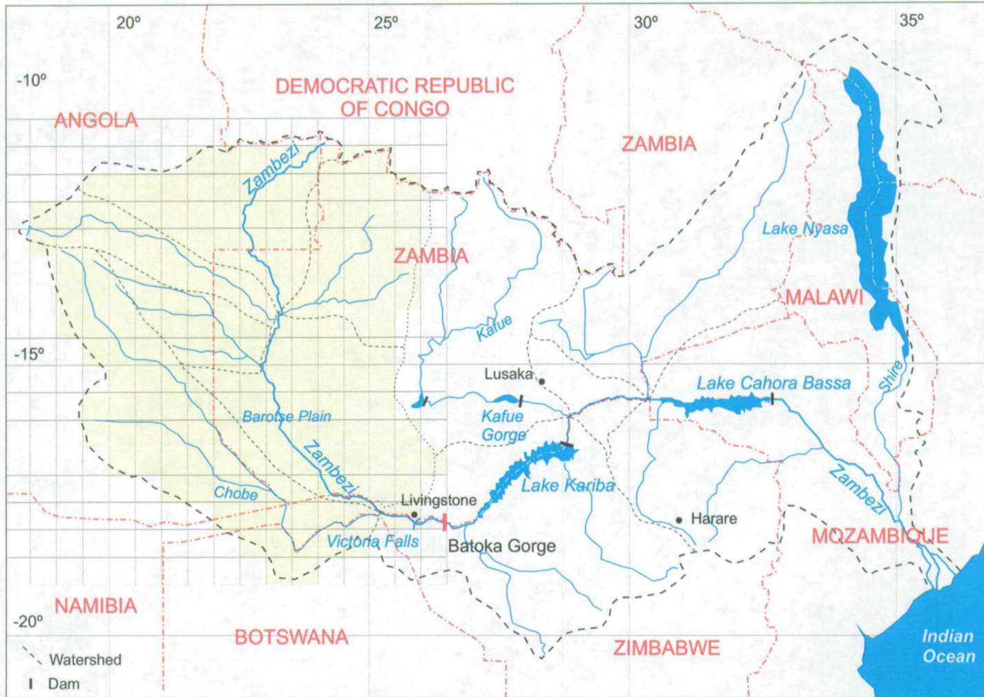
Figure 7.6: Zambezi Basin and aggregation mask
