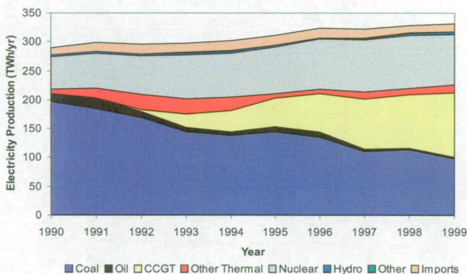
Figure 3.5: UK electricity generation by fuel source 1990-98 (TWh/yr) [84, 85]
