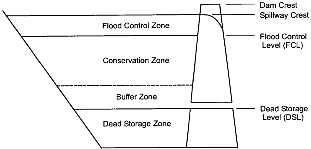
Figure 5.3: USACE defined reservoir storage zones and levels [173]
