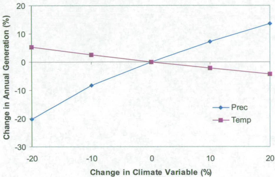
Figure 7.11: Sensitivity of annual generation to changes in precipitation and temperature
