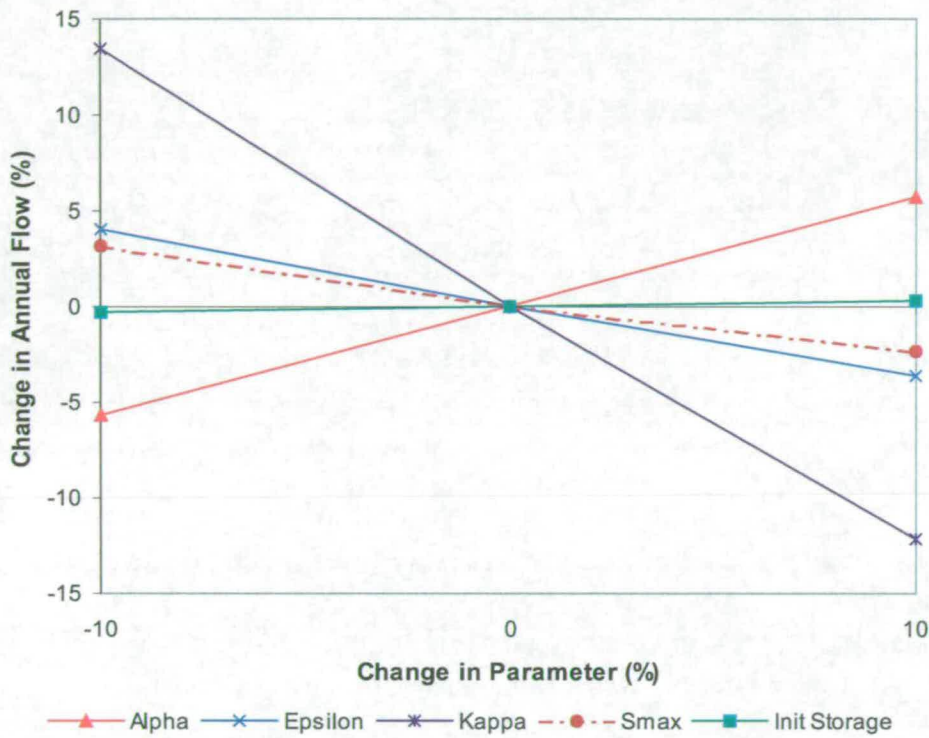
Figure A.1: Annual flow sensitivity to WatBal parameter values
