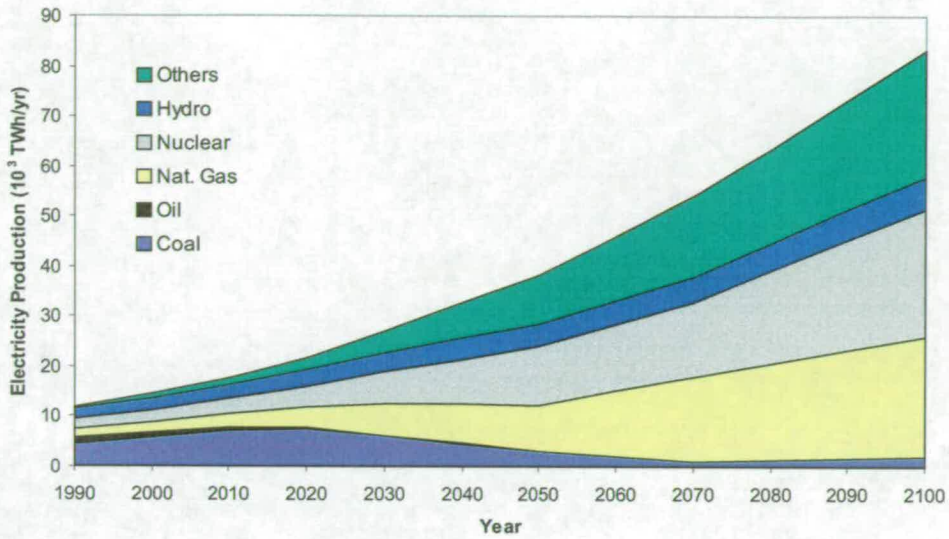
Figure 3.3: High growth WEC/IIASA electricity supply scenario A1 [74]
