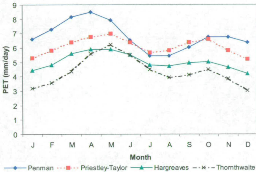
Figure 6.5: Potential evapotranspiration method comparison for Blue Nile [140]
