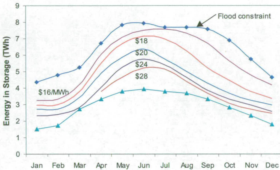
Figure 5.5: Marginal value of water in storage [179]
