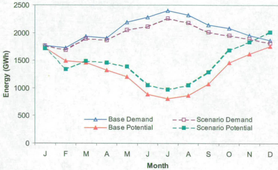
Figure 4.5: Mean monthly hydro potential energy production and consumption in New Zealand. (Scenario \Delta P + 20, \Delta T + 2^\circ\text{C} ) [99]
