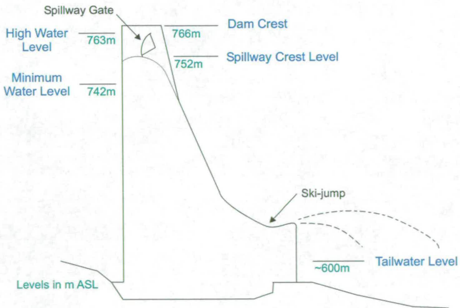
Figure 7.5: Spillway section schematic
