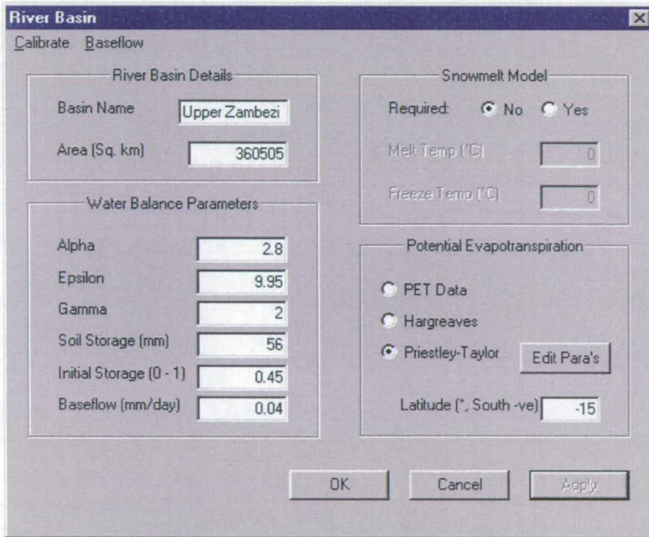
Figure 6.6: WatBal dialog
