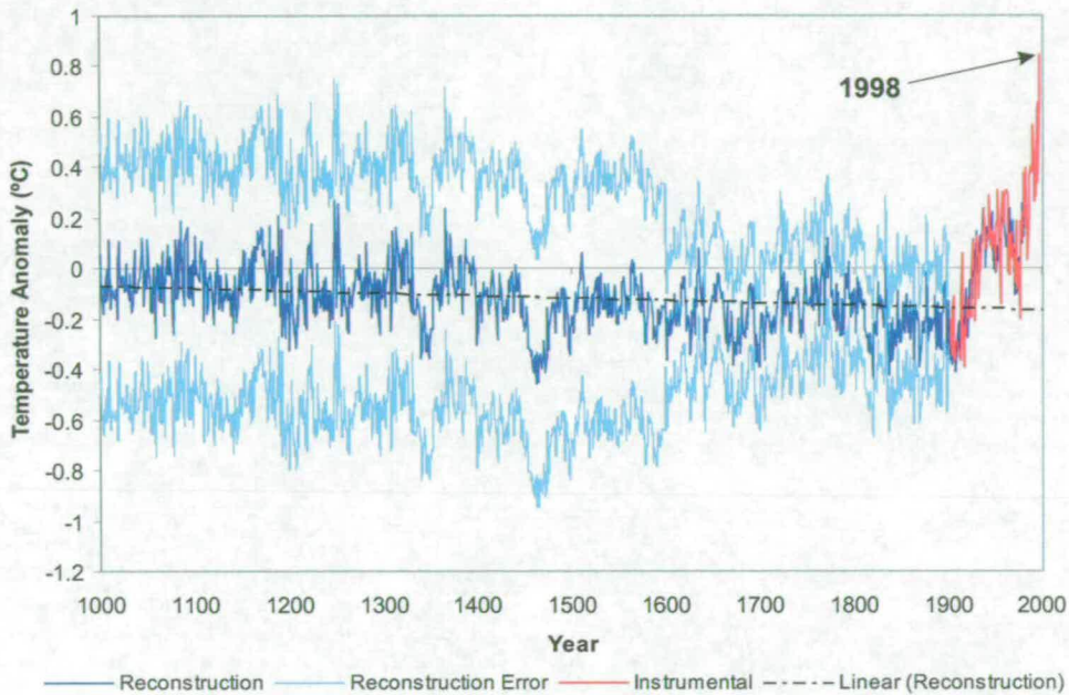
Figure 2.6: Northern Hemisphere temperature anomaly over last Millennium reconstructed from proxy sources (relative to 1902-1980 mean) [24]
