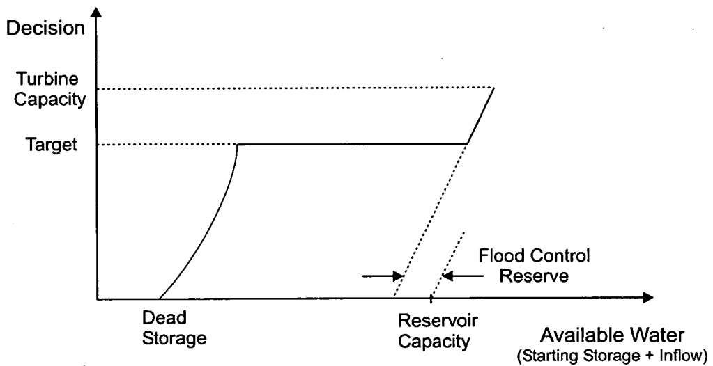
Figure 5.4: Standard reservoir operating rule [175]
