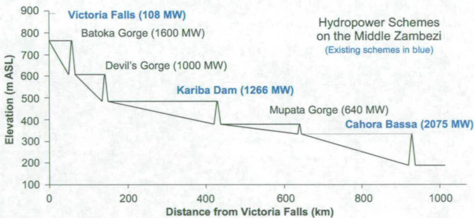
Figure 7.3: Hydroelectric facilities on the Middle Zambezi River [220]
