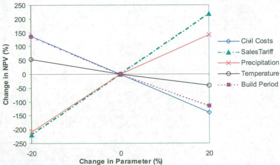
Figure 7.13: Sensitivity of project NPV to climate and project parameter changes (20% temperature change equivalent to 4°C)
