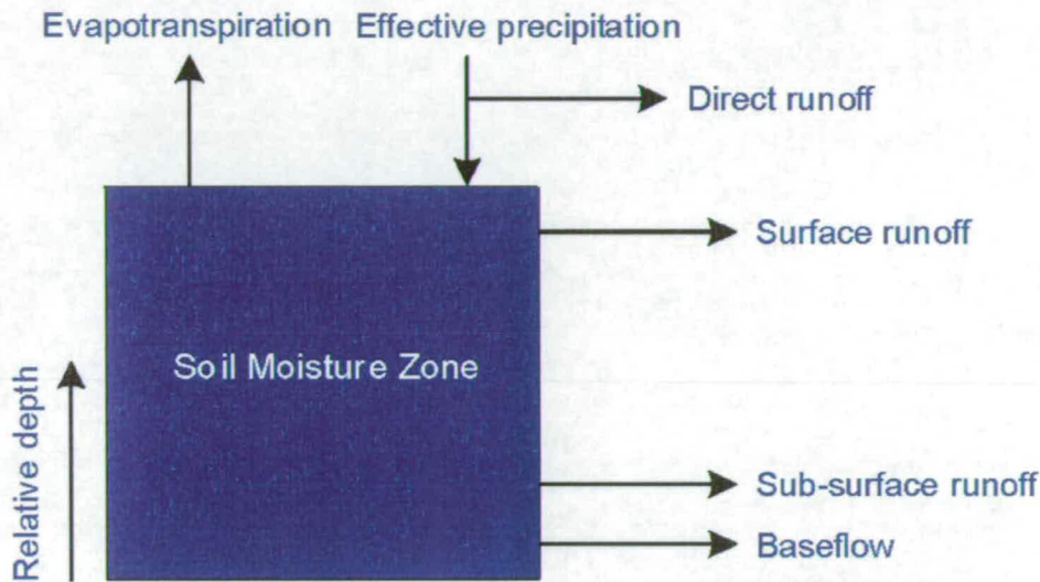
Figure 6.4: Conceptual structure of WatBal model [205]
