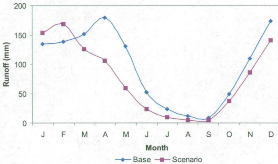
Figure 4.4: Monthly runoff in the Mesohora basin, Greece, for current and altered ( \Delta P = -10\% , \Delta T = 4^\circ\text{C} ) climates [117]
