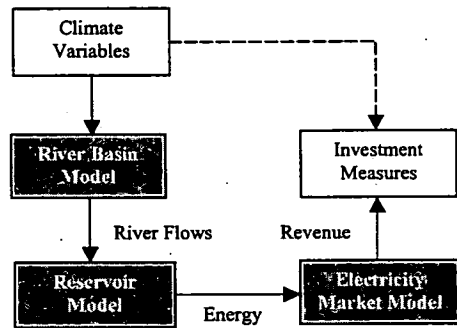
Figure 3. Software tool structure.
