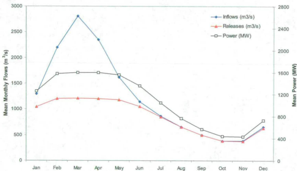
Figure 7.9: Monthly production, releases and river flows
