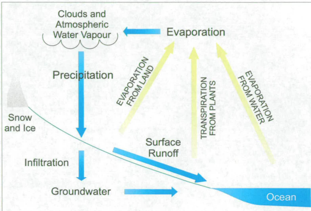
Figure 4.1: Climate and the hydrological cycle
