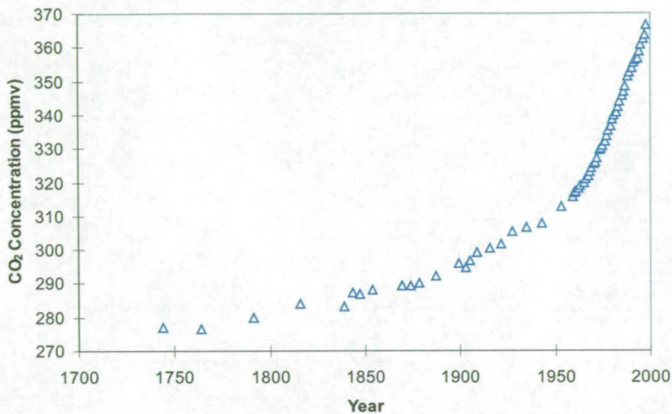
Figure 2.1: Atmospheric CO 2 increase over the past 250 years, indicated by air trapped in Antarctic ice (up to 1953) and by direct measurement at Mauna Loa, Hawaii from 1958 onwards [4, 5].
