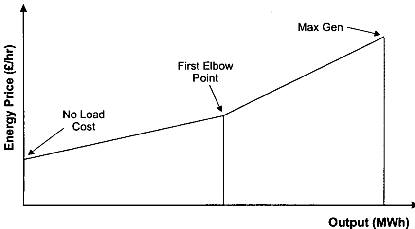
Figure 3.6: Thermal generation marginal cost curve, Willans' Line [73]
