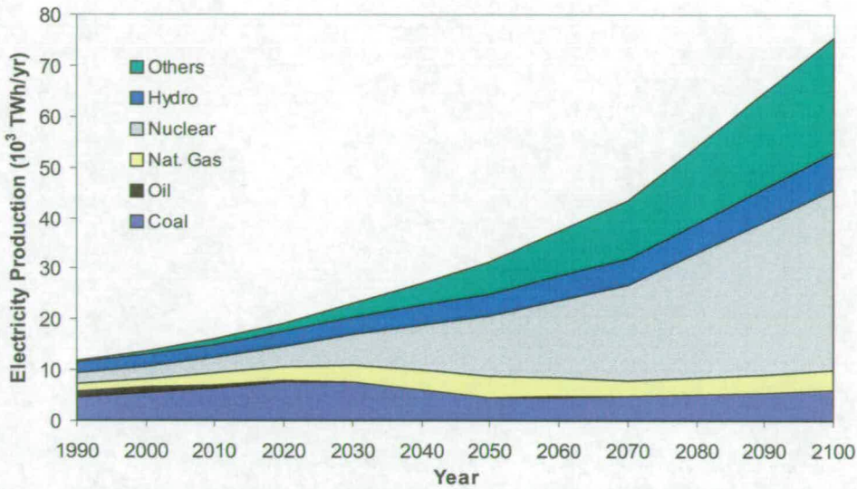
Figure 3.2: Middle course WEC/IIASA electricity supply scenario B [74]
