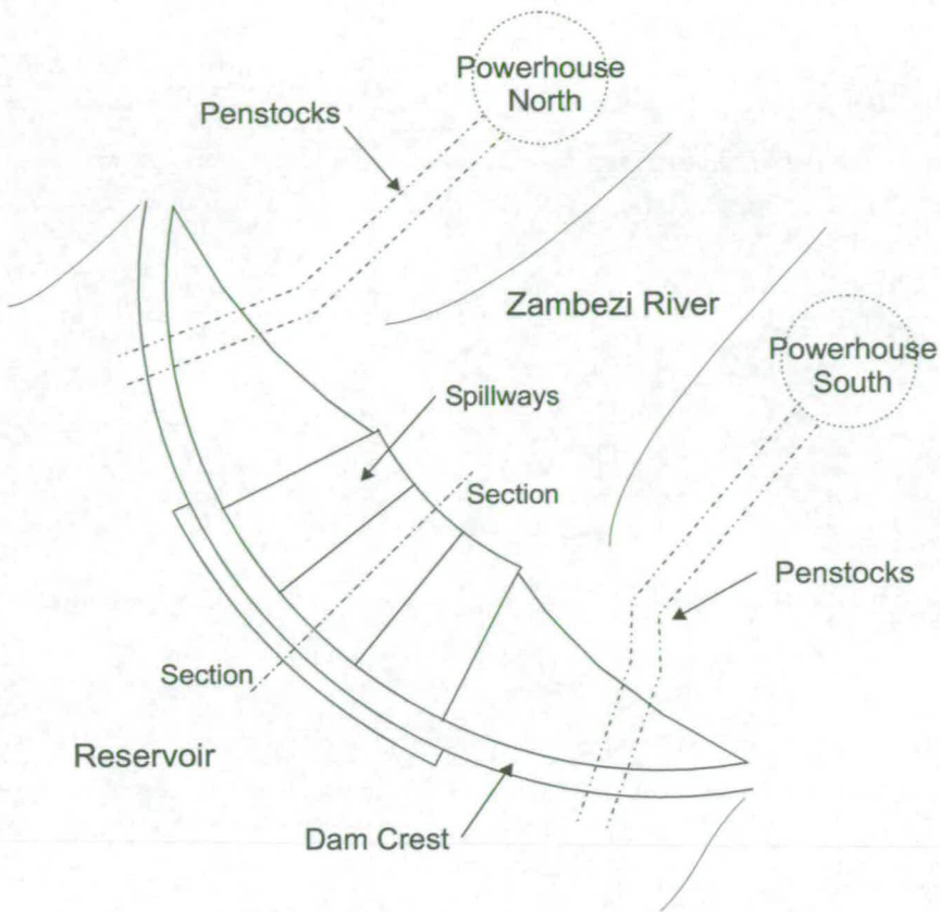
Figure 7.4: Schematic plan view of Batoka Scheme
