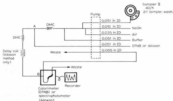
Fig. 1. The flow-diagrams for the automated DTNB and alloxan GSH methods. Both systems employ standard Technicon AutoAnalyser equipment except for the Unicam SP1800 spectrophotometer and AR25 recorder used with the alloxan manifold. The inclusion of a delay coil in the alloxan manifold is the only other difference between the two systems. The reagents for both methods are described in the text.
