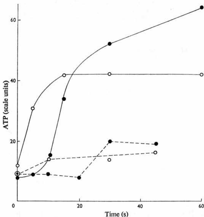
Fig. 2. ATP synthesis in rat liver mitochondrial suspensions preincubated anaerobically for 3 min or 20 min at 30°C with or without the addition of D_{Na}
