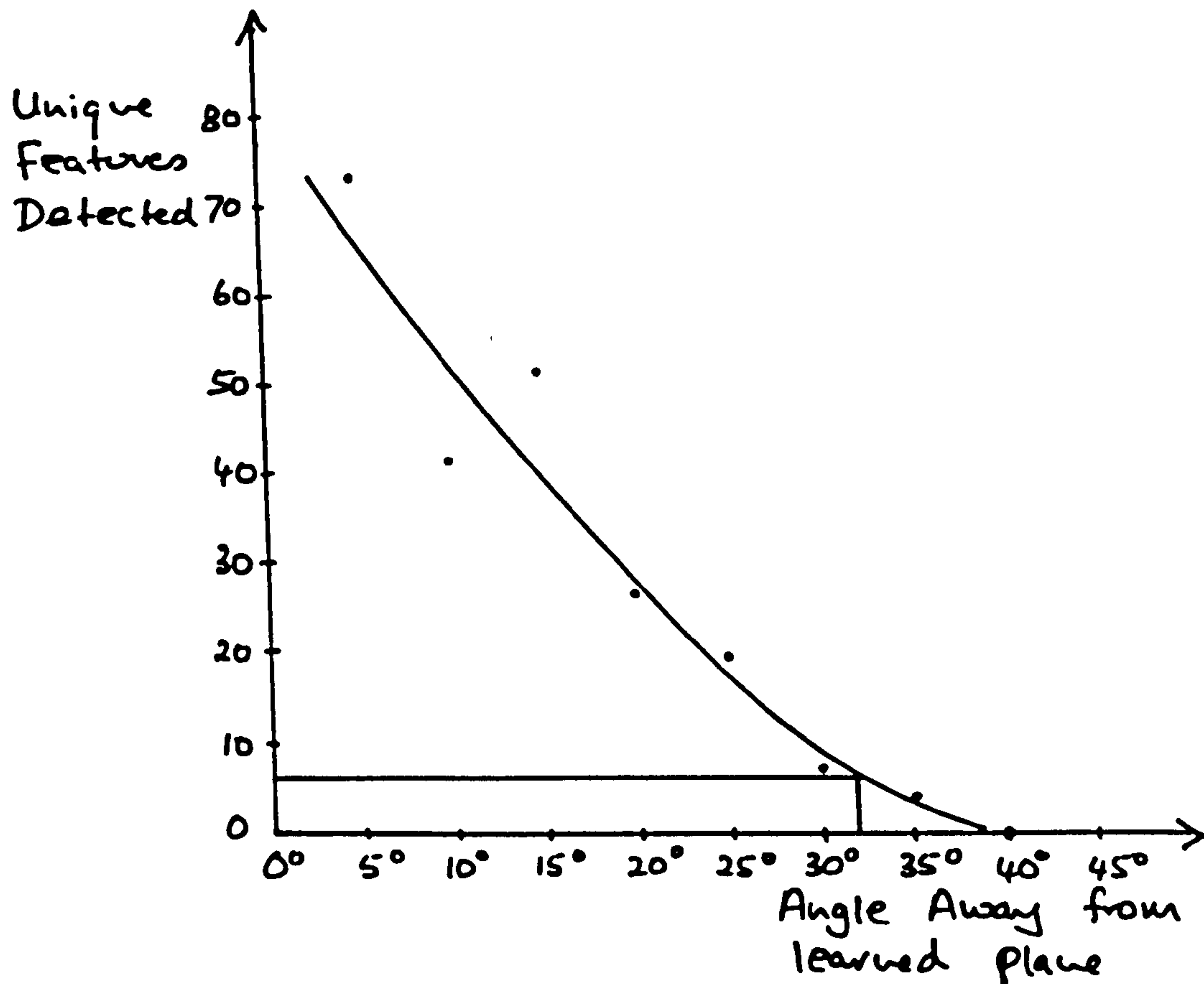
Fig. 5-12 Unique features detected for the cutter with orientation variation learned plane ( 47^\circ for the tooth wheel). Fig. 5-13 shows the cutter on the inclined plane at the threshold of recognition. From the following statistics it will be noticed that the number of spurious features were very high on this test. (But note the lack of spurious features when the tooth wheel was in the image). This demonstrates the need to extend the reliability check to these situations if the system is required to operate with such images.
