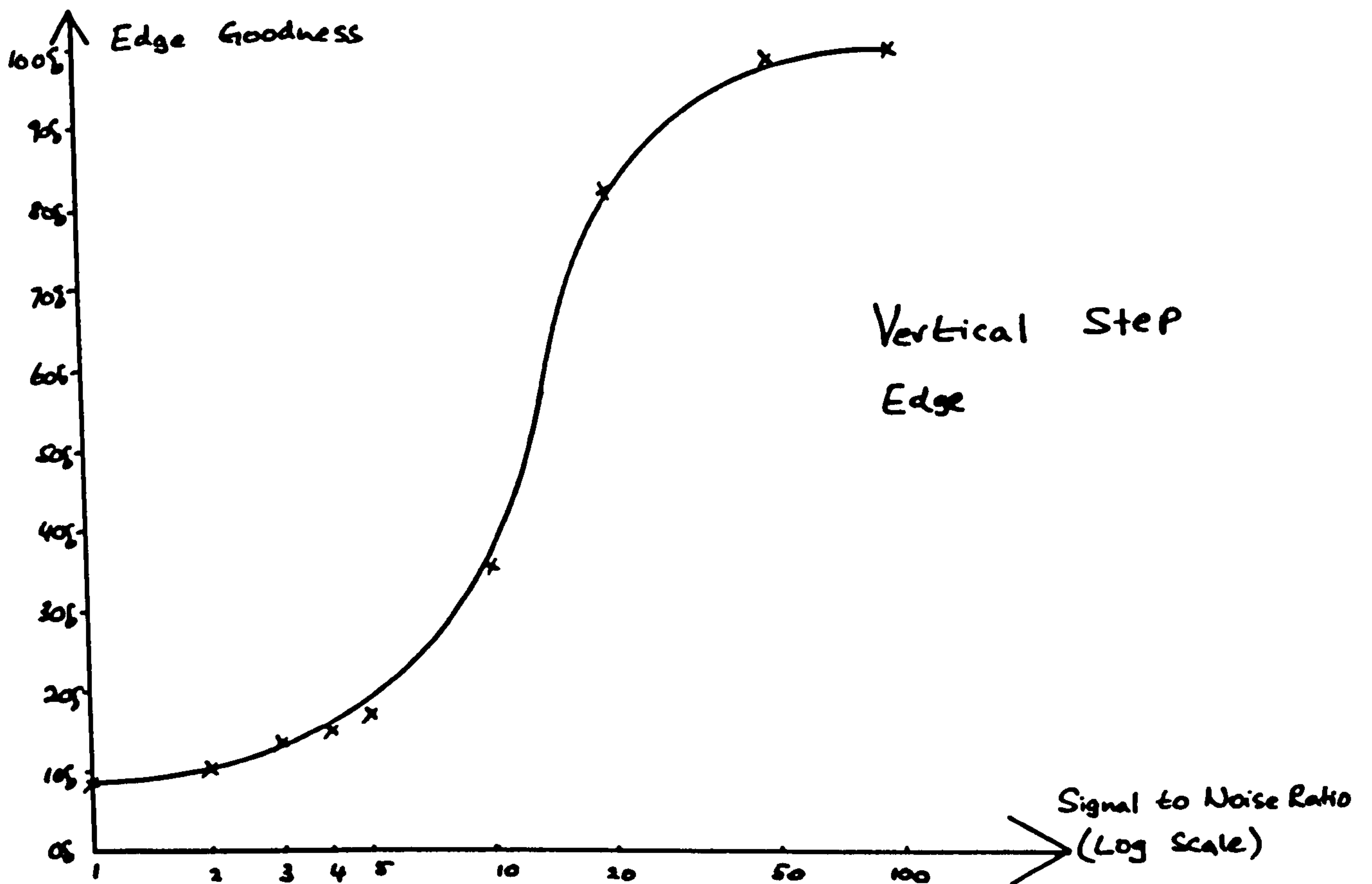
Fig. 5-36 Variation of Pratt goodness measure with added noise
