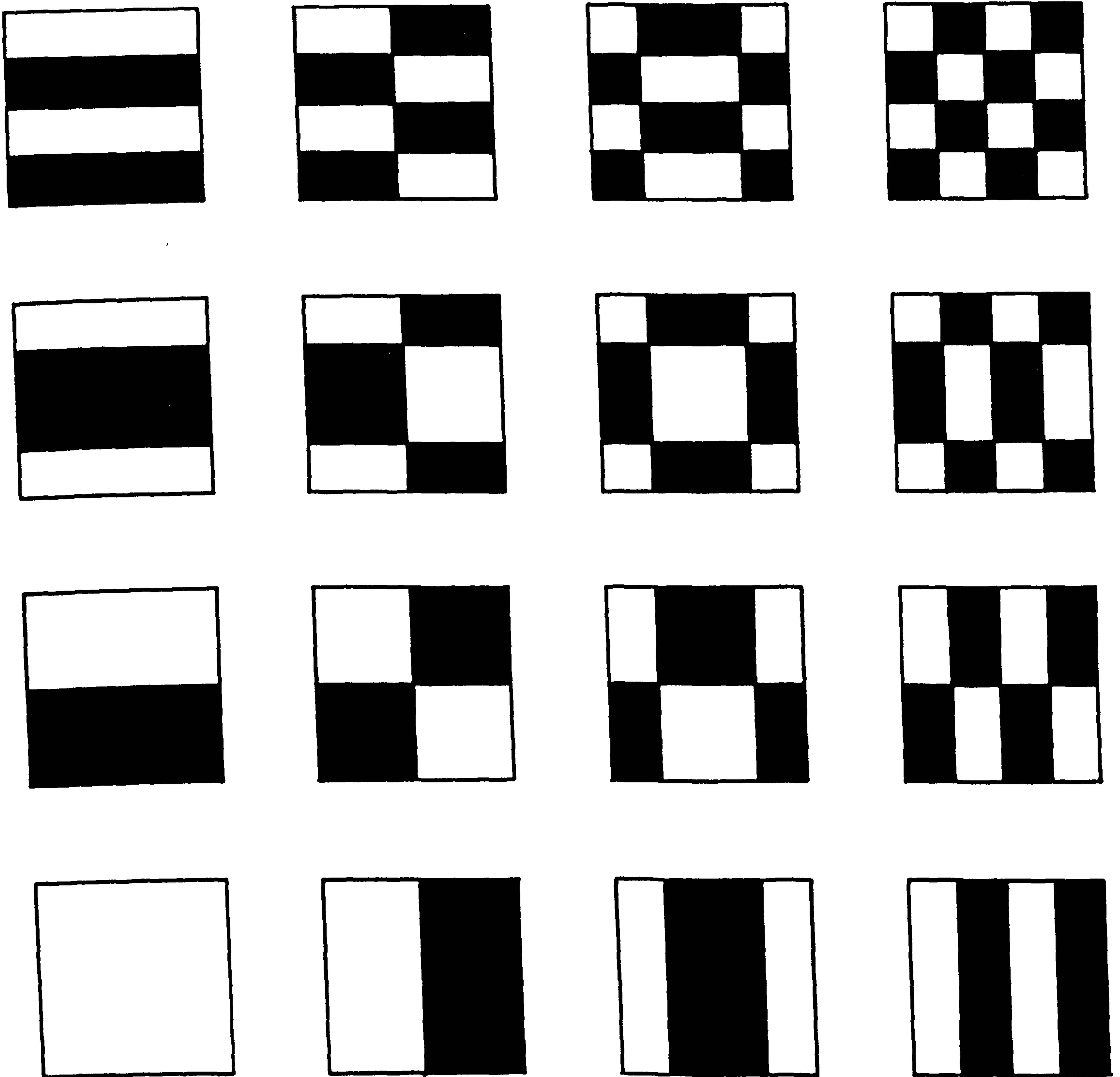
Fig. 4-3 The first 16 Walsh functions in 2D (Black=-1, White=+1)
