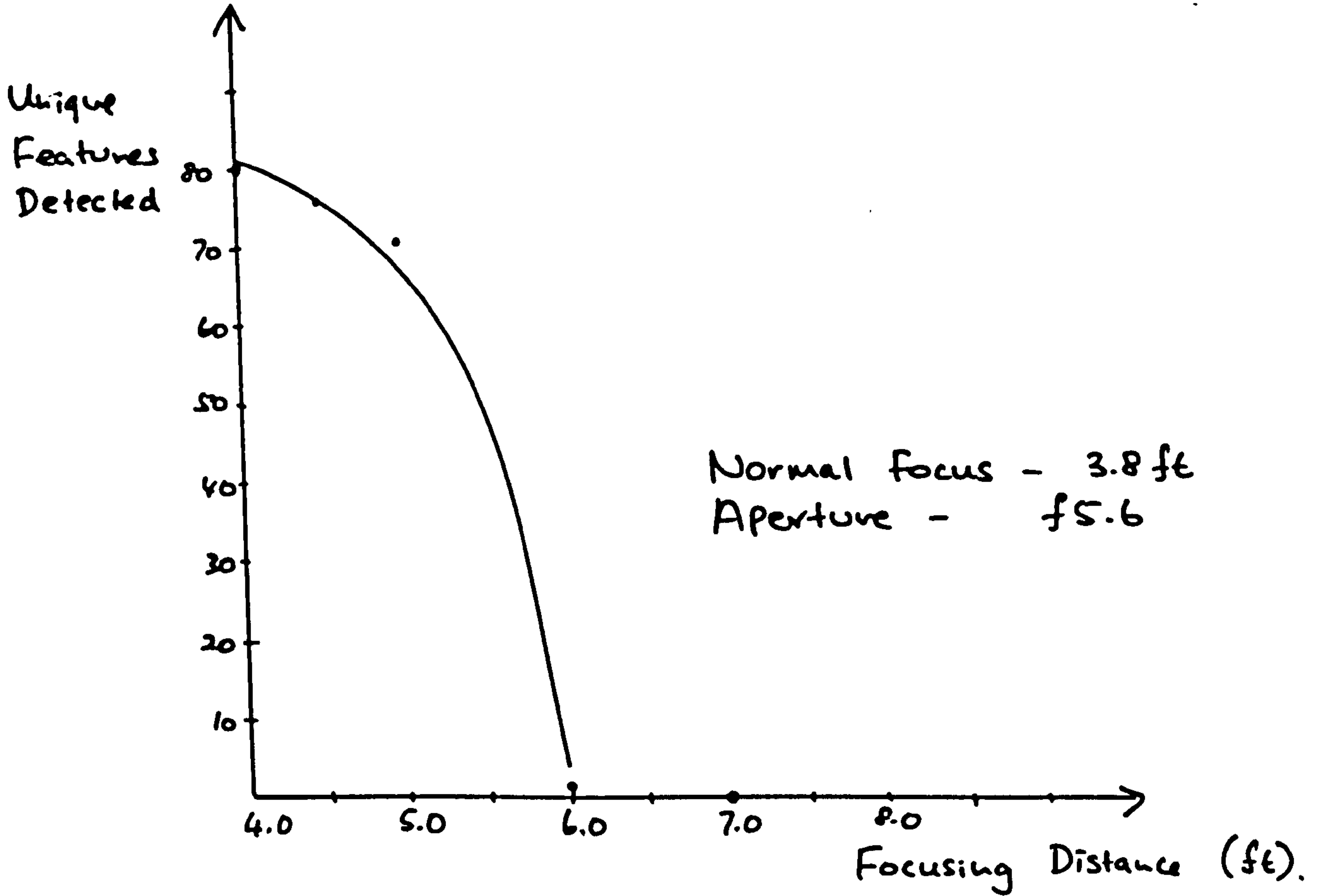
Fig. 5-14 Unique features detected for the tooth-wheel with defocussing
