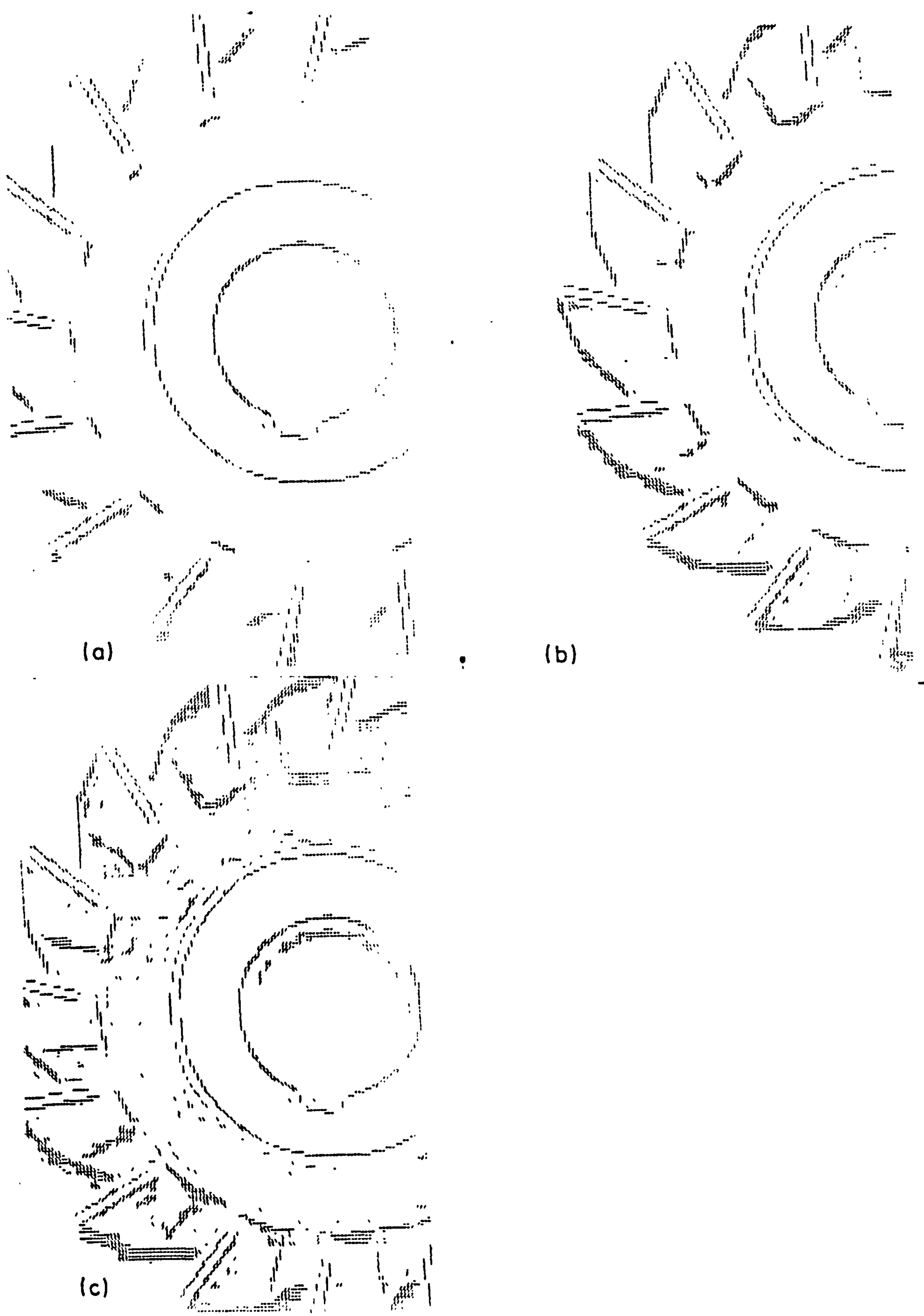
Fig. 5-29 Variation of edge image with d threshold
