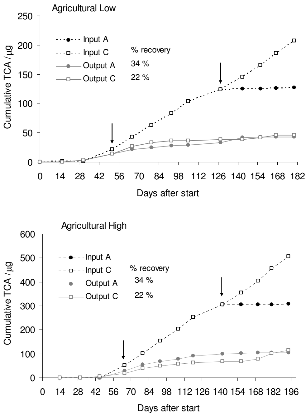
Figure S2. Cumulative TCA inputs and outputs to lysimeters from an agricultural site near Edinburgh, dosed two-weekly with 20 \mu\text{g} TCA (Low) or 50 \mu\text{g} TCA (High) over a 6-month period (Jan – June 2002). On each site visit the leachate present was collected before the lysimeter was dosed. The input data is the sum of rainwater plus dosing input up to that point. The first arrow in each graph indicates the first TCA dosing and the second arrow indicates the final dosing for lysimeter A. The final % recoveries of input TCA in the leachate are shown in the legend.
