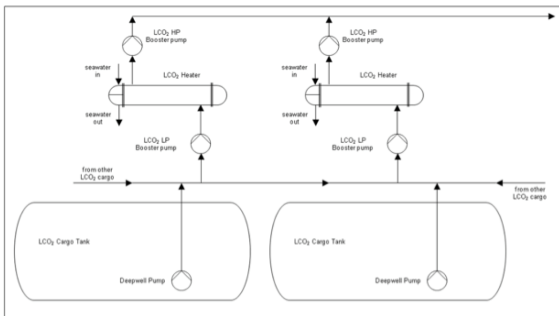
Figure 8. Proposed discharge equipment on ship (Vermeulen, 2011)
