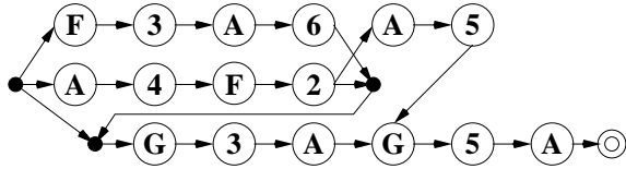
Figure 6. Example of a substroke network for three Kanji characters: “右 (incorrect stroke-order) (A4F2G3AG5A)”, “右 (F3A6G3AG5A)”, “左 (A4F2A5G5A)”, “口 (G3AG5A)”.
