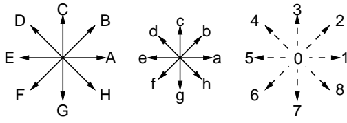
Figure 1. Substroke categories: A–H (a–h) are long (short) substrokes with pen-down and 0–8 are directions of pen-up movement.
