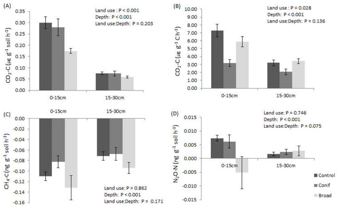
Figure 2.2 Potential fluxes of (A) \text{CO}_2 ( \mu\text{g g}^{-1} \text{ soil hr}^{-1} ), (B) \text{CO}_2 ( \mu\text{g g}^{-1} \text{ C hr}^{-1} ), (C) \text{CH}_4 ( \text{ng g}^{-1} \text{ soil hr}^{-1} ), and (D) \text{N}_2\text{O} ( \text{ng g}^{-1} \text{ soil hr}^{-1} ) from soils under different land uses (control, coniferous and broadleaved) and different depths. Fluxes in (A), (C) and (D) are based on soil dry weight. Note scales are not consistent; error bars represent standard error.
