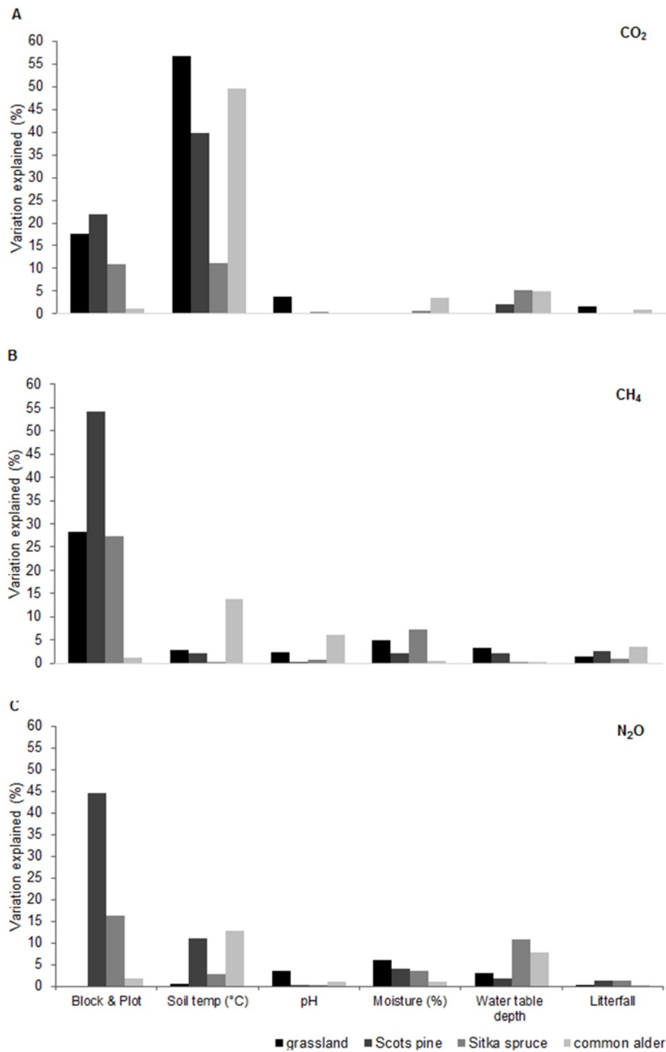
Figure 3.5. Percentage variation (as determined by linear mixed models) in soil GHG fluxes as explained by measured variables in each habitat. (A) net CO 2 flux, (B) CH 4 flux, and (C) N 2 O flux. Block & Plot were random factors in the model. Values for residuals have been omitted from these plots.
