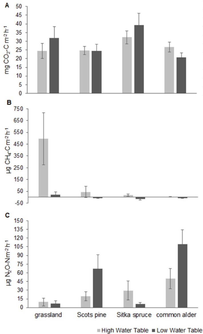
Figure 4.1. Soil GHG fluxes for all habitats. (A) CO 2 , (B) CH 4 , (C) N 2 O, at high (3 cm below surface) and low water table (27 cm below surface) depths. Error bars represent standard error. n= 3 for Grassland mesocosms; n = 9 for tree species mesocosms.
