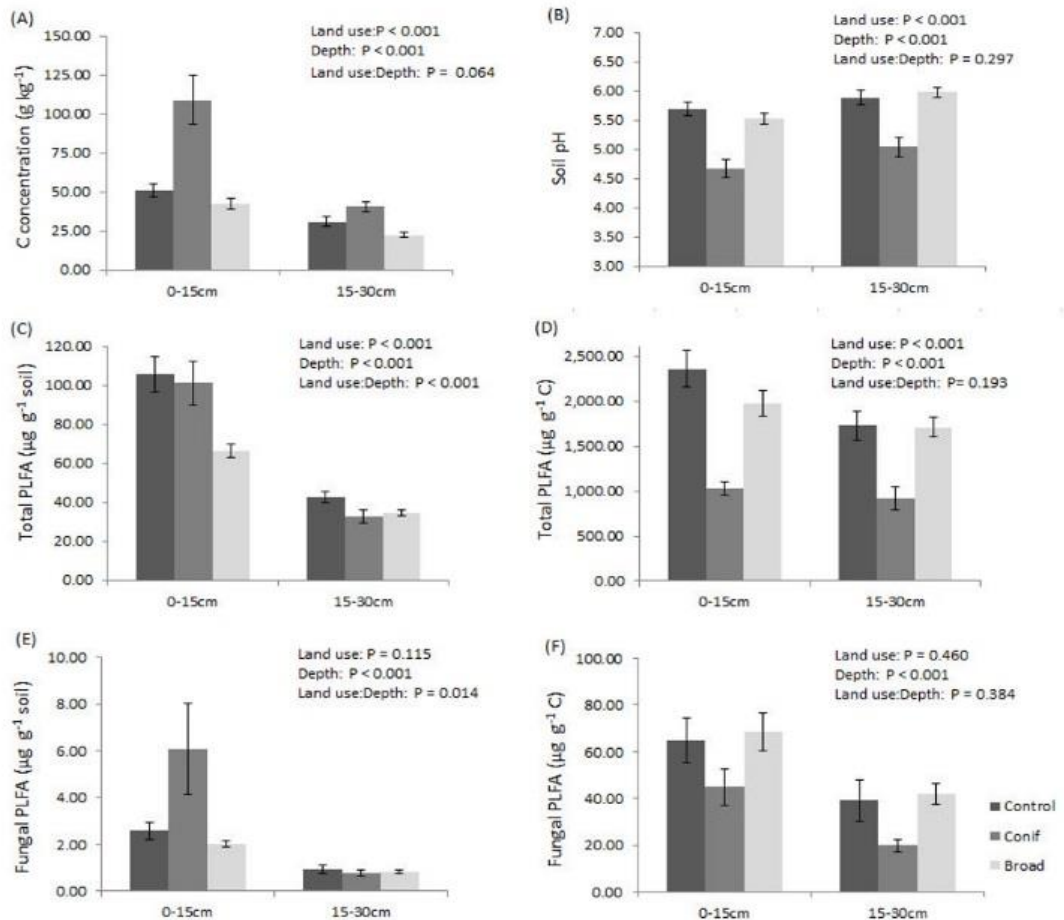
Figure 2.1 Measured (A) Soil carbon concentration (g kg -1 ), (B) Soil pH, (C) Total PLFA (μg g -1 soil), (D) Total PLFA (μg g -1 C), (E) Fungal PLFA (μg g -1 soil) and (F) Fungal PLFA (μg g -1 C) from soils under different land uses (control, broadleaved and coniferous) and different depths. Data in (C) and (E) are based on soil dry weight. Note scales are not consistent; error bars represent standard error.
