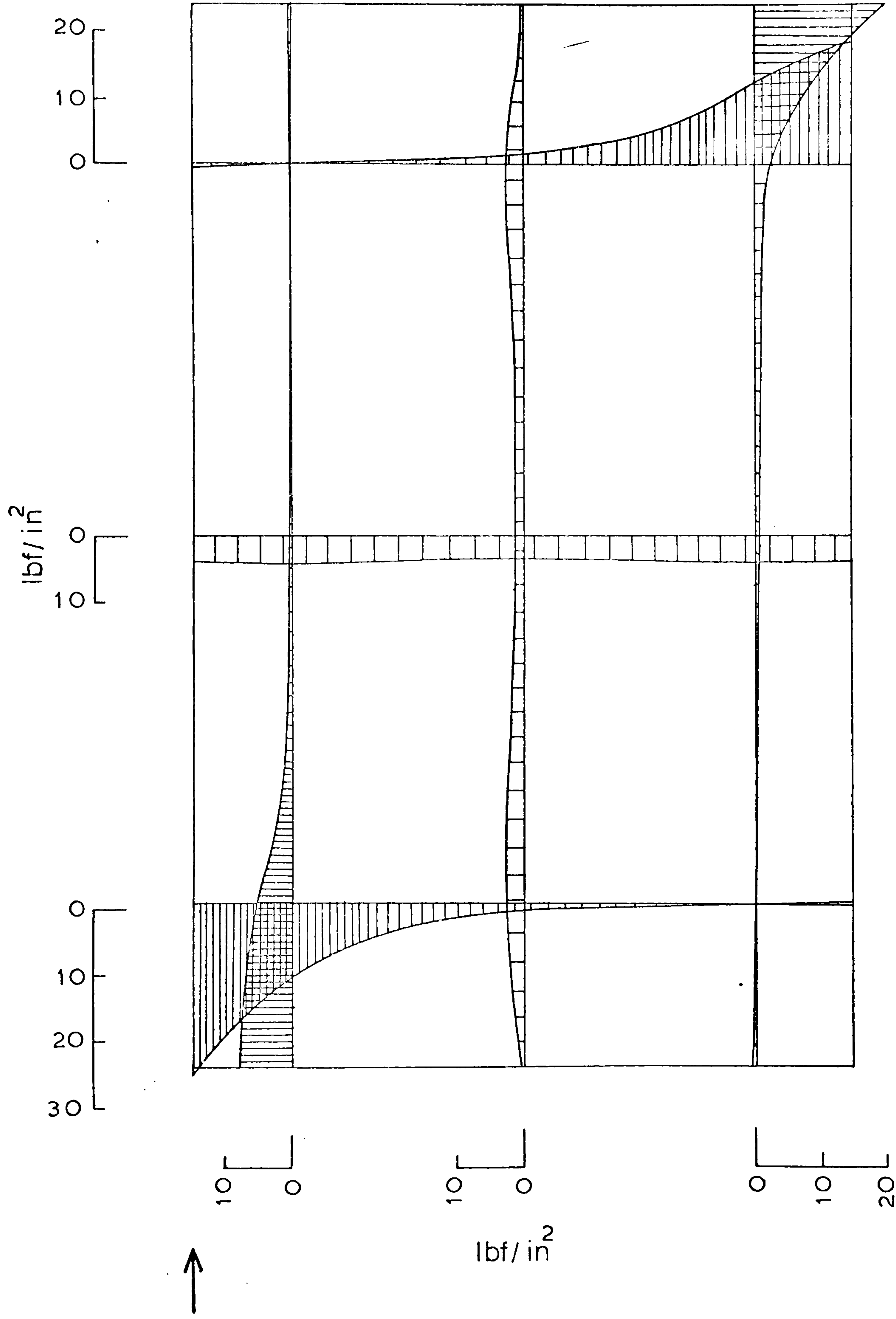
Fig.(4.18) Normal stress distribution , rect.1:16 (0.75in)
