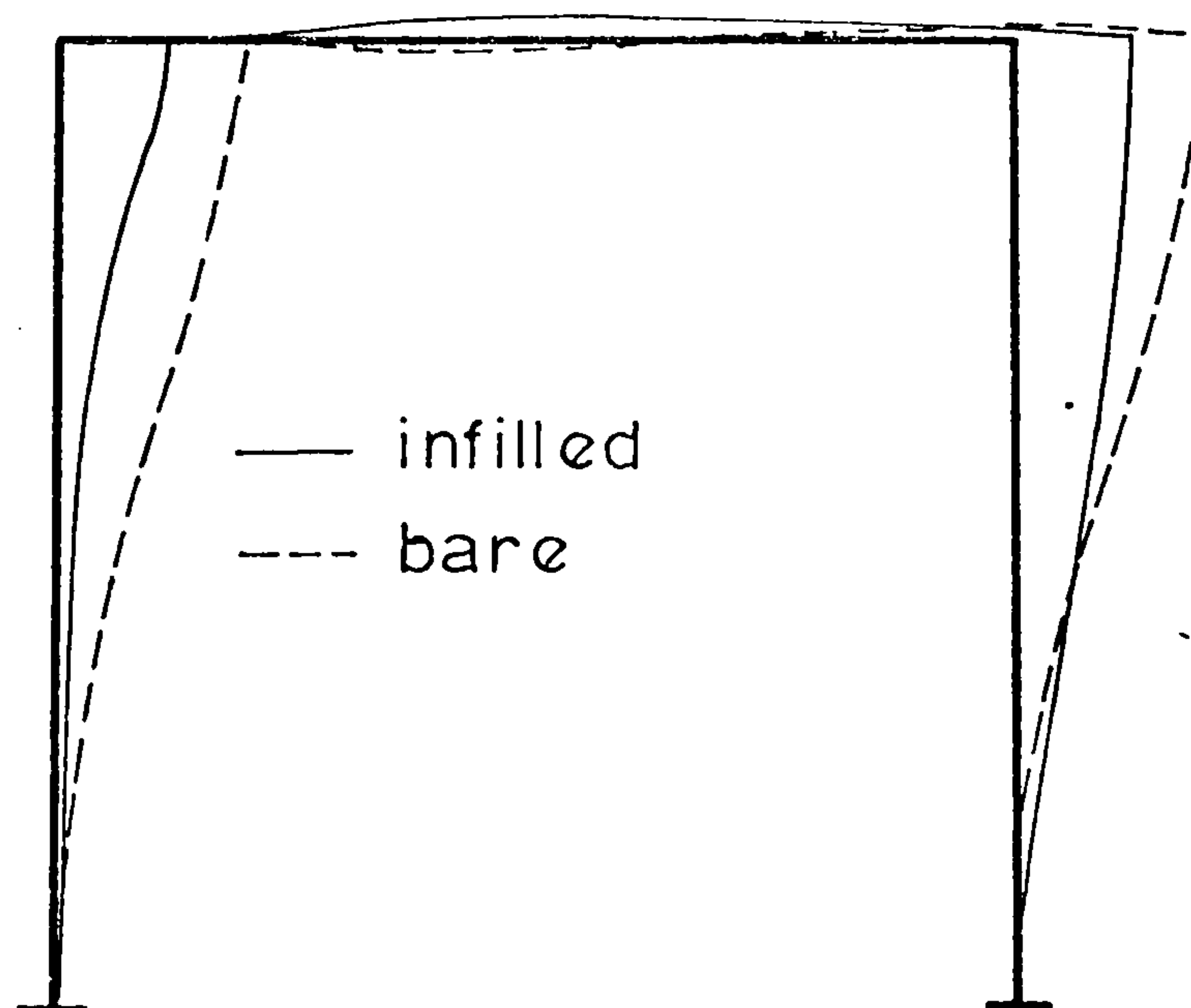
Fig.(4.15) Deflection shape of bare & infilled frame
