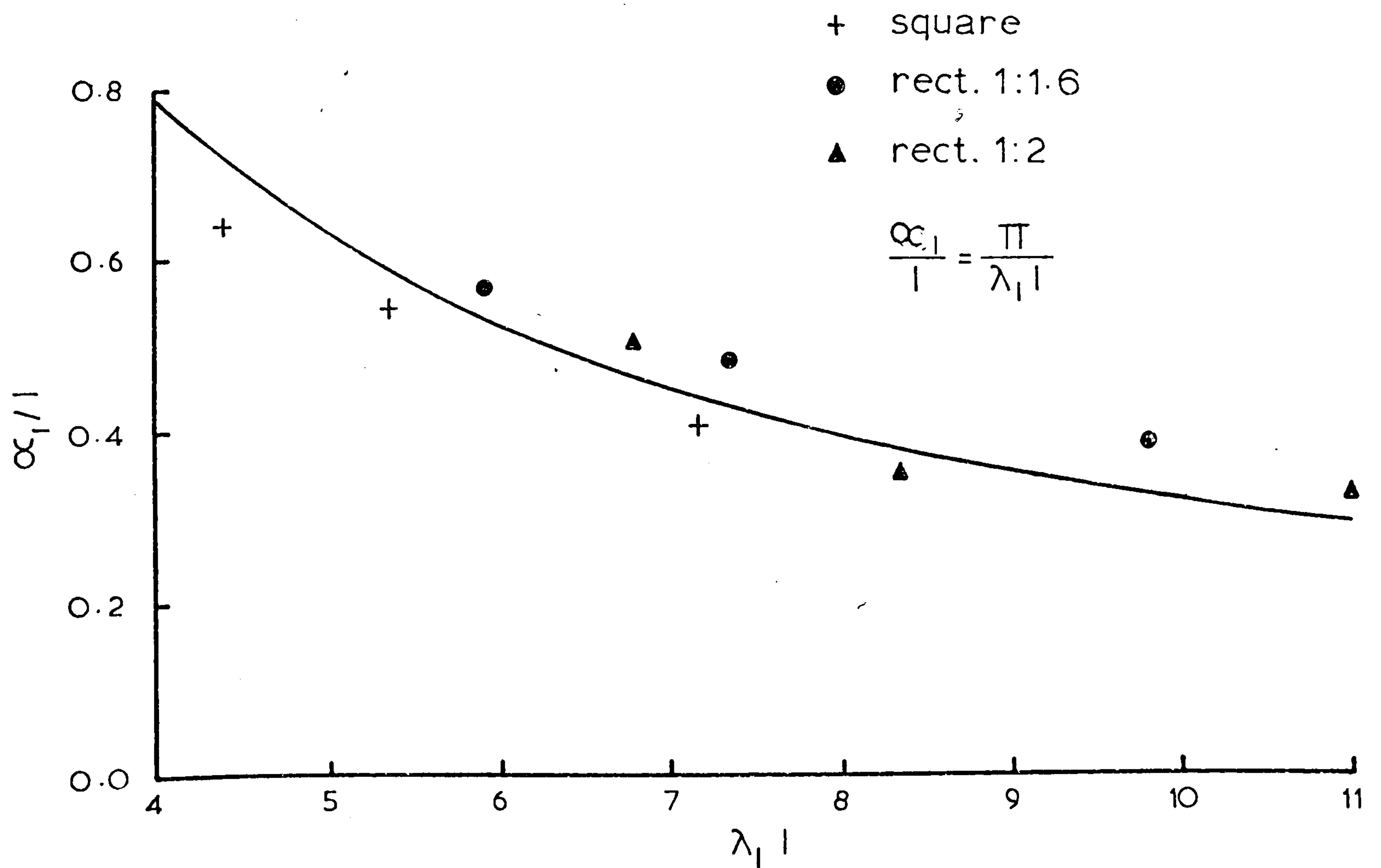
Fig.(4.4) \alpha_l as function of \lambda_l l
