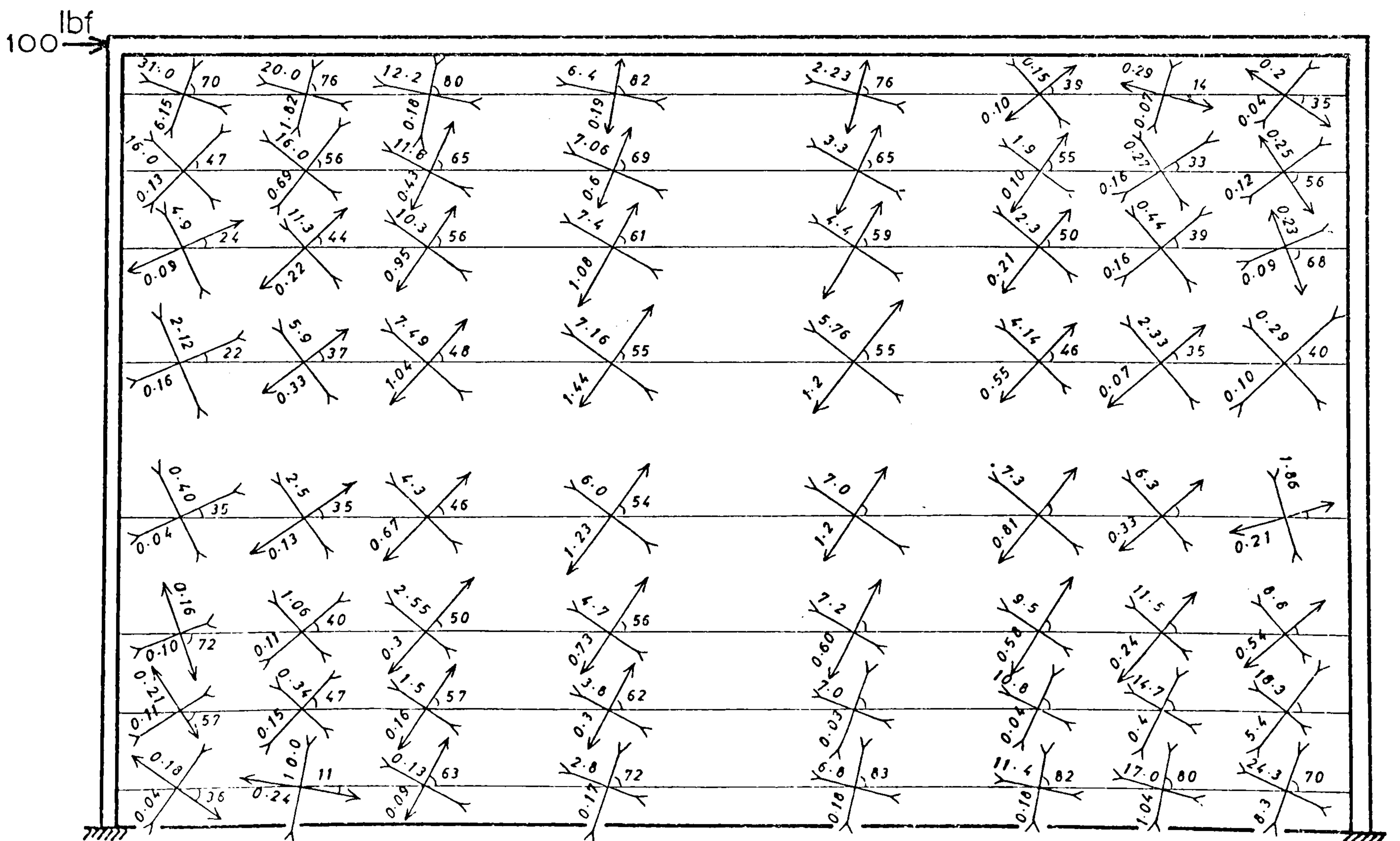
Fig. (4.23) Principle stresses (WT2)
