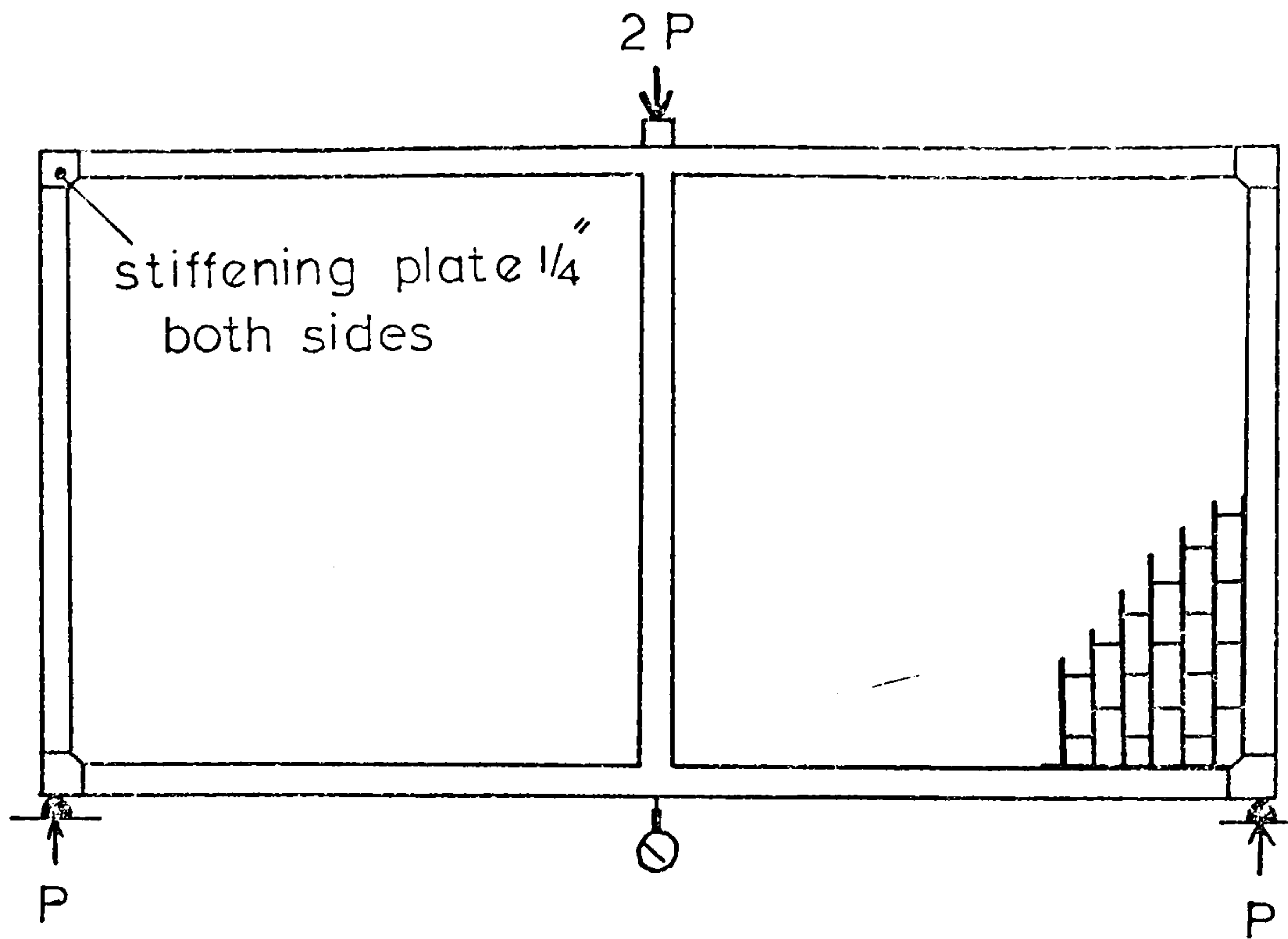
Fig.(3.2) Testing method.
