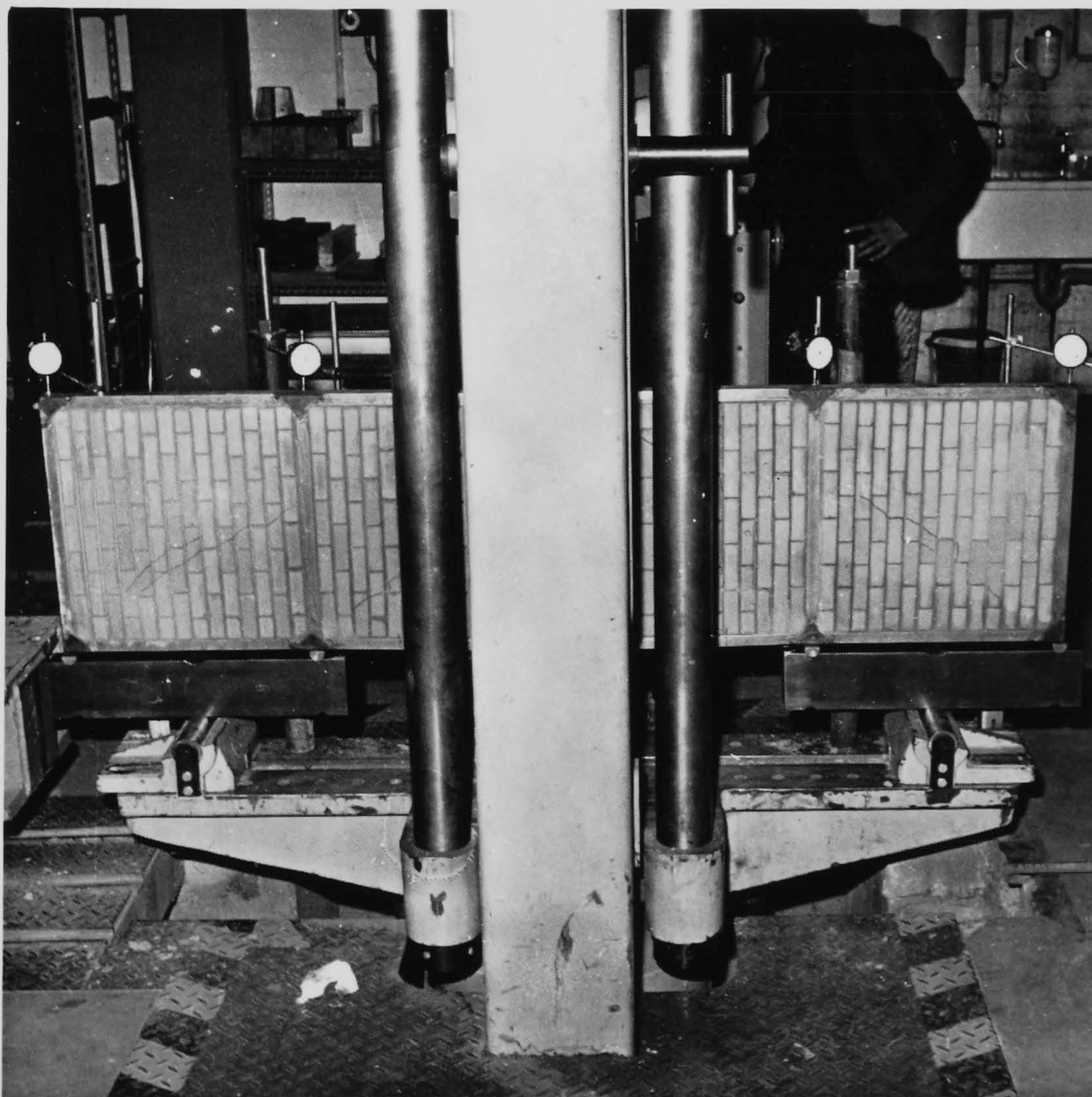
PLATE 7 TESTING ARRANGEMENT FOR THE TWO-STOREY PANELS
