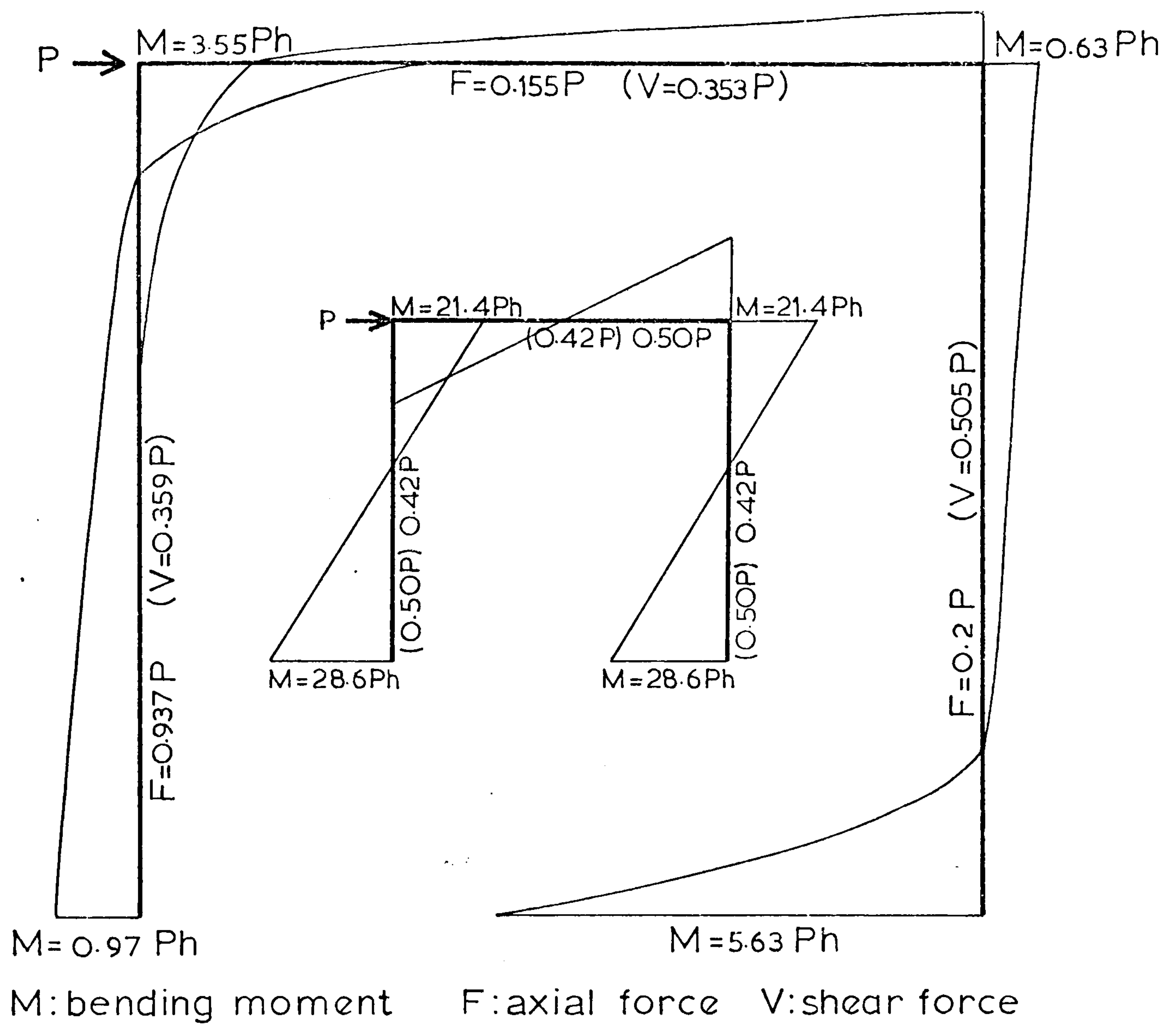
Fig.(4.14) Typical bare & infilled frame forces (WS2)
