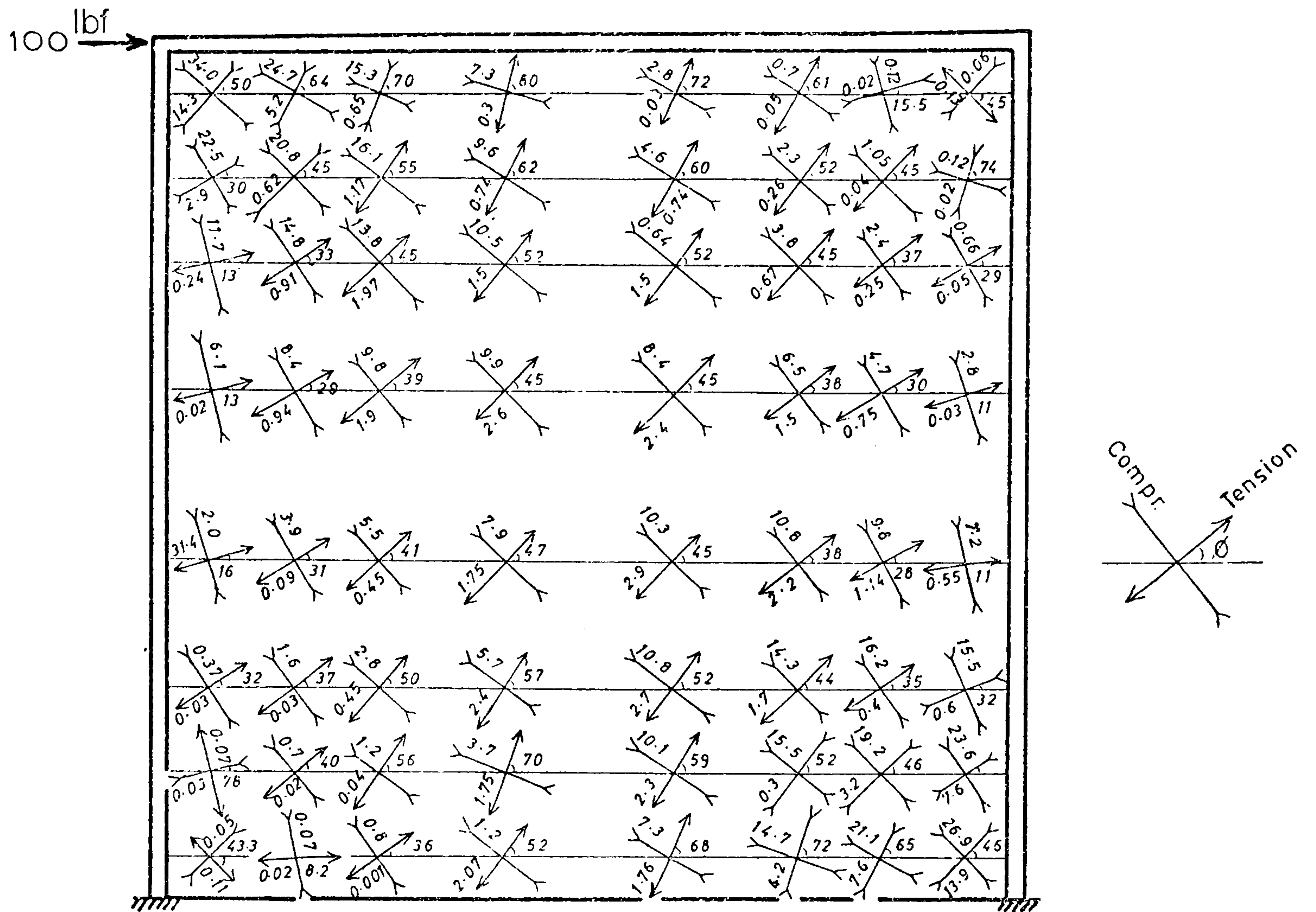
Fig. (4.22) Principle stresses (WS2)
