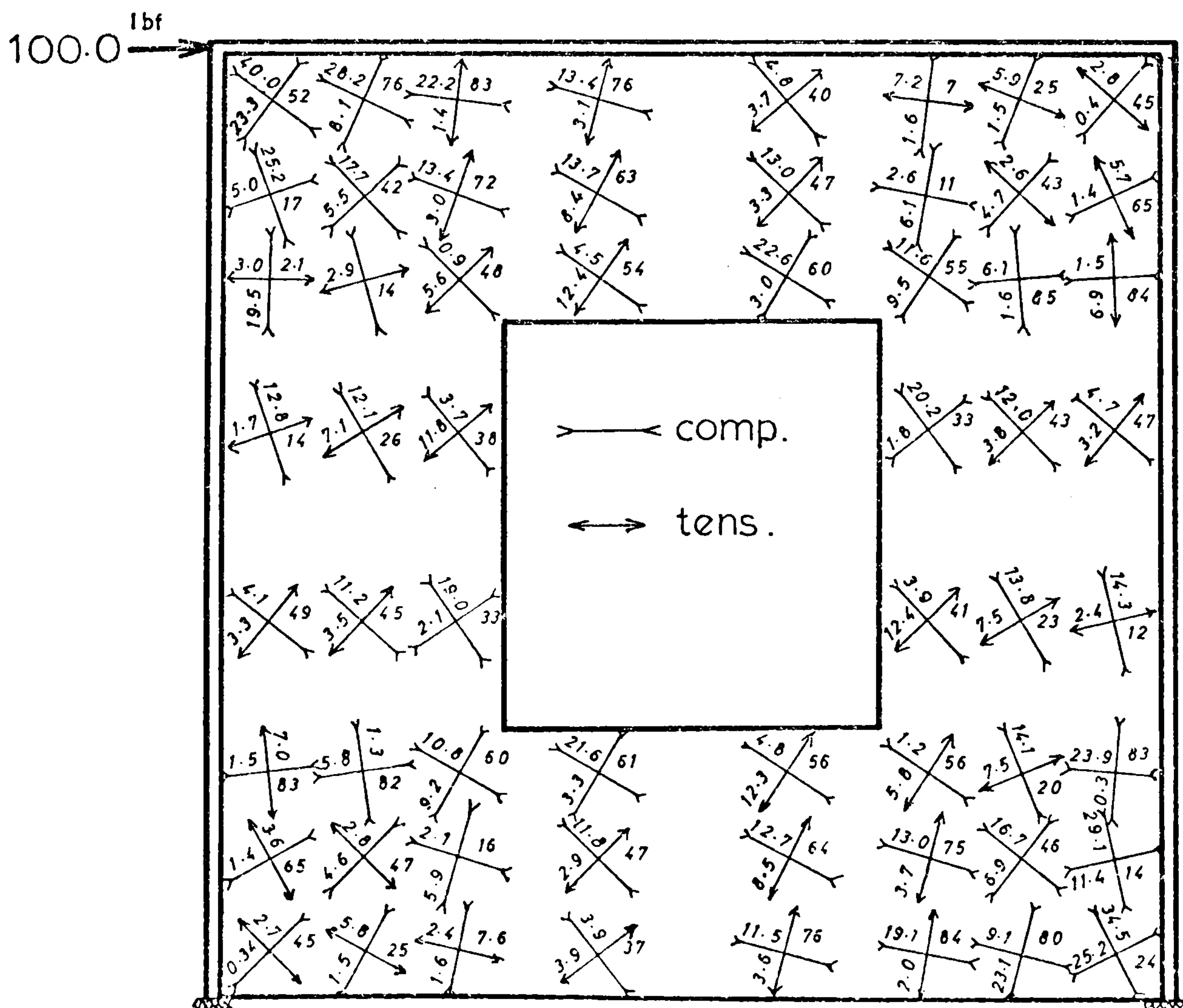
Fig. (5.6) Maximam principle stresses (WW1)
