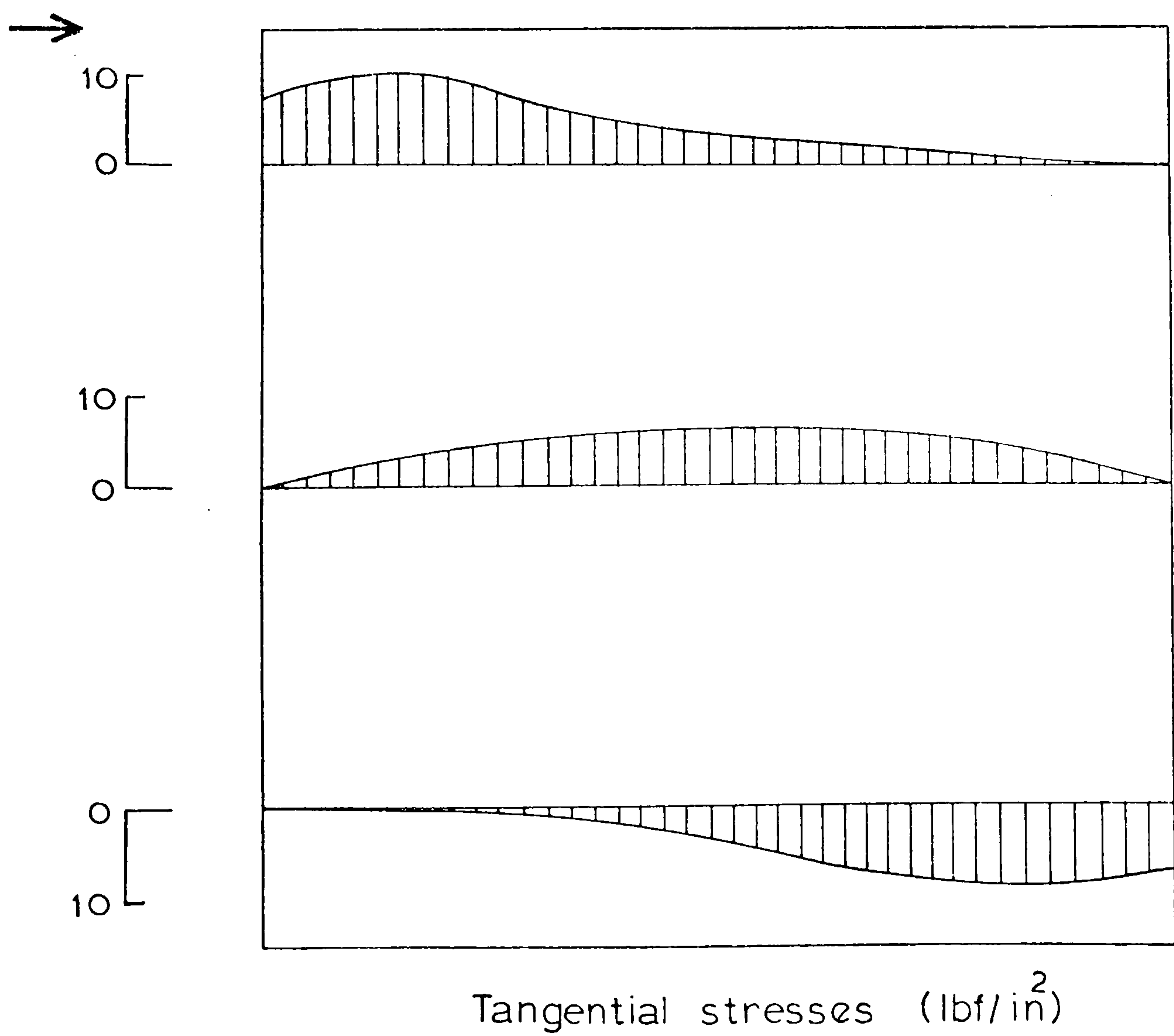
Fig.(4.17) Stress distribution, square (0.75 in)
