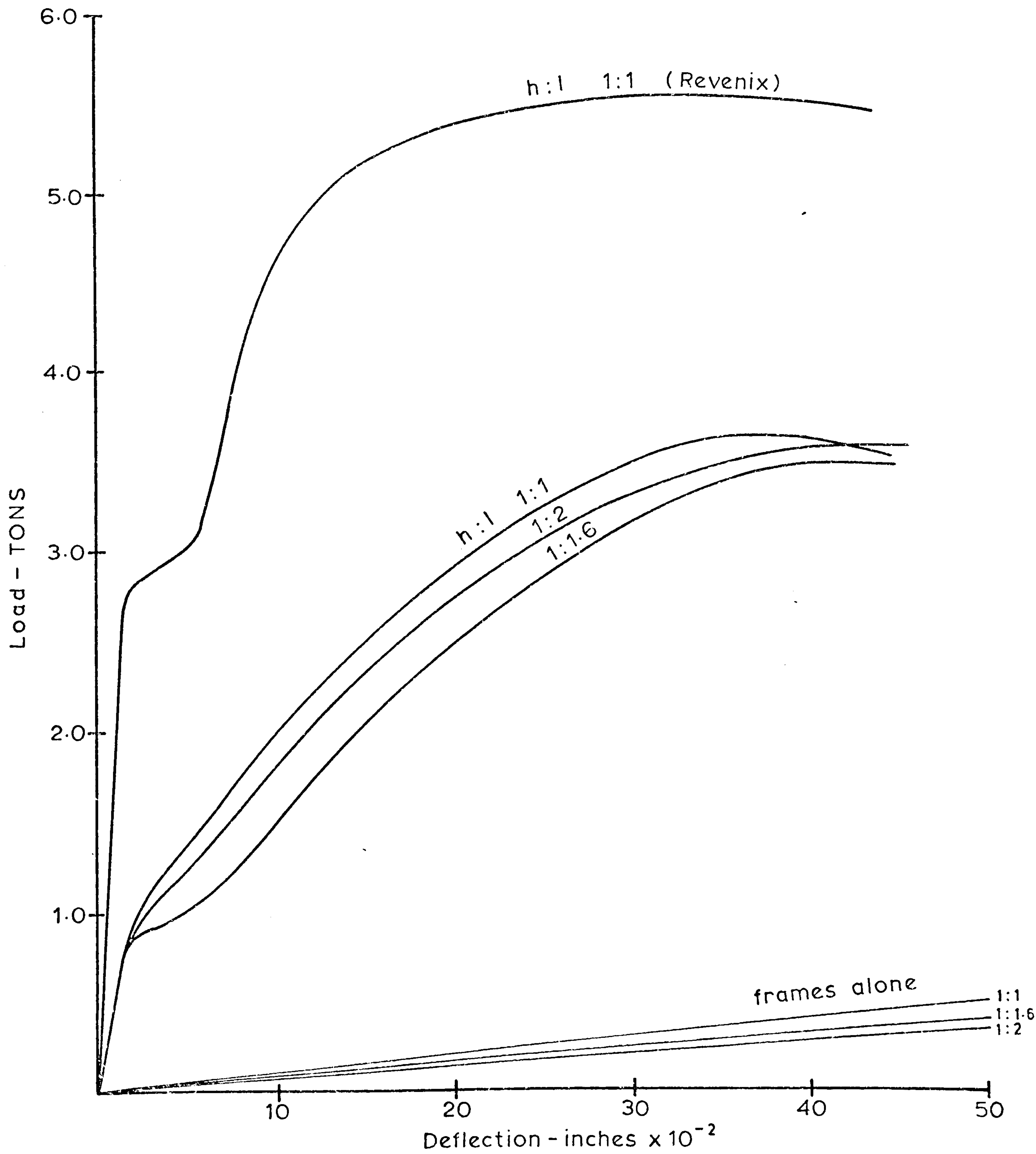
Fig.(3.6) Load- deflection curves (frame:0.5 in.)
