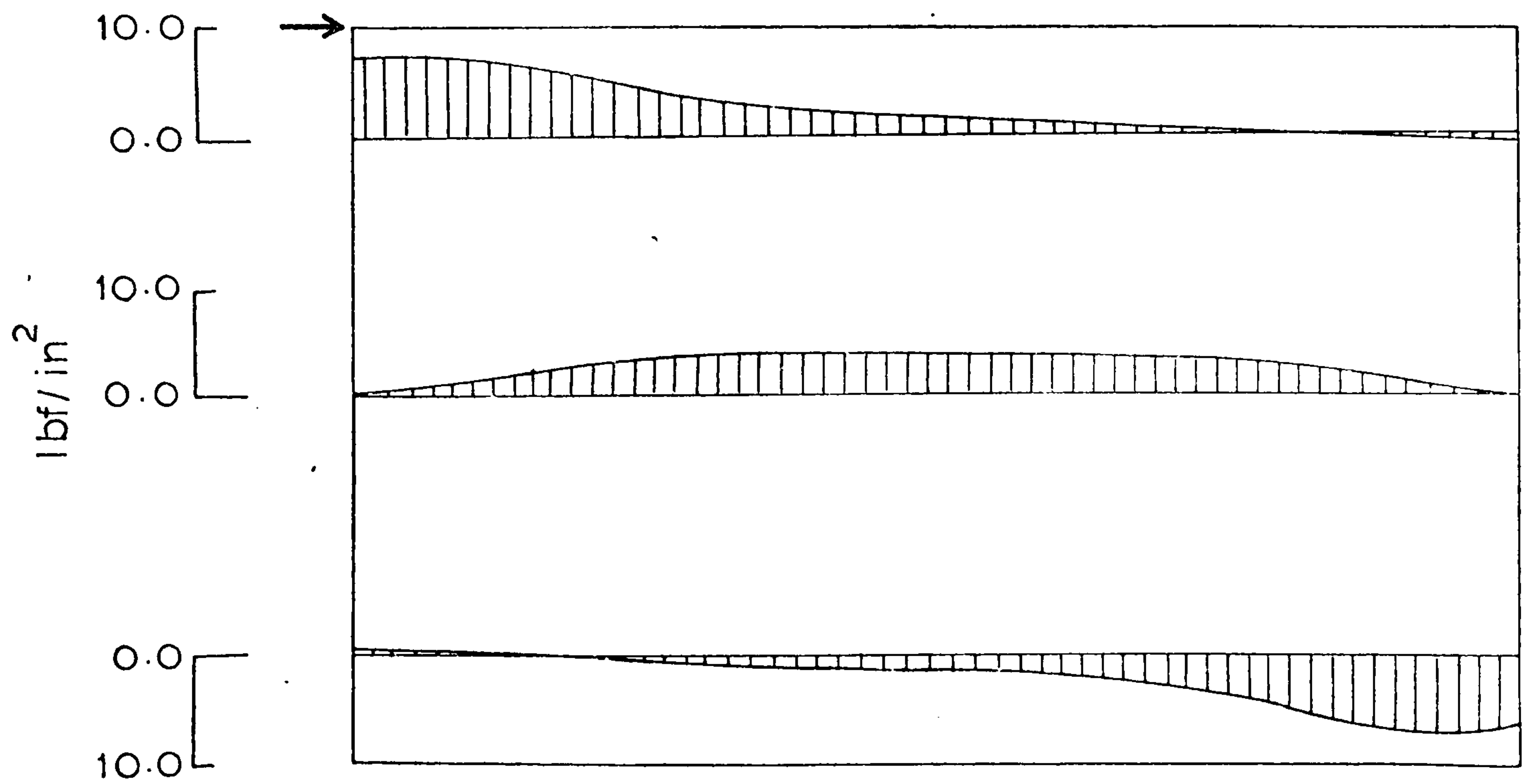
Fig.(4.21) Tangential stress distribution rect.1:1.6 (0.75 in)
