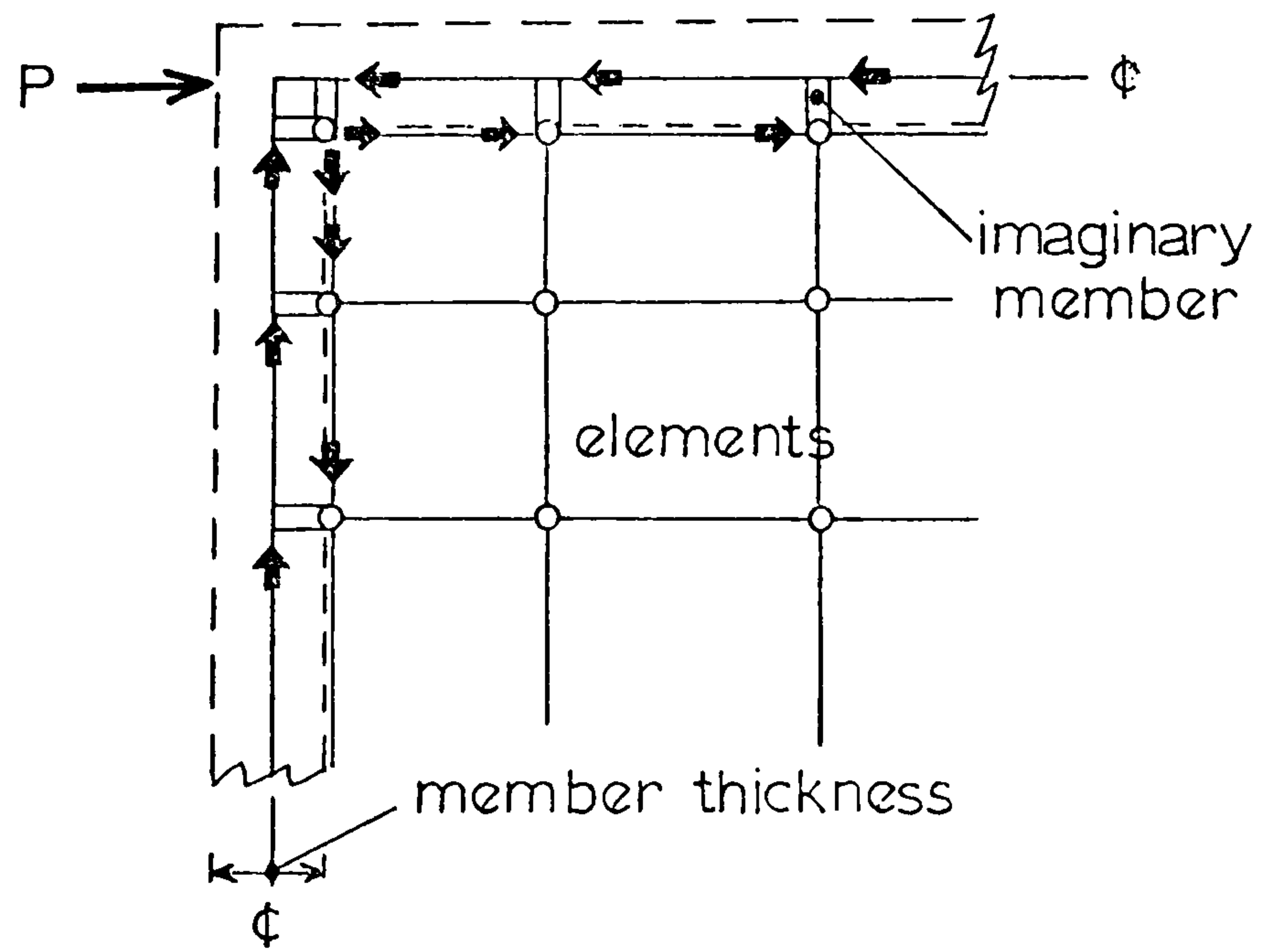
Fig.(4.13) Friction forces at the interface
