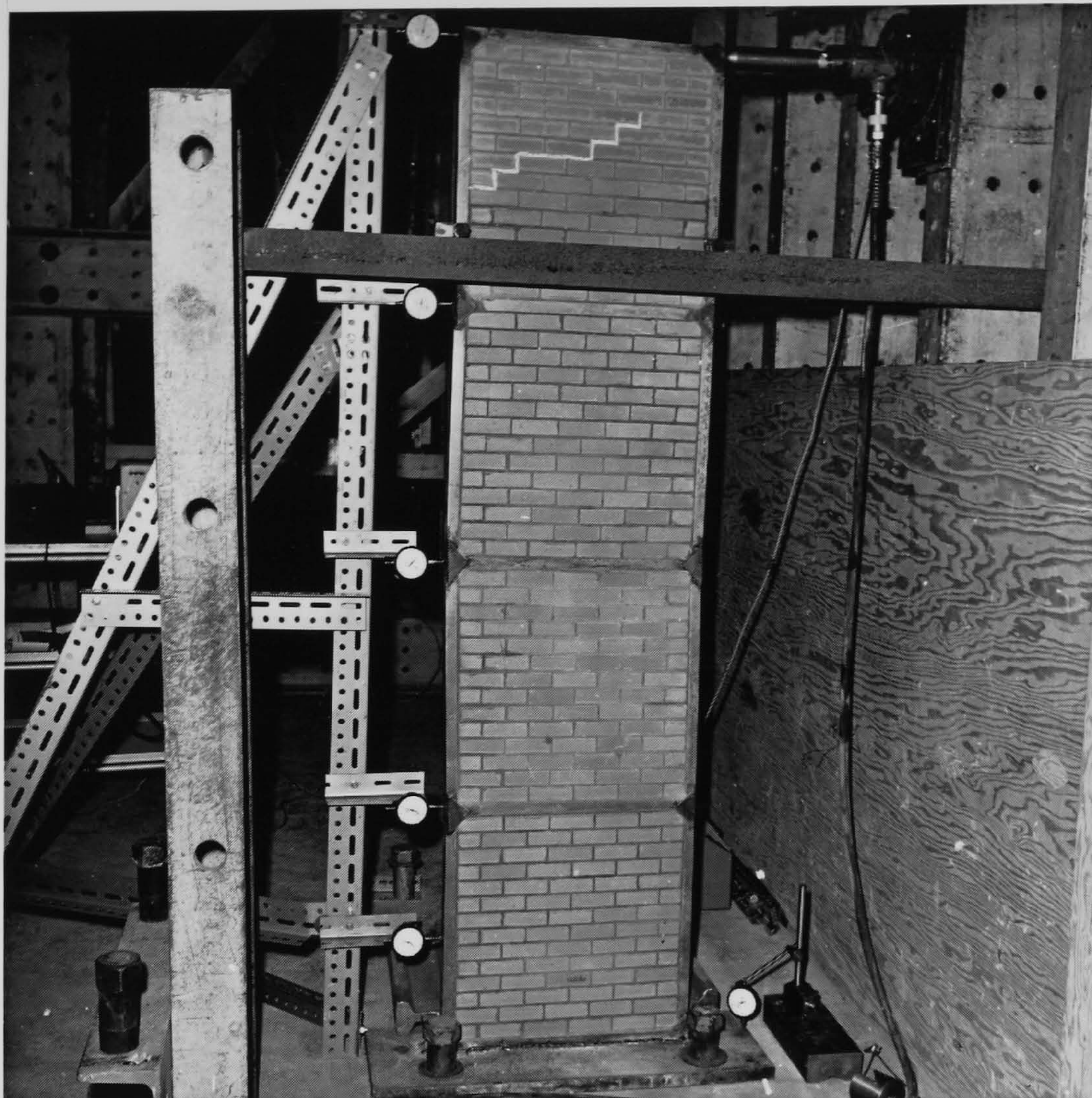
PLATE 9 TESTING ARRANGEMENT (4S)
