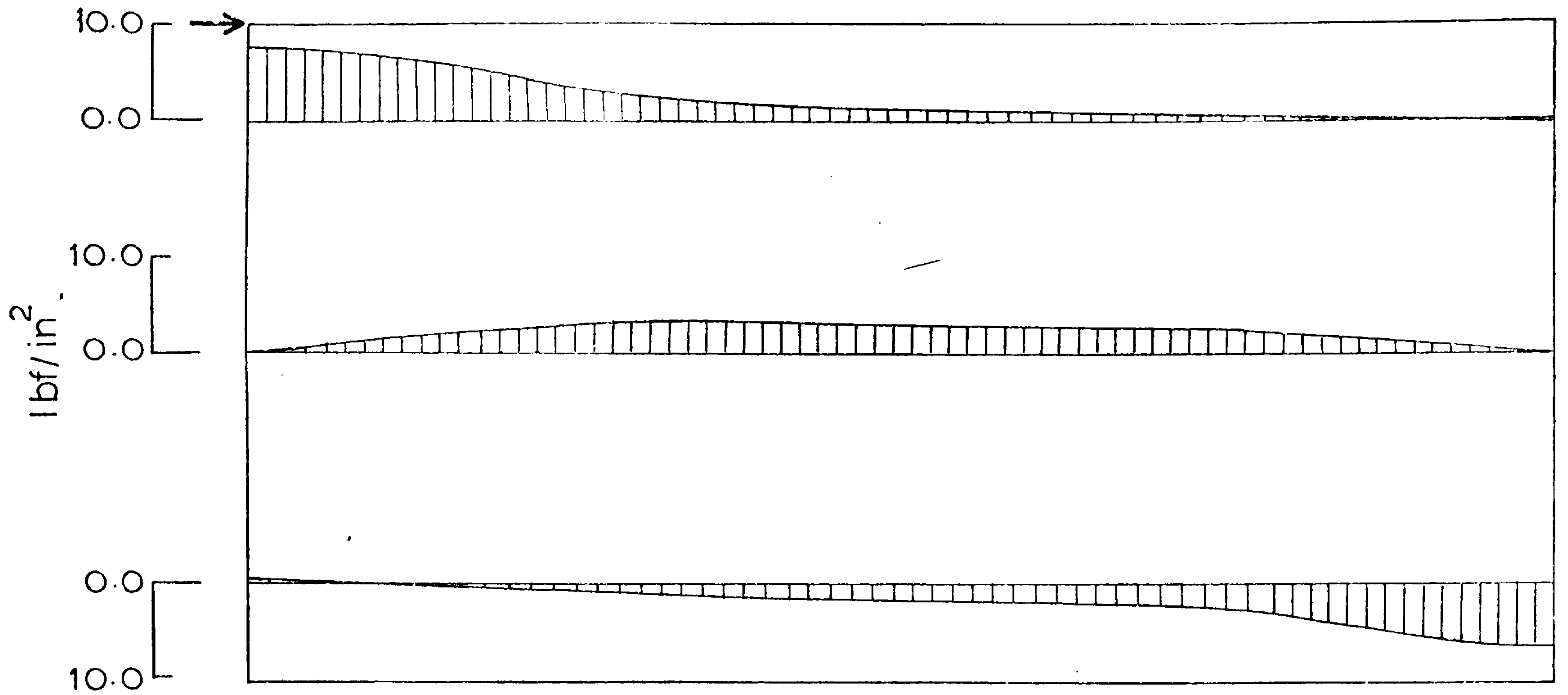
Fig.(4.20) Tangential stress distribution rect.1:2 (0.75 in)
