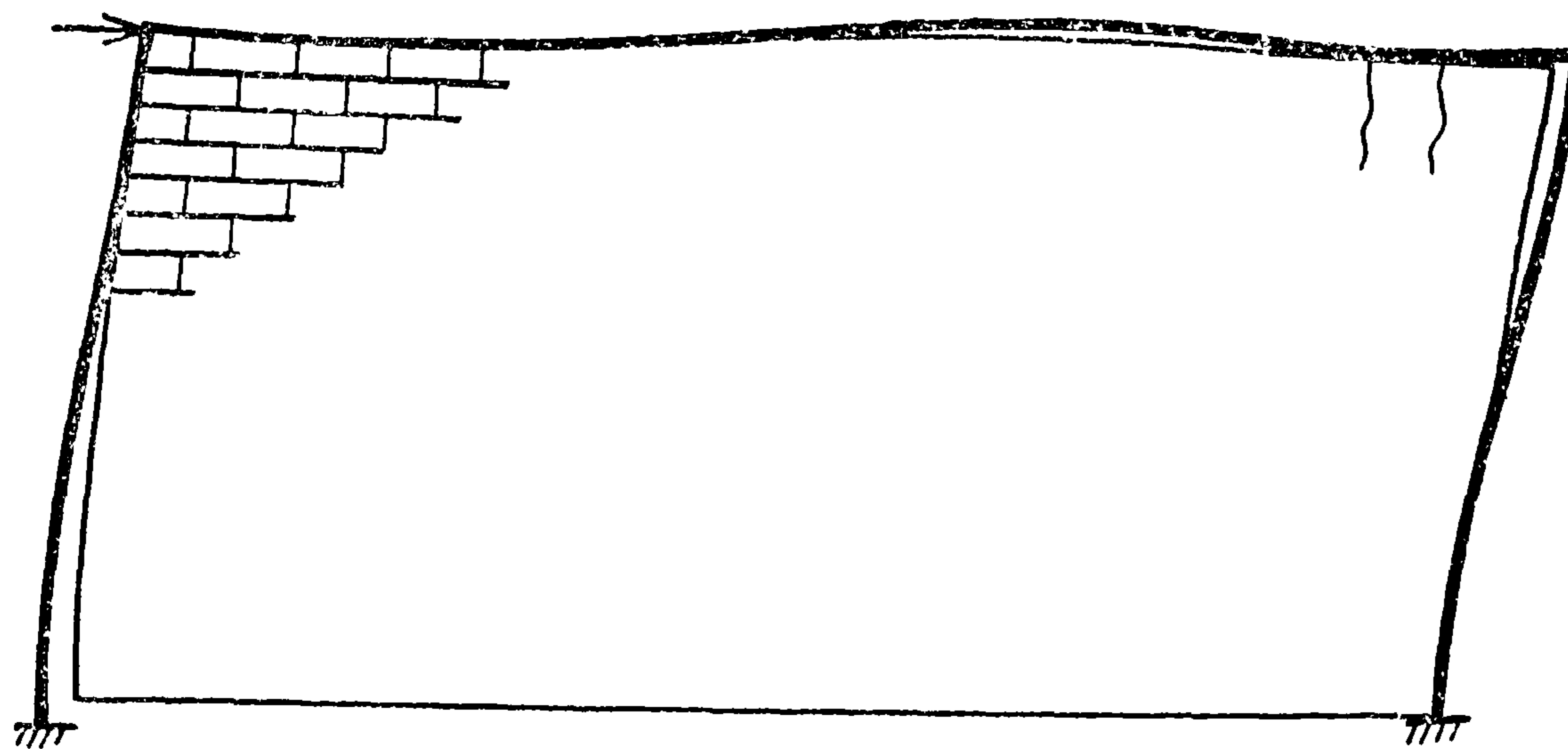
Fig.(3.17) Vertical cracks at the un-loaded corner.
