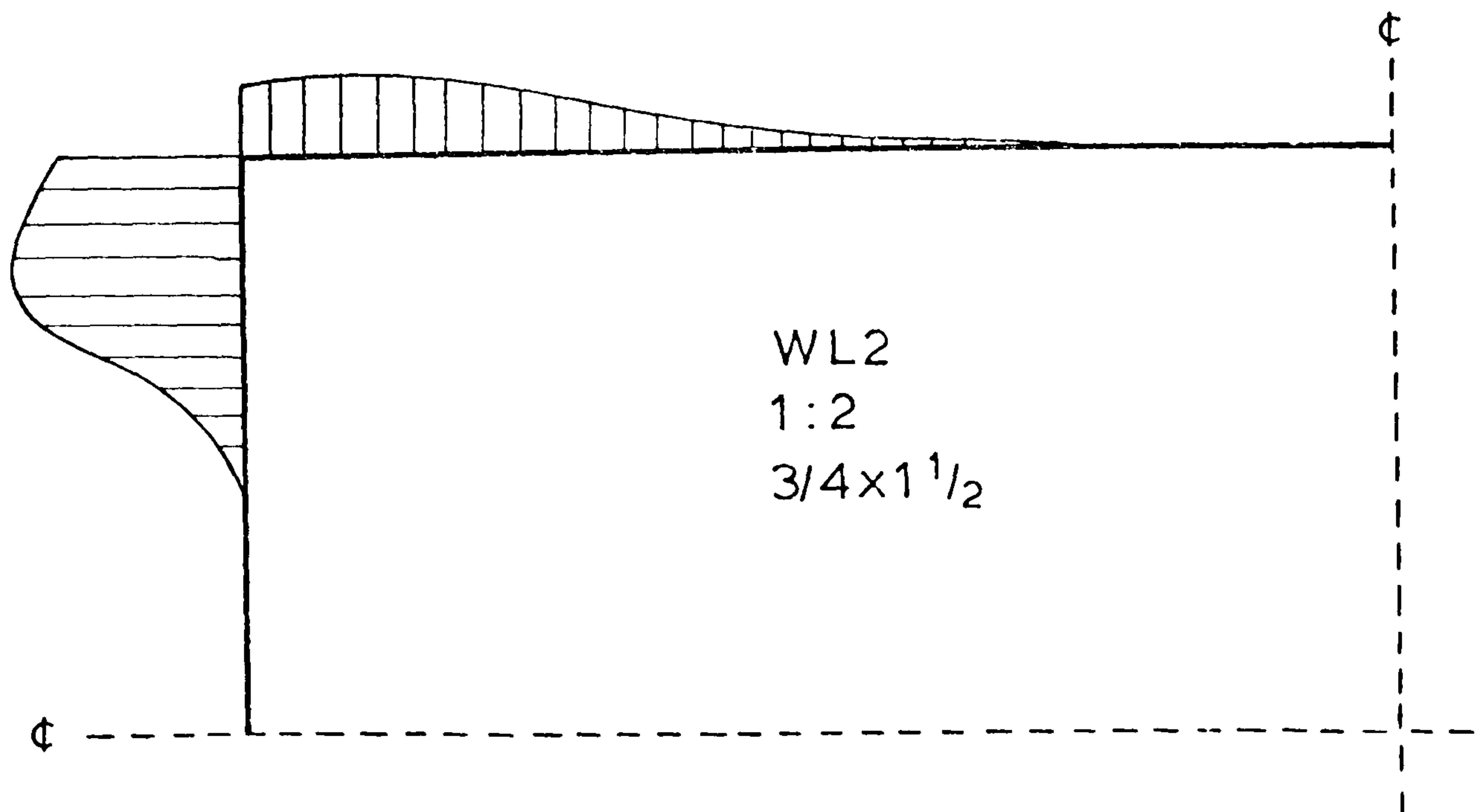
Fig.(4.16) Stress distribution at interfaces
