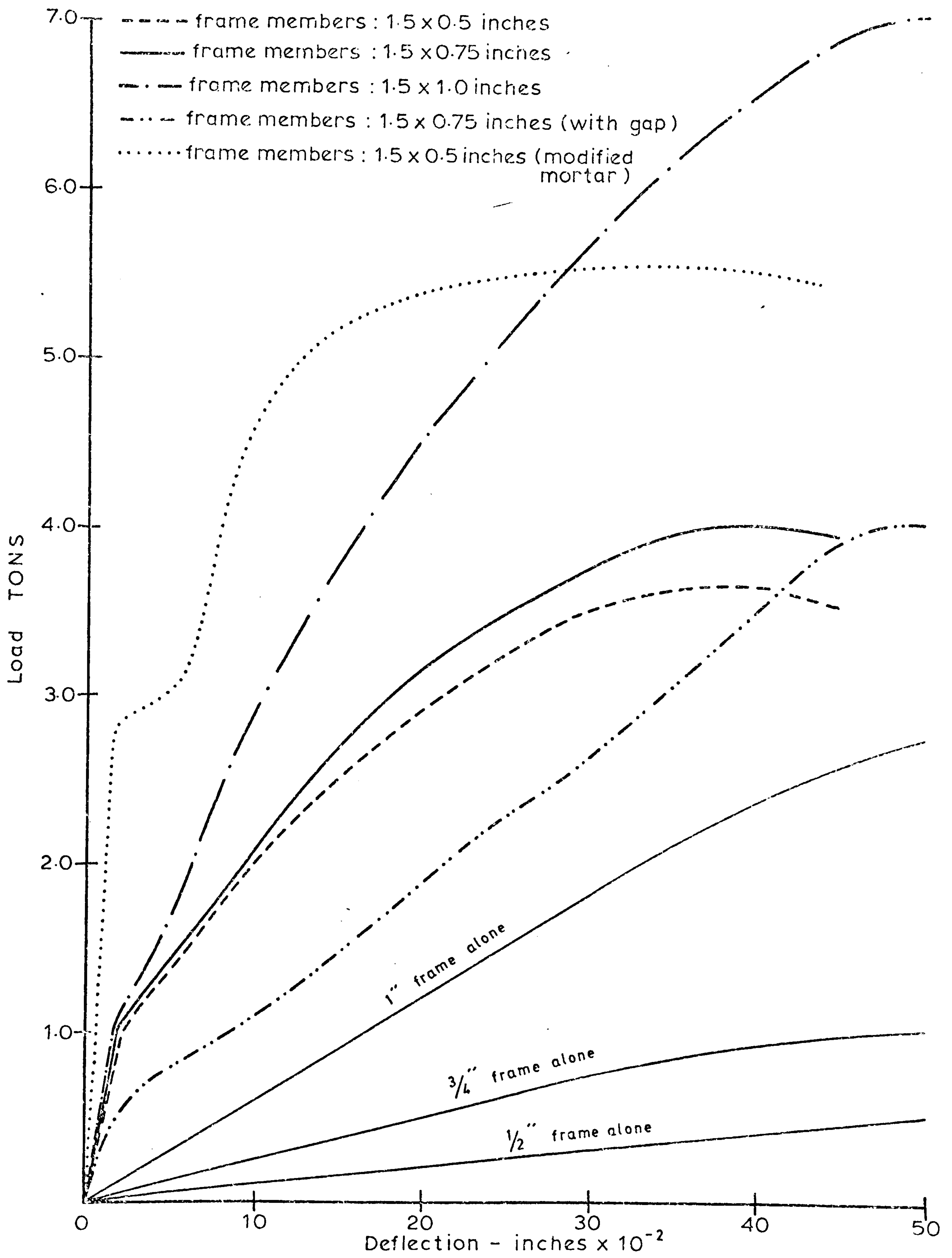
Fig.(3.3) Load-deflection curves (square panels)
