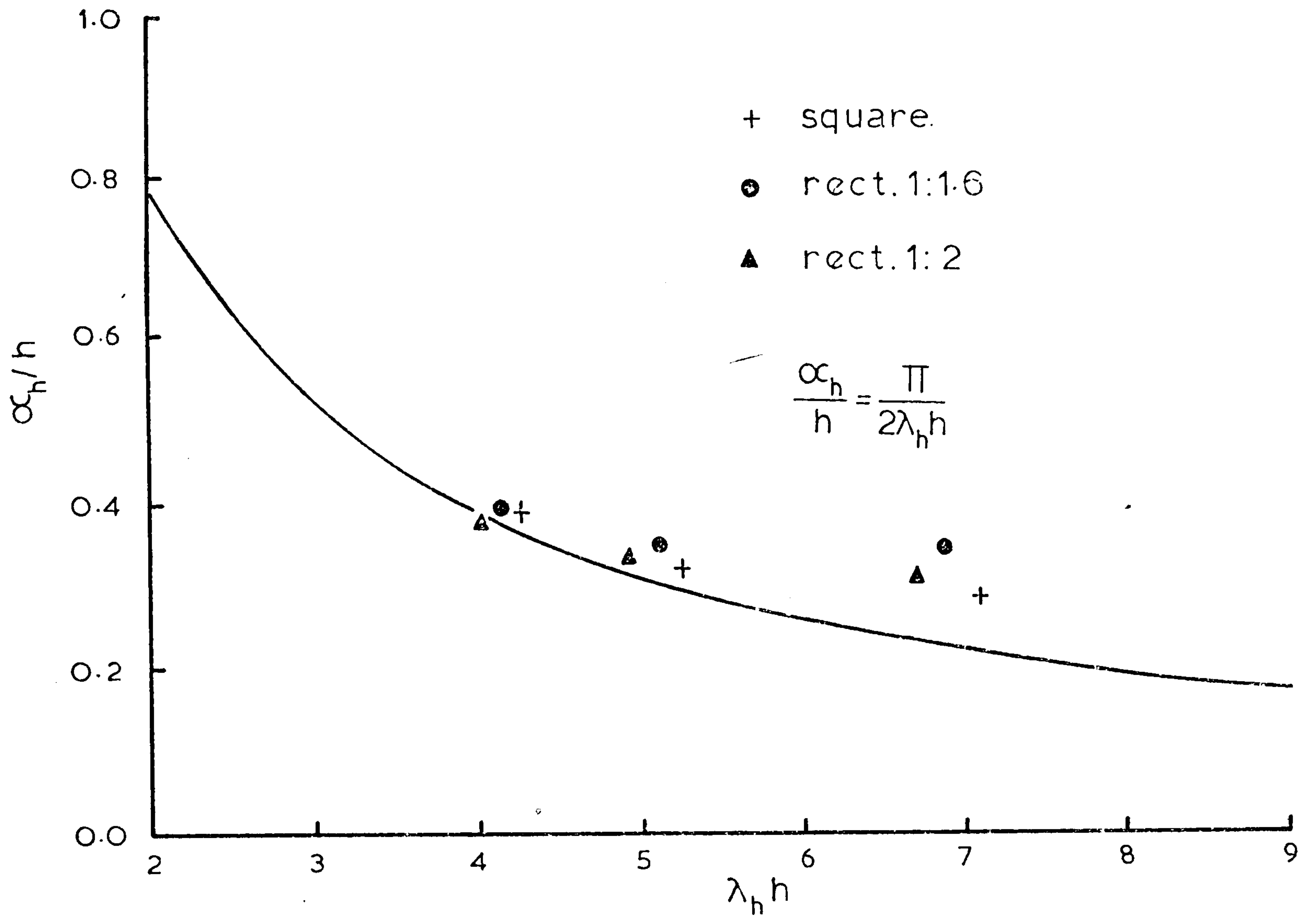
Fig.(4.3) \alpha_h as function of \lambda_h h
