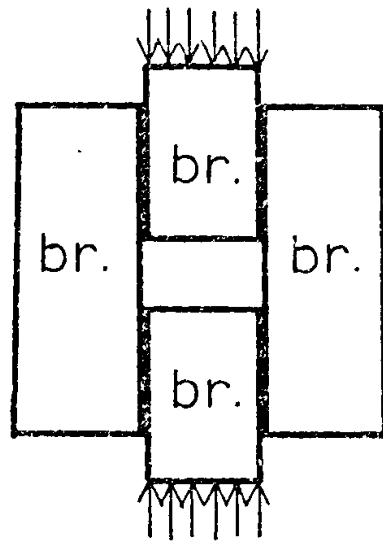
Fig.(A1) Brick triplet
