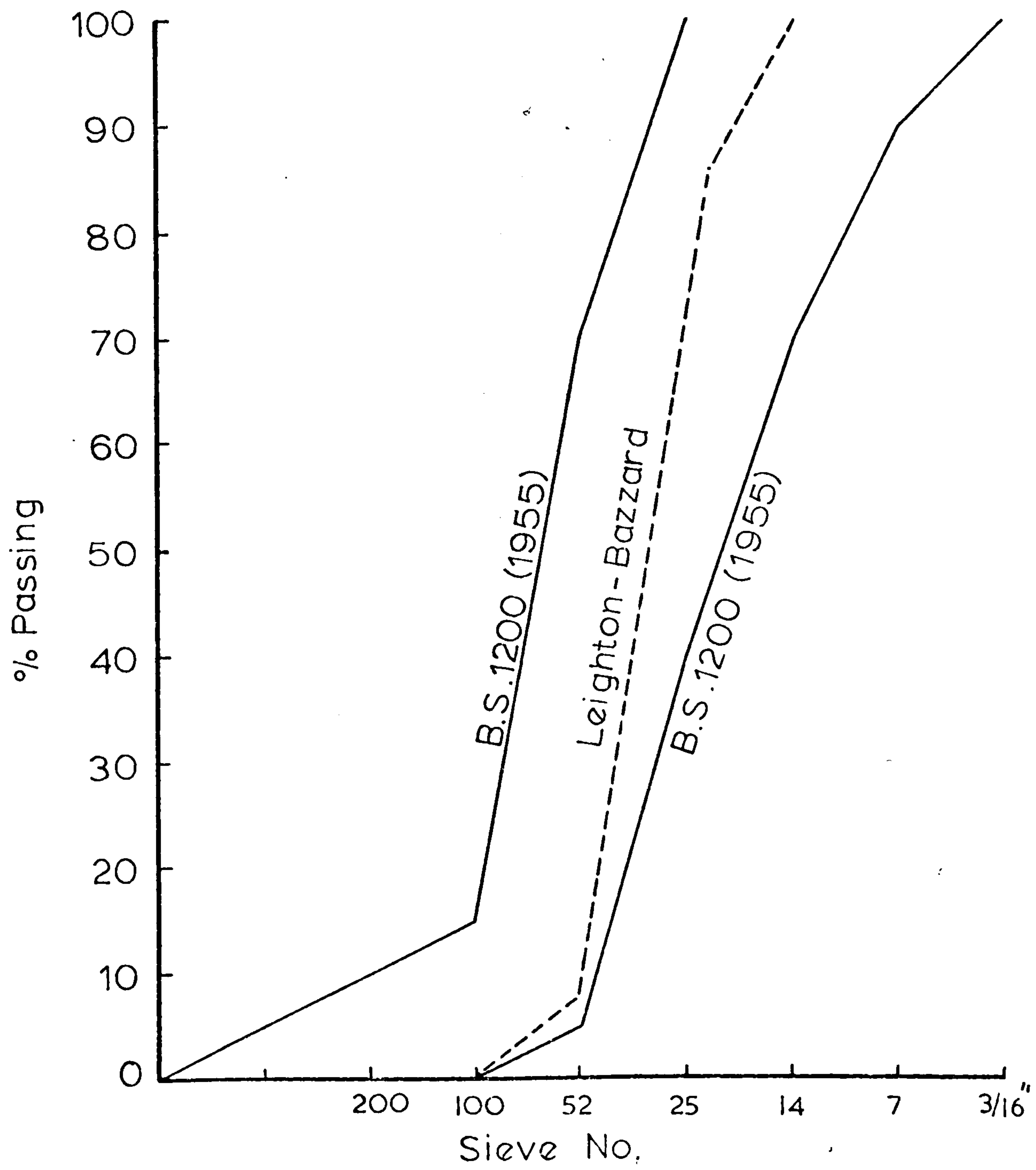
Fig.(3.1) Leighton-Bazzard sand grading curve.
