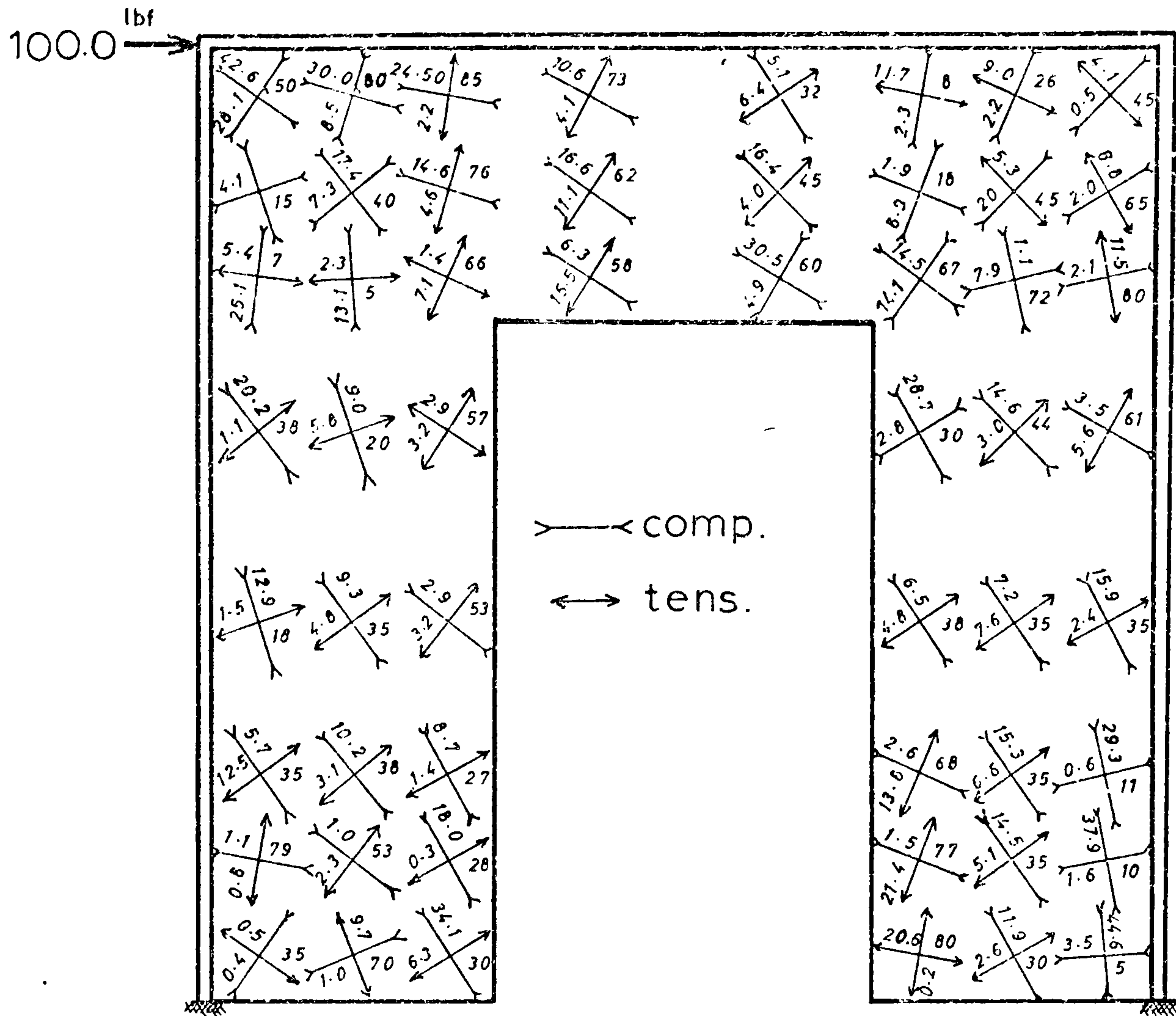
Fig.(5.5) Maximam principle stresses (WD)
