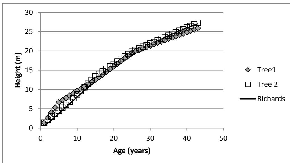
Figure 5.13: Height by age from stem analysis of Glenbranter trees.
