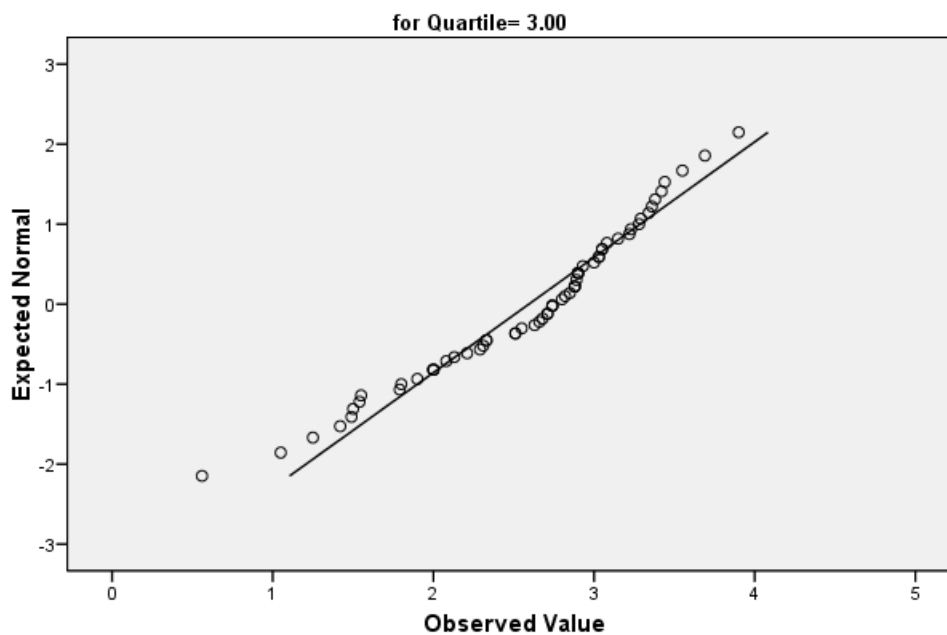
Normal Q-Q Plot of percnthgrwth
