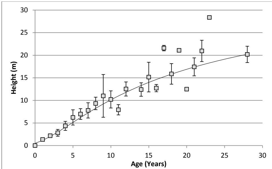
Figure 5.8: Height by age from stem analysis of Chiddingfold trees, with mean heights and error bars.
