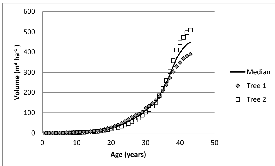
Figure 5.16: Cumulative volume ha -1 by age at Glenbranter.
