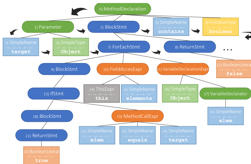
FIGURE 3. An Abstract Syntax Tree, generated from the example of Figure 2. The numbers inside each element indicate the place of the node in the visiting order. Leaves are denoted with standard rectangles (note that here the value and the type is also represented), while intermediate nodes are represented by rectangles with rounded corners.
