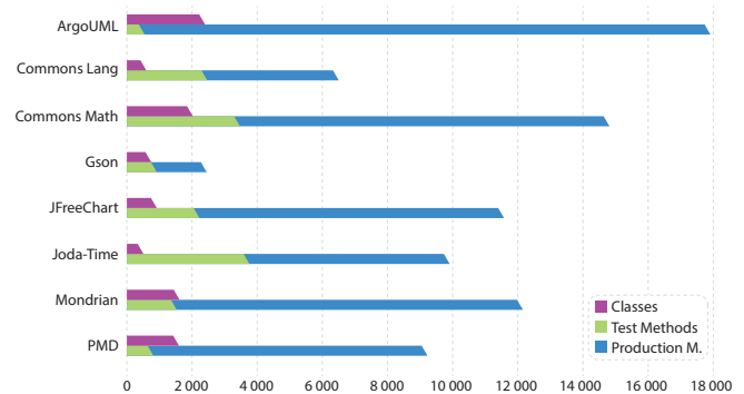
FIGURE 4. Properties of the sample projects used
