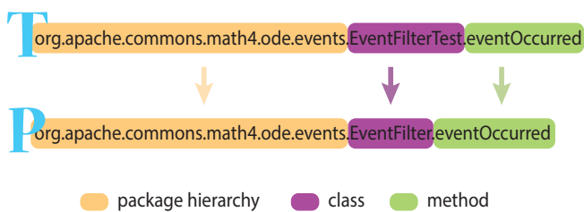
FIGURE 9. A trivial naming convention example from Commons Math
