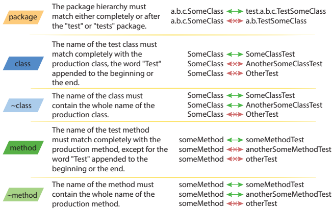
FIGURE 5. Various possible naming convention criteria components
