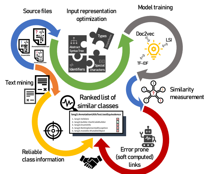
FIGURE 1. A high level overview of the proposed process
