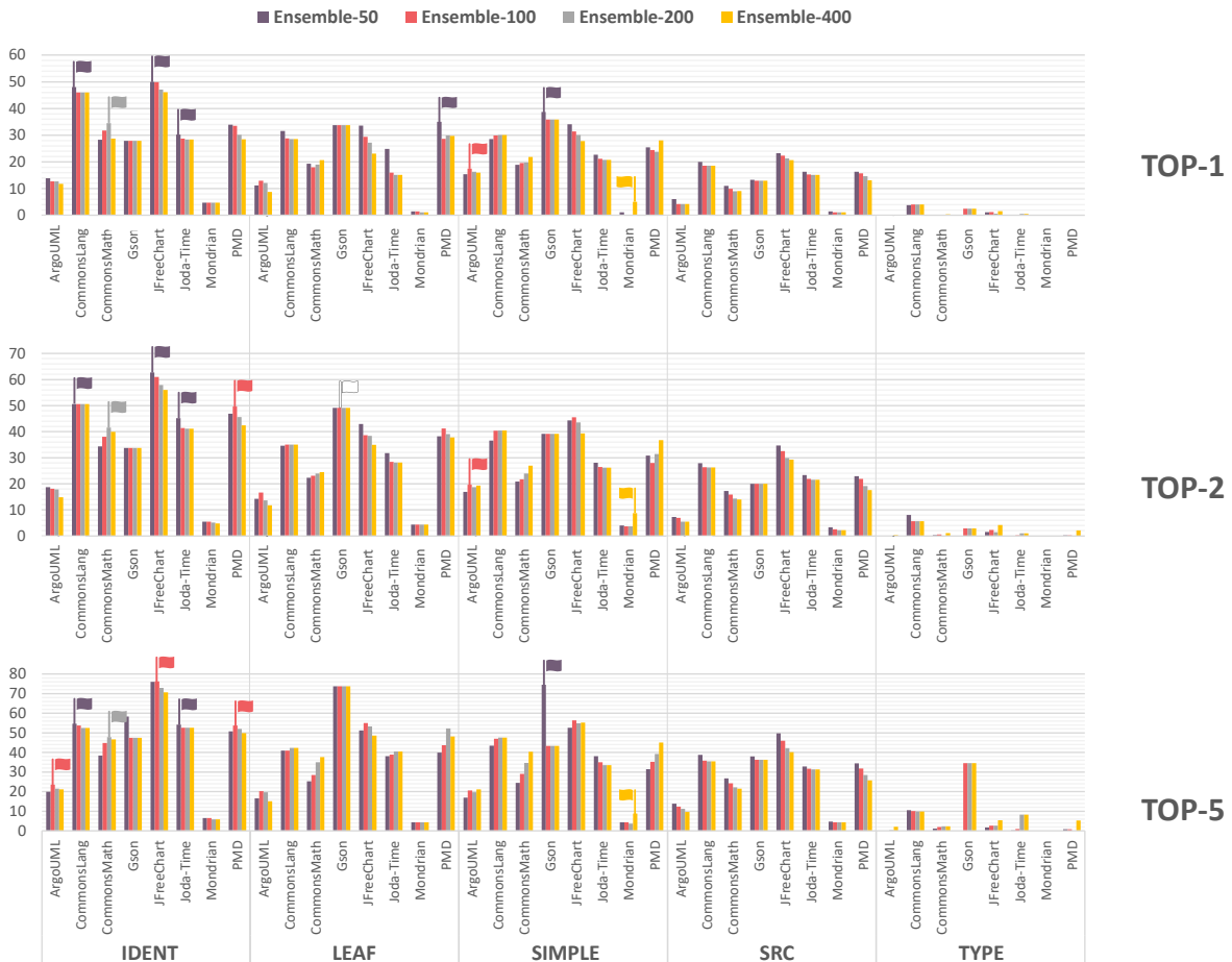
FIGURE 8. Results of the ensemble_N learning approach using NC-based evaluation.
