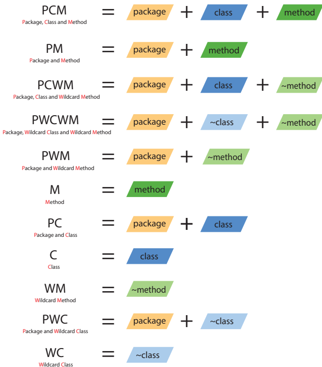
FIGURE 6. Some of the possible naming convention criteria in descending order of restrictiveness
