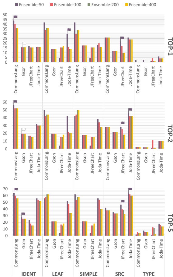
FIGURE 7. Results of the ensemble_N learning approach measured on the manual dataset.
