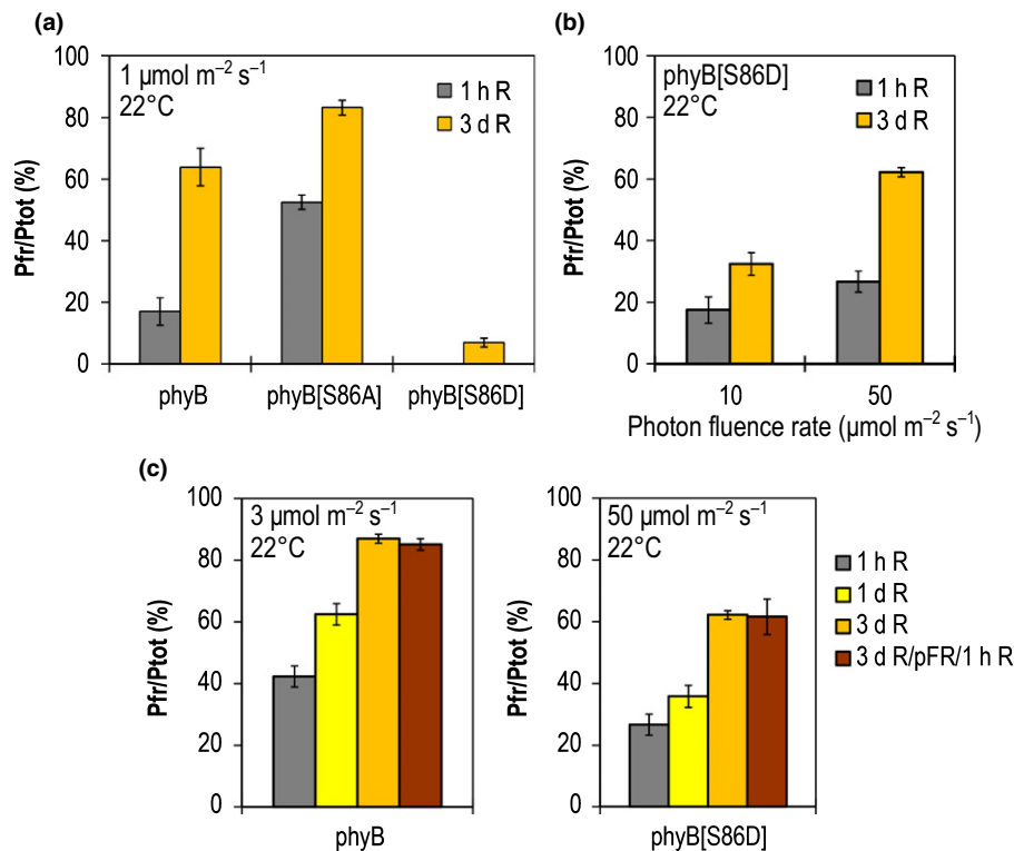
Fig. 3 The far-red light-absorbing form (Pfr) of phyB is stabilized in continuous red light in Arabidopsis thaliana . (a–c) Pfr/Ptot ratios (Ptot, total amount of phytochrome) established under prolonged irradiation with red light at 22°C were measured by in vivo spectroscopy. Seedlings were grown on norflurazon-containing plates. (a) Seedlings overexpressing phyB-green fluorescent protein (phyB-GFP), phyB[S86A]-yellow fluorescent protein (phyB[S86A]-YFP) or phyB[S86D]-YFP in the phyA-211 phyB-9 double mutant background were grown for 1 d in darkness followed by 3 d in 1 \mu\text{mol m}^{-2} \text{s}^{-1} red light (3 d R). As a control, 4-d-old etiolated seedlings were irradiated for 1 h with 1 \mu\text{mol m}^{-2} \text{s}^{-1} red light (1 h R). (b) Seedlings overexpressing phyB[S86D]-YFP were grown for 1 d in darkness followed by 3 d in 10 or 50 \mu\text{mol m}^{-2} \text{s}^{-1} red light (3 d R). As controls, 4-d-old etiolated seedlings were irradiated with 10 or 50 \mu\text{mol m}^{-2} \text{s}^{-1} red light for 1 h (1 h R). (c) Seedlings overexpressing phyB-GFP or phyB[S86D]-YFP were grown for either 3 d in darkness followed by 1 d in 3 or 50 \mu\text{mol m}^{-2} \text{s}^{-1} red light (1 d R) or for 1 d in darkness and 3 d in red light (3 d R) or were subsequently treated with a Pfr-reverting far-red light pulse (776 nm, 10 min, 50 \mu\text{mol m}^{-2} \text{s}^{-1} ) followed by 1 h red light irradiation (3 d R/pFR/1 h R). As a control, 4-d-old etiolated seedlings were irradiated with red light for 1 h (1 h R). Data are means of n \geq 3 independent measurements. Error bars indicate SEM.
