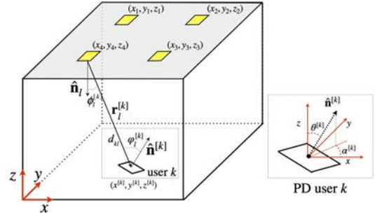
Fig. 1. Scenario and geometry of the pair transmitter-receiver.
