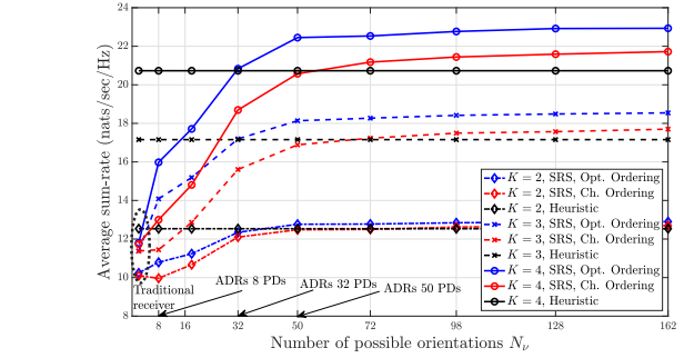
Fig. 2. Evolution of the average sum-rate versus accuracy of the vROA photodetector. P_{\text{LED}} = 40 dBm, \Psi_c = 60^\circ .
