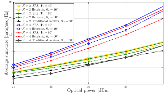
Fig. 3. Average sum-rate versus optical power per transmitter.
