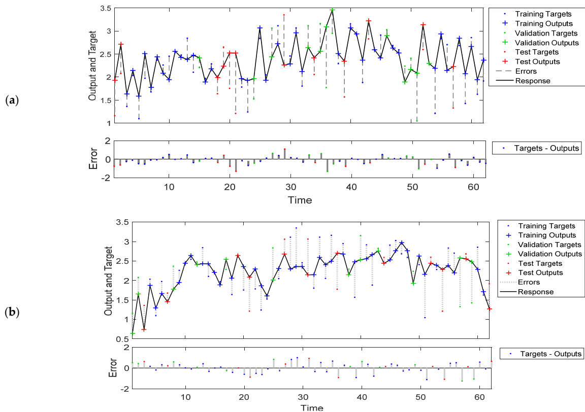
Figure 5. Response of the NARX (a) and FTD (b) neural network model output to the mosquito population time series and error. The model training was performed in an open loop (i.e., parallel series architecture), including the validation and testing step, and later on, after training, it was transformed to a closed loop for the multistep-ahead prediction.
