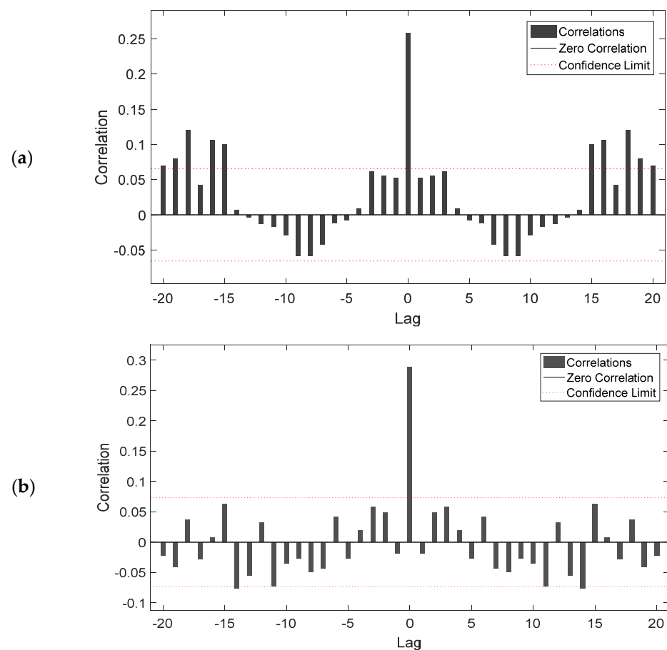
Figure 7. Autocorrelation values of the NARX (a) and the FTD (b) model in respect to different time lags and related confidence limits.
