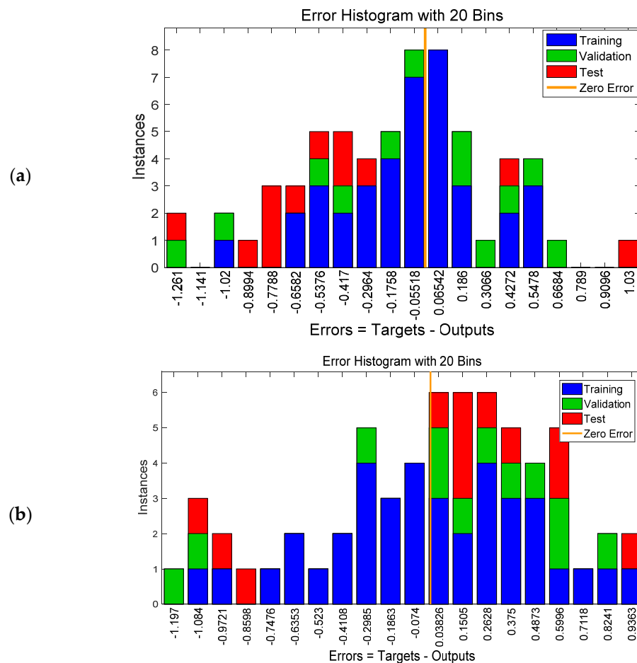
Figure 6. Error histogram chart having 20 bins for the NARX (a) and the FTD (b) neural network.
