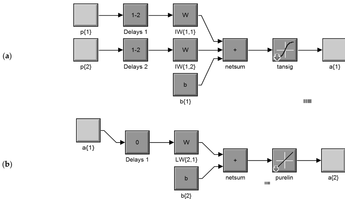
Figure 2. Abbreviated dynamic model structure, in a parallel mode, of the overall NARX network for the input layer (a) and the output layer (b), according to the Mat Lab Simulink ANN system model construction process (details in text).
