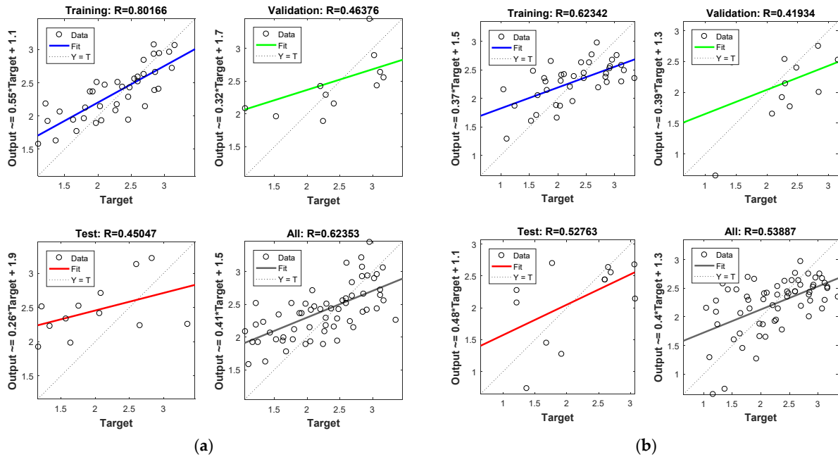
Figure 4. NARX (a) and FTD (b) neural network training, validation, and testing performance. Note that the best validation performance for the NARX model was 0.388 at epoch 3, and for the FDR model, it was 0.276 at epoch 3.
