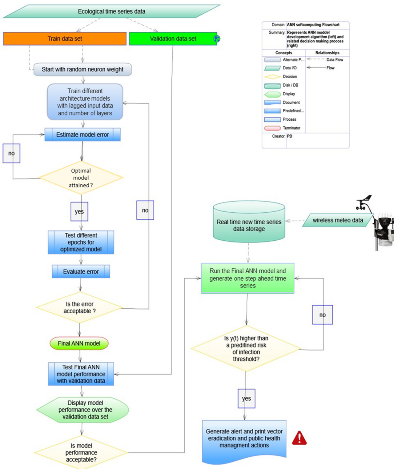
Figure 8. Graphical illustration of the logical operations followed to develop the dynamics autoregressive ANNs models for predicting adult mosquito population dynamics (left). Real-time data can be used later to forecast the arthropod vector population dynamics based on the calibrated ANN model that has been developed or to be retrained under new circumstances (right).
