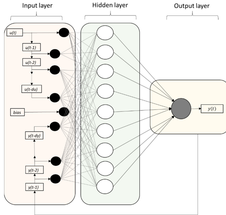
Figure 1. Graphical illustration of the NARX network with du input and dy output memory and a number of neurons in the hidden layer. Note that if the output memory is set at dy = 0 , then the NARX network is reduced to a plain FTD neural network architecture.
