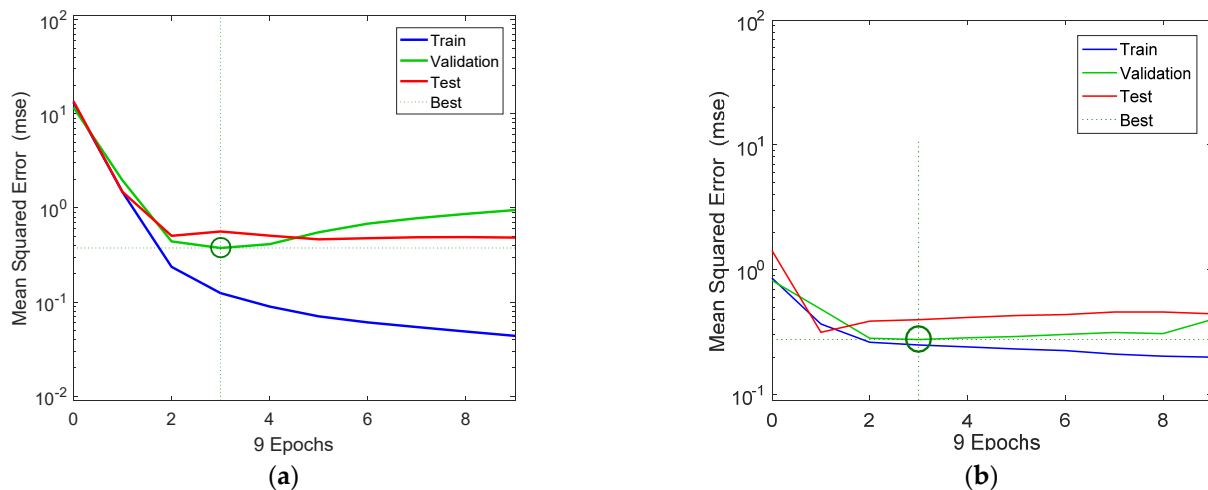
Figure 3. NARX (a) and FTD (b) neural network training, validation, and testing performance. Note that the best validation performance for the NARX model was 0.388 at epoch 3, and for the FDR model, it was 0.276 at epoch 3.
