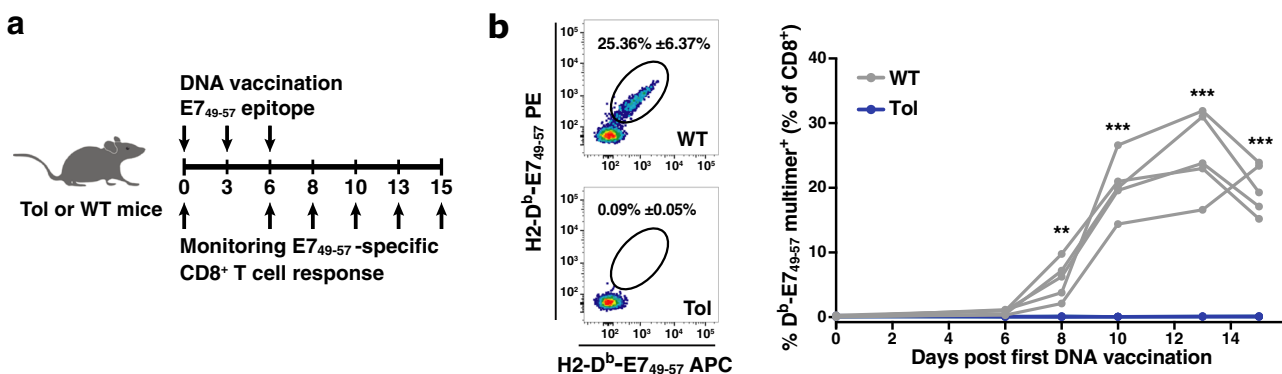
Fig. 2 Complete loss of E7 49-57 immunogenicity in Tol mice. a Schematic overview of vaccination and monitoring strategy. b Left: Representative flow cytometry plots depicting E7 49-57 -specific CD8 + T cells at day 13 post DNA vaccination in WT and Tol mice. Right: E7 49-57 -specific CD8 + T-cell response in blood of WT (gray) and Tol (blue) mice at the indicated timepoints post first DNA vaccination. Lines indicate individual mice. Cells are gated on IR-dye - CD8 + lymphocytes. Depicted data are representative of two independent experiments, including at least 5 mice per group. P values were determined by Repeated Measures two-way ANOVA with Sidak's multiple comparisons test to test the significance at each timepoint. * p < 0.05; ** p < 0.01; *** p < 0.001.
