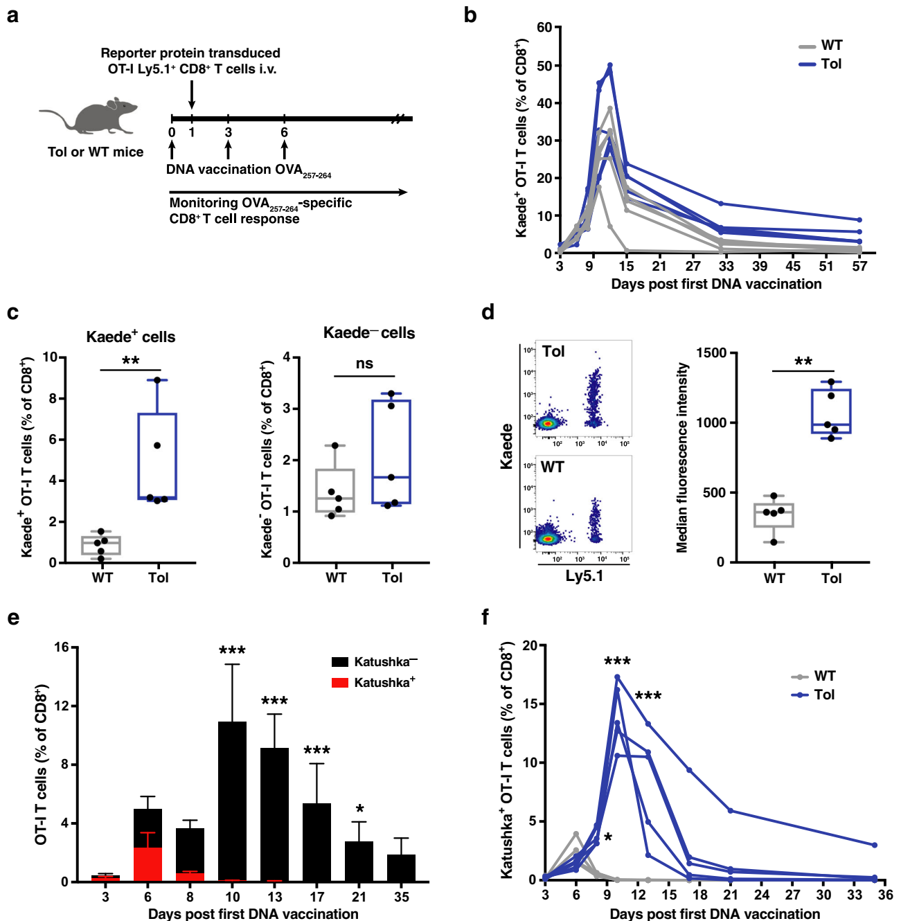
Fig. 3 Enhanced engraftment of Kaede - and Katushka-expressing cells in Tol mice. a Schematic overview of experimental design. b Percentage of Kaede + OT-I T cells in the blood of WT (gray) and Tol (blue) mice at the indicated timepoints post first DNA vaccination. c Percentage of Kaede + (left) or Kaede - (right) OT-I cells in WT and Tol mice at day 57 after first DNA vaccination. d Left: representative flow cytometry plots depicting Kaede expression in transferred (Ly5.1 + ) cells at day 57 after first DNA vaccination. Right: median fluorescence intensity (MFI) of Kaede + OT-I cells in WT and Tol mice at day 57 post first DNA vaccination. e Percentage of Katushka + (red) and Katushka - (black) OT-I cells in WT animals at the indicated timepoints after first DNA vaccination. f Percentage Katushka + OT-I cells in WT and Tol mice at the indicated timepoints after first DNA vaccination. Cells ( b–f ) are gated on IR-dye - CD8 + lymphocytes, and plots depict n = 5 (Tol) and n = 5 (WT) mice. Depicted data are representative of one ( b–d ) or two ( e, f ) independent experiments. Box-plots ( c, d ) depict interquartile range, with whiskers representing minimum and maximum values. Dots ( c, d ) and lines ( b, f ) indicate individual mice. Error bars ( e ) represent SD. P values were determined by either two-tailed Mann-Whitney signed rank test ( c, d ) or Repeated Measures two-way ANOVA with Sidak's multiple comparisons test ( e, f ). * p < 0.05 ; ** p < 0.01 ; *** p < 0.001 , ns not significant.
