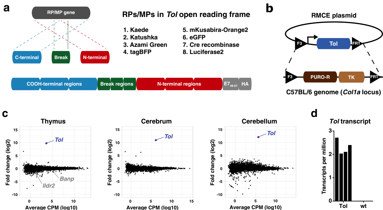
Fig. 1 Generation and validation of the Tol mouse model. a Top left: cartoon depicting the strategy for reporter gene fragmentation, applied for each RP/MP gene included in the Tol ORF. Top right: reporter proteins included in the Tol ORF. Bottom: schematic overview of gene fragment placement in the Tol ORF. Note that the Tol ORF encodes the HPV E7 49-57 epitope in the COOH-terminal region of the chimeric Tol protein. b Cartoon depicting the targeting strategy of the Tol ORF into the Col1a1 locus through recombinase-mediated cassette exchange. c Differential gene expression analysis of indicated organs of Tol mice relative to WT mice. Scatterplots indicate average log 2 fold changes and average counts per million. Genes with a statistically significant change in expression in Tol mice are indicated in gray, and the Tol transcript is indicated in blue. d Expression levels of the Tol transcript in thymi of Tol and WT mice. Data shown ( c , d ) is aggregated from n = 4 (Tol) and n = 4 (WT) mice. RP reporter protein, MP modifier protein, RMCE recombinase-mediated cassette exchange, PURO-R puromycin resistance gene, TK thymidine kinase gene, CPM counts per million.
