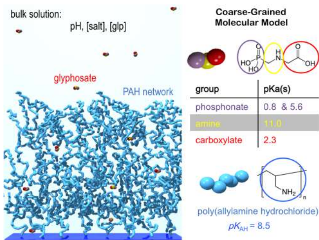
Figure 1. Left: Scheme representing the adsorption of GLP from a salt solution to a surface-grafted, cross-linked PAH network. The coarse-grained molecular model is illustrated on the right. AMPA is modeled similarly to GLP but without including the carboxylate unit.
