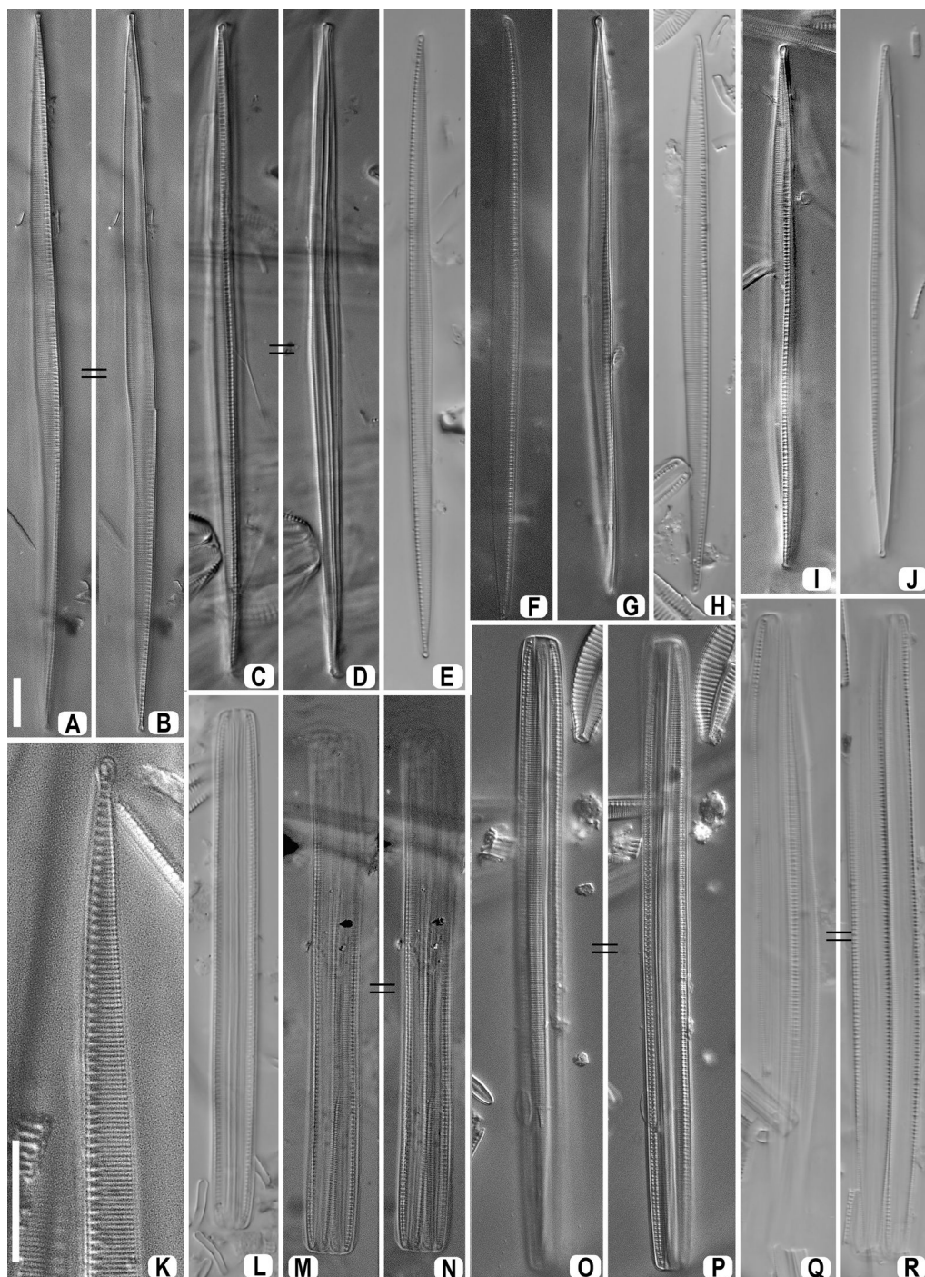
Fig. 4. Nitzschia araucana , sp. nov. LM. Specimens of type population. A-B. Holotypus. A-K. Valve views. K. Higher magnification image of the valve apex; fibular and slightly punctate striae are evident. L-R. Girdle views showing different frustular symmetries. M-N. Two frustules at different levels of focus, one exhibiting hantzschoid symmetry and one with nitzschoid symmetry. O-P. Frustule at different focal planes, showing hantzschoid symmetry. Q-R. Two frustules at different levels of focus, one exhibiting hantzschoid symmetry and one with nitzschoid symmetry. Scale bars = 10 \mu\text{m} (A-J, L-R); 5 \mu\text{m} (K).
