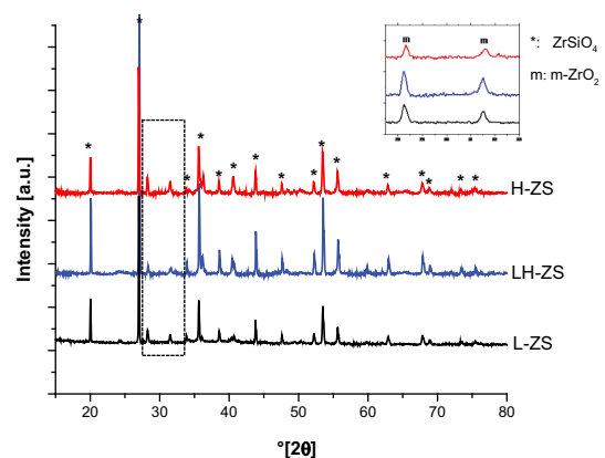
Figure 3. XRD plots of solid sintered dog-bone samples Inset: m- ZrO_2 peaks.
