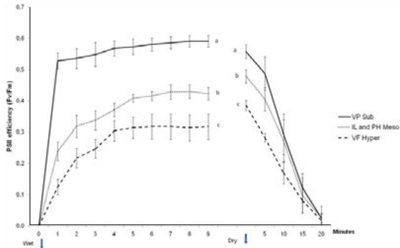
Fig. 4. Recovery of photosynthetic activity ( F_v/F_m ) after hydration of dry freshwater lichen thalli by liquid water and then cessation of activity of fully hydrated fragments during desiccation in-air (at T = 20^\circ\text{C} and RH = 50\% ). Values are means \pm SE; n = 10 , the different letters correspond to statistically different groups ( P < 0.001 ). Lichen species and sampling, see legend of Figure 1. RH, relative humidity.
