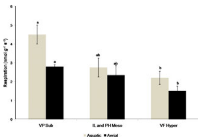
Fig. 1. Dry mass-related dark respiration of wet thalli of freshwater lichens. Respiration of immersed thalli ( \text{O}_2 uptake) or aerial fully hydrated thalli ( \text{CO}_2 evolution) was measured on selected species. Experiments were performed a few days after collection of dry lichens from sun-exposed watercourses. Values are means ± SE; n = 30 , the different letters correspond to statistically different groups ( P < 0.001 ). Statistical analyses were performed separately for immersed or aerial thalli. VP sub, Verrucaria praetermissa subhydrophilic; IL and PH meso, Ionaspis lacustris and Porpidia hydrophila mesohydrophilic; VF hyper, Verrucaria funckii hyperhydrophilic.
