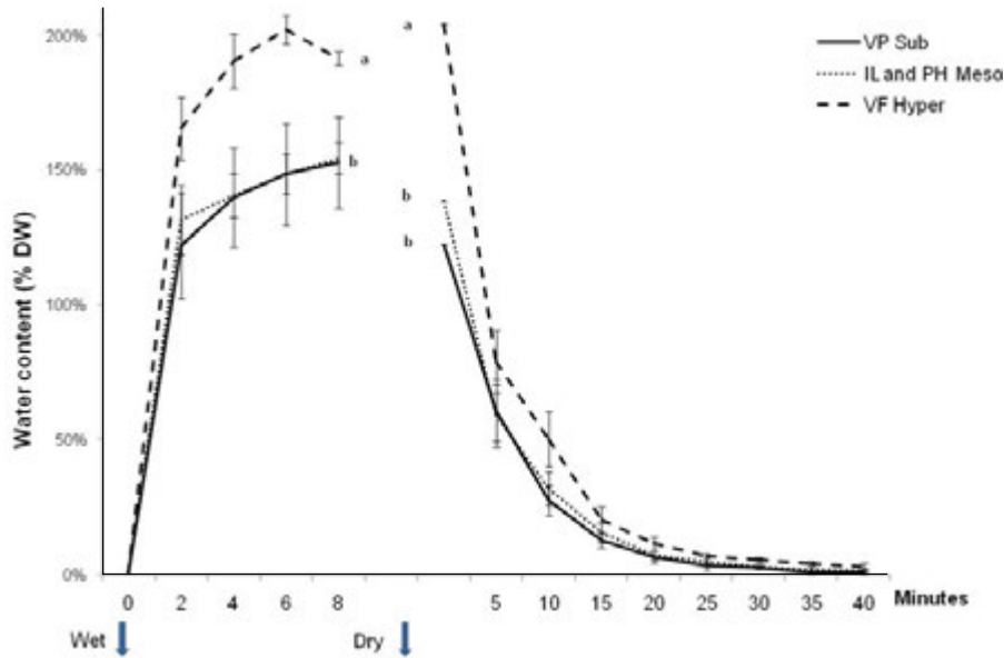
Fig. 3. Changes in lichen freshwater water content versus time after immersion in liquid water of dry thalli and then after placing the hydrated thalli in-air (at T = 20^\circ\text{C} and RH = 50\% ). Values are means \pm SE; n = 10 , the different letters correspond to statistically different groups ( P < 0.001 ). Lichen species and sampling, see legend of Figure 1. RH, relative humidity.
