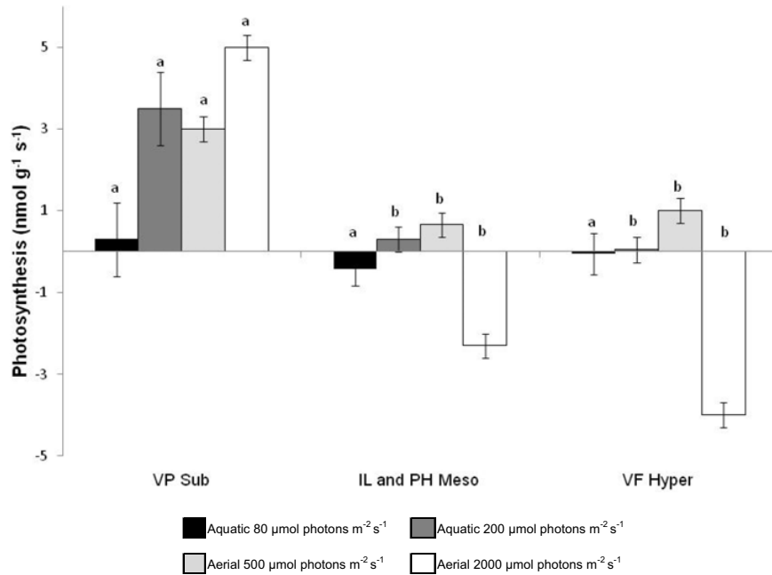
Fig. 2. Dry mass-related net photosynthesis of wet thalli of freshwater lichens. Photosynthesis of immersed thalli ( O_2 evolution) or aerial fully hydrated thalli ( CO_2 uptake) were measured on selected species. Light irradiance at thallus level was 80 \mu\text{mol}\cdot\text{m}^{-2}\cdot\text{s}^{-1} PAR (photosynthetically active radiation) or 200 \mu\text{mol}\cdot\text{m}^{-2}\cdot\text{s}^{-1} PAR for underwater measurements and 500 \mu\text{mol}\cdot\text{m}^{-2}\cdot\text{s}^{-1} PAR or 2000 \mu\text{mol}\cdot\text{m}^{-2}\cdot\text{s}^{-1} PAR for aerial measurements. Values are means \pm SE; n = 30 , the different letters correspond to statistically different groups ( P < 0.001 ). Statistical analyses were performed separately for immersed or aerial thalli. Lichen species and sampling, see legend of Figure 1.
